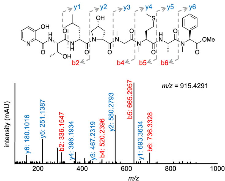
Fig. 2. ESI-TOF MS/MS Analysis of seco -Viridogrisein B Methyl ester
