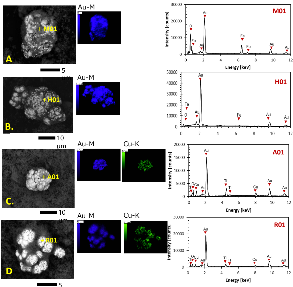
Figure 4.3. SEM photomicrographs of gold cemented in different semiconductive material in single system A) magnetite B) hematite C) anatase and D) rutile.
