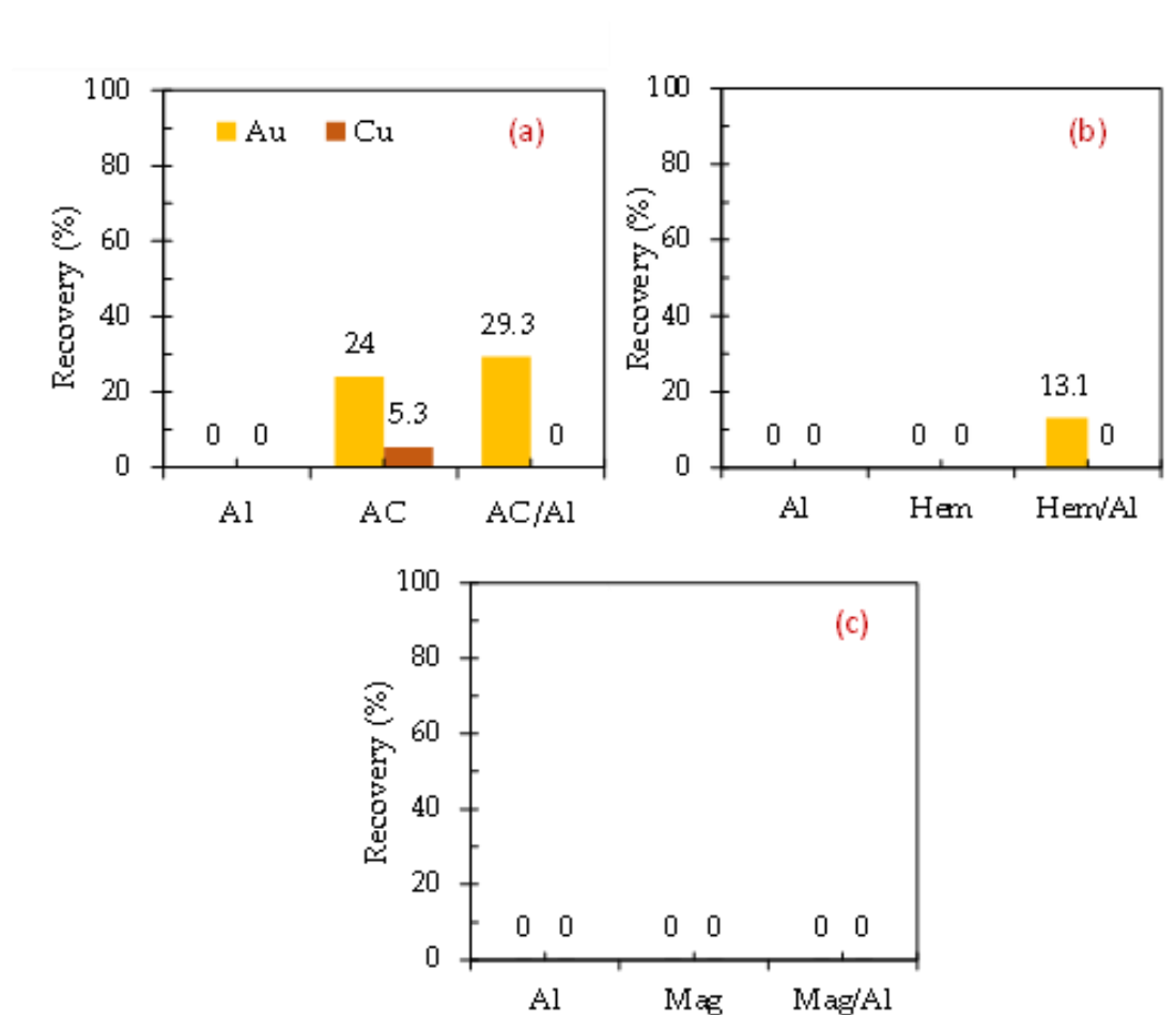
Figure 2.1 Percent (%) recovery of gold, Au and copper, Cu from different galvanic constituents in air atmosphere after 24hrs a) activated carbon (AC) and or /ZVAl b) hematite (Hem) and or/ ZVAl and c.) magnetite (Mag) and or /ZVAl.
