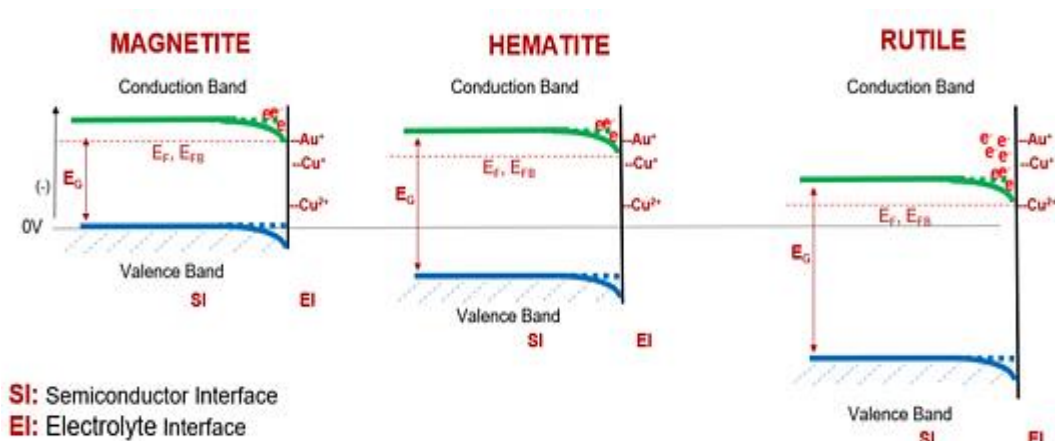
Figure 5.4 Schematic Energy band diagrams for the semiconductor-electrolyte interface (SEI) for a) Rutile b) Hematite and c) Magnetite.
