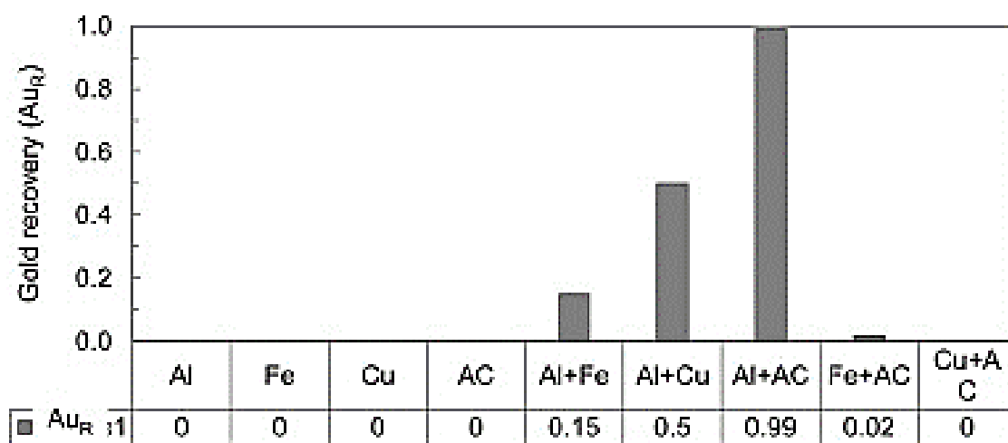
Figure 1.13 Recovery of Au ions from ammonium thiosulfate solution by various materials and their mixtures (Al, Fe, Cu, AC, Al-Fe, Al-Cu, Al-AC, Fe-AC, and Cu-AC) (Note that AC denotes activated carbon) Jeon et. al, 2022.
