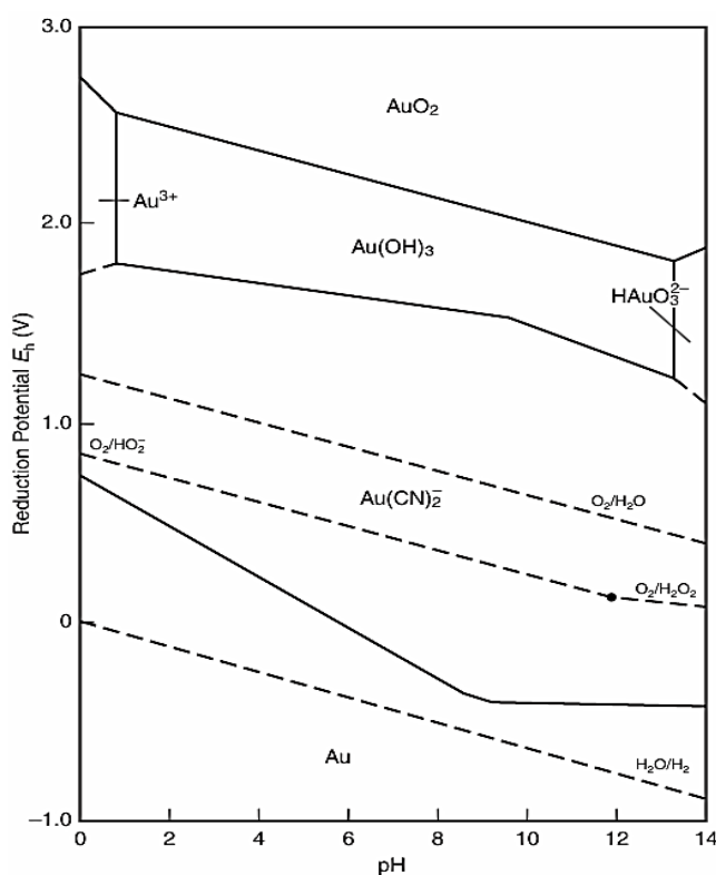
Figure 1.3 Potential-pH equilibrium diagram for the system Au-H 2 O-CN - at 25°C. Concentrations of all gold species = 10^{-4} M [6]. [\text{CN}^-]_{\text{total}} = 10^{-3} M, p\text{O}_2 = p\text{H}_2 = 1 atm, \log ([\text{H}_2\text{O}_2] - [\text{HO}_2^-]/p\text{O}_2) . (From the Textbook Chemistry of Gold Extraction, J.O Marsden).
