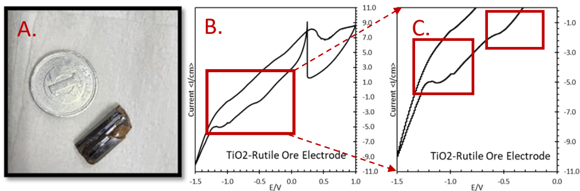
Figure 4.10 Electrochemical profile using rutile crystal A) rutile crystal specimen B) Cyclic voltammogram C) Narrow reductive scan.
