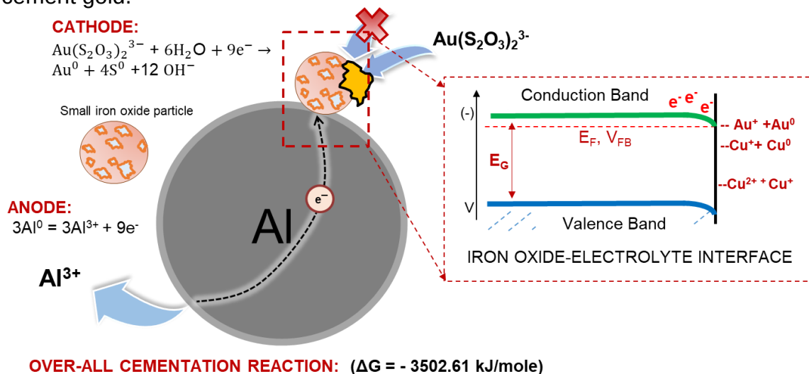
Figure 4.21 Schematic diagram of iron oxide's selective cementation mechanism to gold as an electron mediator upon galvanic interaction with zero-valent aluminum.
