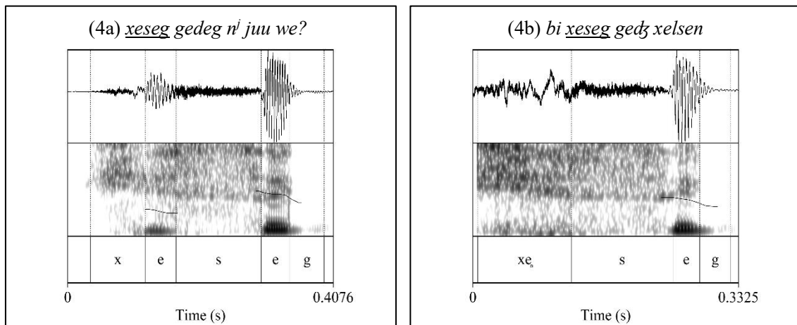
Figure 4. Wave forms, spectrograms, and pitch curves of xesege pronounced by an informant (left: in (4a), right: in (4b))
