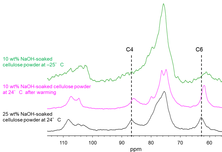
Fig. 2-12. In situ solid-state ^{13}\text{C} CP/MAS NMR spectra. Color code: green line, 10 wt% NaOH-soaked cellulose powder (the spectrum was recorded at -25^\circ\text{C} after cooling the sample from 24^\circ\text{C} to -25^\circ\text{C} ); pink line, 10 wt% NaOH-soaked cellulose powder (the spectrum was recorded at 24^\circ\text{C} after cooling the sample from 24^\circ\text{C} to -25^\circ\text{C} , followed by warming to 24^\circ\text{C} ); and black line, 25 wt% NaOH-soaked cellulose powder at 24^\circ\text{C} .
