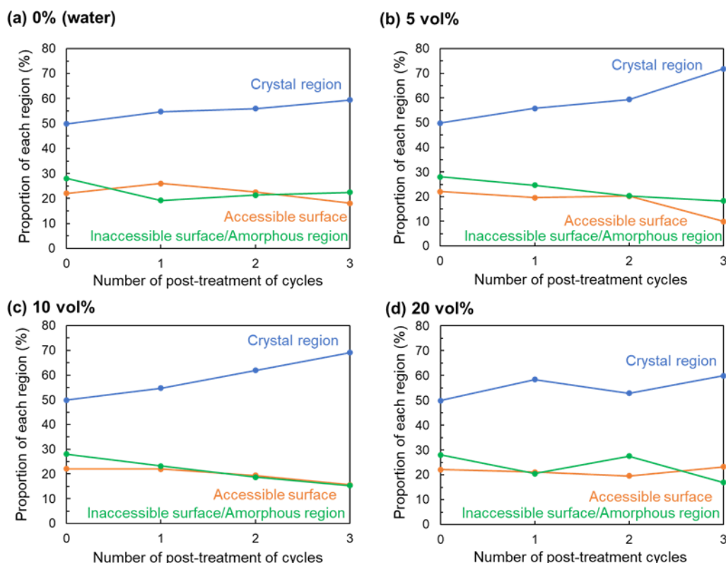
Fig. 3-9. Proportions of crystalline regions (blue line), accessible surfaces (orange line), and inaccessible surfaces/amorphous regions (green line) evaluated from the ^{13}\text{C} CP/MAS NMR spectra of samples obtained after multicycle post-treatment with neutralization using (a) 0% (water), (b) 5 vol%, (c) 10 vol%, and (d) 20 vol% \text{H}_2\text{SO}_4 solutions.
