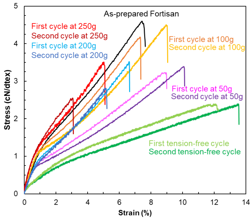
Fig. 3-17. The stress-strain (S-S) curves of the as-prepared fortisan and the fortisan samples that underwent the multicycle post-treatments; black line, the as-prepared fortisan; redline, first cycle tensioned at 250 g on single strain; deep red line, second cycle tensioned at 250 g on single strain; light blue line, first cycle tensioned at 200 g on single strain; blue line, second cycle tensioned at 200 g on single strain; orange line, first cycle tensioned at 100 g on single strain; yellow line, second cycle tensioned at 100 g on a single strain, pink line, first cycle tensioned at 50 g on single strain; purple line, second cycle tensioned at 50 g on single strain; light green line, first tension-free cycle; green line, second tension-free cycle.
