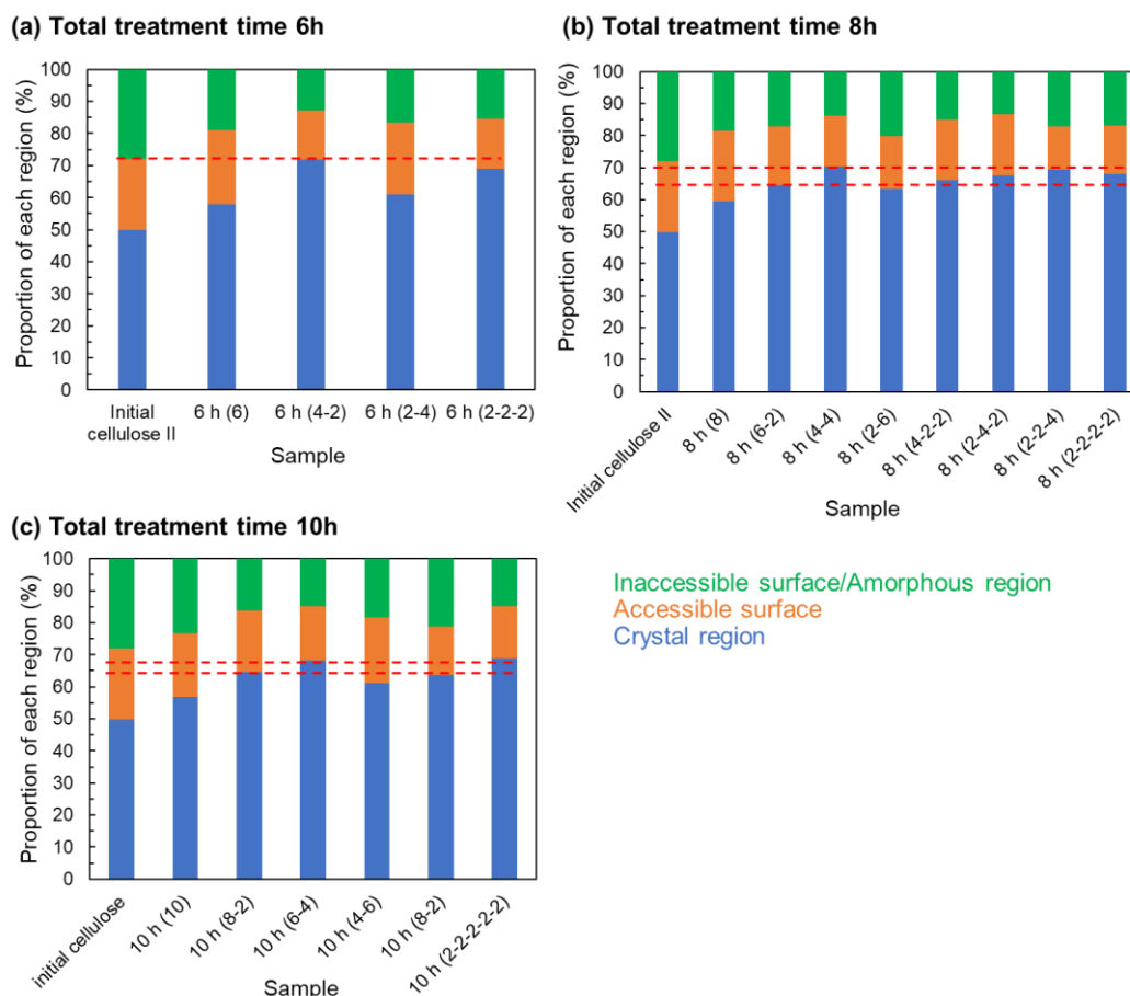
Fig. 3-12. Proportions of crystalline regions (blue bars), accessible surfaces (orange bars), and inaccessible surfaces/amorphous regions (green bars) as evaluated from the solid-state ^{13}\text{C} CP/MAS NMR spectra of samples obtained via multicycle post-treatment with a total post-treatment time of (a) 6 h, (b) 8 h, and (c) 10 h. When the post-treatment time for the first cycle was sufficiently long and the post-treatment time for the second cycle was relatively short, the crystallinity tended to increase with fewer post-treatment cycles.
