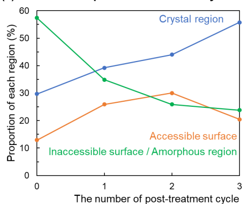
(e) Tension-free post-treatment on polynosic
