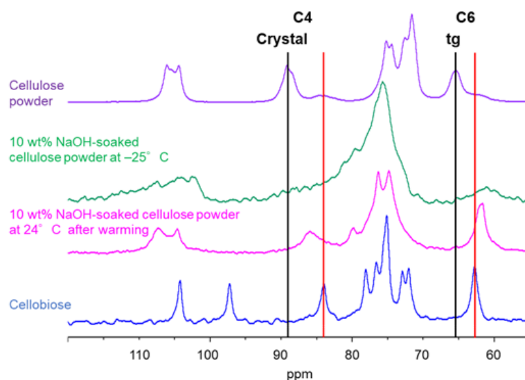
Fig. 2-7. Solid-state ^{13}\text{C} NMR CP/MAS NMR spectra. Color code: purple line, cellulose powder (cellulose \text{I}_\beta rich); green line, 10 wt% NaOH-soaked cellulose powder (the spectrum was recorded at -25^\circ\text{C} after cooling the sample from 24^\circ\text{C} to -25^\circ\text{C} ); pink line, 10 wt% NaOH-soaked cellulose powder (the spectrum was recorded at 24^\circ\text{C} after cooling the sample from 24^\circ\text{C} to -25^\circ\text{C} , followed by warming to 24^\circ\text{C} ); blue line, as-received cellobiose.
