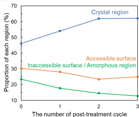
(c) Tension-free post-treatment on rayon
