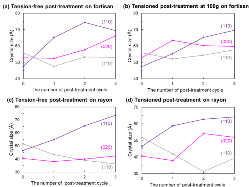
Fig. 3-16. The crystal size of (110̄) plane (gray line), (110) plane (purple line), and (020) plane (pink line) estimated from XRD profiles in (a) the tension-free multicyle post-treatment on fortisan, (b) the tensioned multicyle post-treatment on fortisan applied tension at 100 g on single strand, (c) the tension-free multicyle post-treatment on rayon and (d) the tensioned multicyle post-treatment on rayon.
