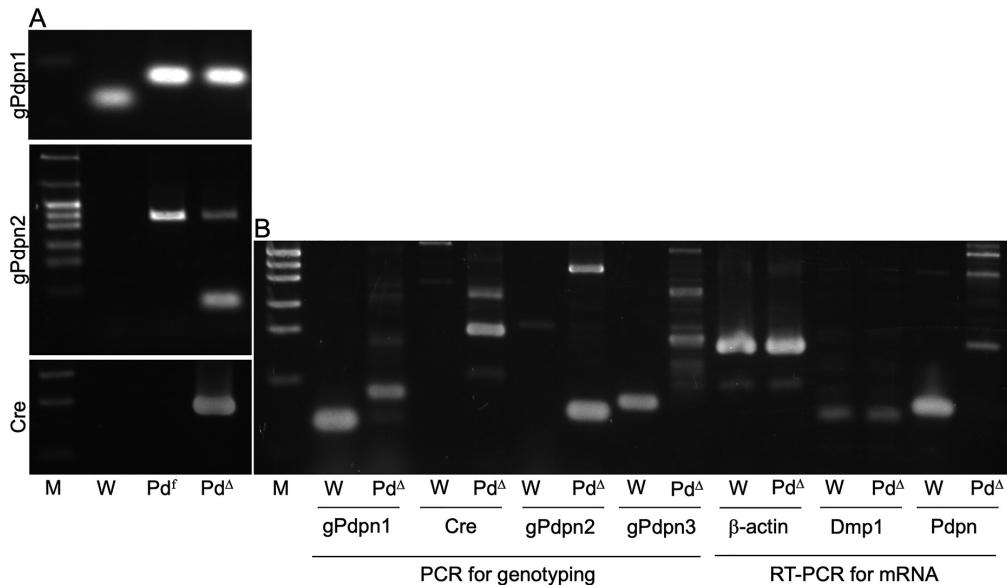
Figure 3. Genotyping and RT-PCR of tail and cultured osteoblasts. (A) The genotyping of the tail. For the gPdpn1, the gene containing loxP after the Pdpn exon 3 in the allele of the Pdpn fl (208 bp) was detected from the tails of the Pdpn fl/fl mice and Dmp1-Cre ; Pdpn Δ/Δ mice, while the gene without loxP after Pdpn exon 3 was detected from the wild-type mice (128 bp). For the gPdpn2, the gene flanking the FRT and loxP after the Pdpn exon 3 (1,096 bp) in the allele of Pdpn fl was detected from the tail of the Pdpn fl/fl mice while not detected from the tail of the wild-type mice. Both of the intact gene (1,096 bp) and the gene cleaved by the Cre recombinase (174 bp) was detected from the Dmp1-Cre ; Pdpn Δ/Δ mice. The gene of Cre recombinase (472 bp) was detected from the tail of the Dmp1-Cre ; Pdpn Δ/Δ mice. (B) The genotyping and RT-PCR of cultured osteoblasts. For the gPdpn1, the gene containing loxP after the Pdpn exon 3 (208 bp) was detected from the cultured osteoblasts of Dmp1-Cre ; Pdpn Δ/Δ mice while the gene without loxP after the Pdpn exon 3 was detected from the wild-type mice (128 bp). The gene of Cre recombinase (472 bp) was detected from the cultured osteoblasts of Dmp1-Cre ; Pdpn Δ/Δ mice while not detected from the cultured osteoblasts of wild-type mice. For the gPdpn2, both of the gene flanking the FRT and loxP after the Pdpn exon 3 (1,096 bp) and the gene cleaved by the Cre recombinase (174 bp) were detected from the cultured osteoblasts of Dmp1-Cre ; Pdpn Δ/Δ mice, while not detected from cultured osteoblasts of wild-type mice. For the gPdpn3, the gene flanking the Pdpn exon 3 (207 bp) was detected from the cultured osteoblasts of the wild-type mice while not detected from the cultured osteoblasts of the Dmp1-Cre ; Pdpn Δ/Δ mice. For RT-PCR, the mRNAs of β-actin (411 bp) and DMP-1 (165 bp) were detected at the same level from the cultured osteoblasts of both the wild-type and Dmp1-Cre ; Pdpn Δ/Δ mice. The mRNAs of podoplanin (Pdpn, 192 bp) were detected from the cultured osteoblasts of wild-type mice but not from the cultured osteoblasts of Dmp1-Cre ; Pdpn Δ/Δ mice. M: molecular weight marker; W: wild-type, Pd f : Pdpn fl/fl ; Pd Δ : Pdpn Δ/Δ
