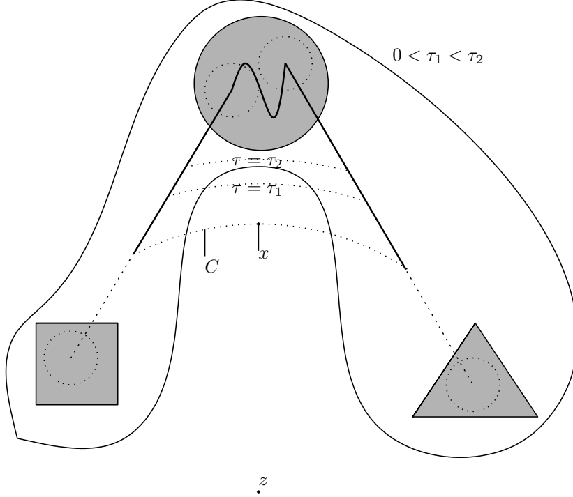
Figure 4: Strategy for x \in Co(O_-)
