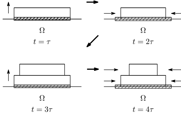
Figure 23: Birth and spread model.
