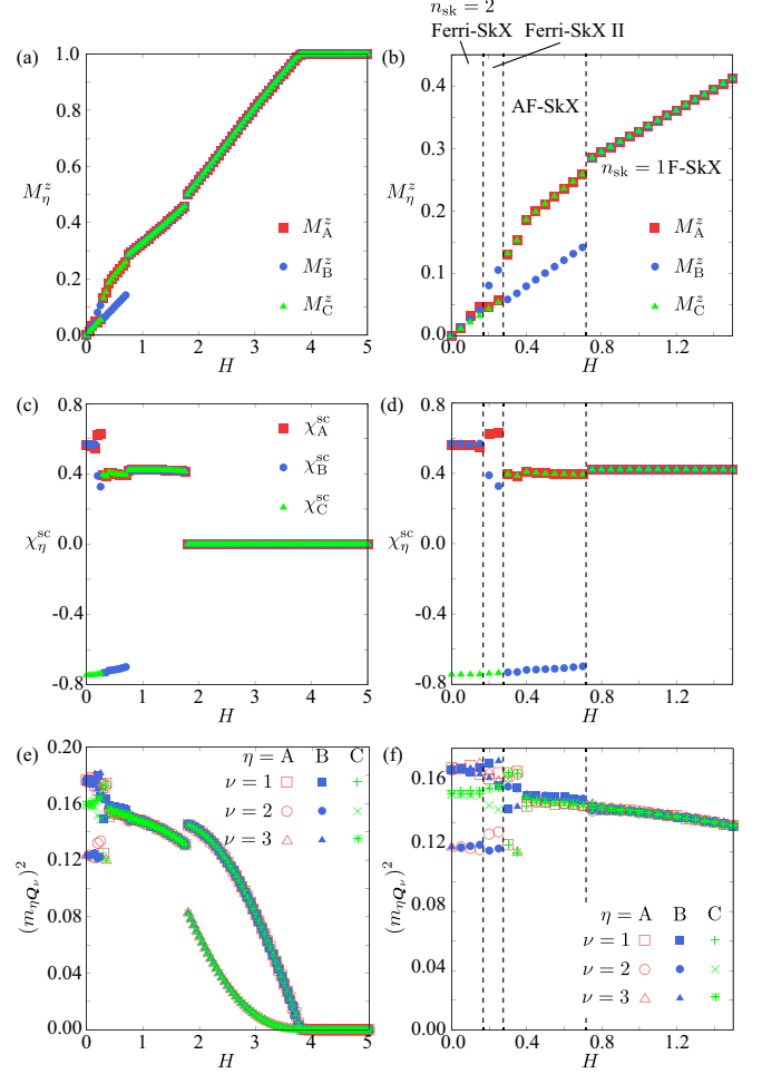
FIG. 5. The same plot as Fig. 4 with J^{\text{inter}} = 0.6 .
