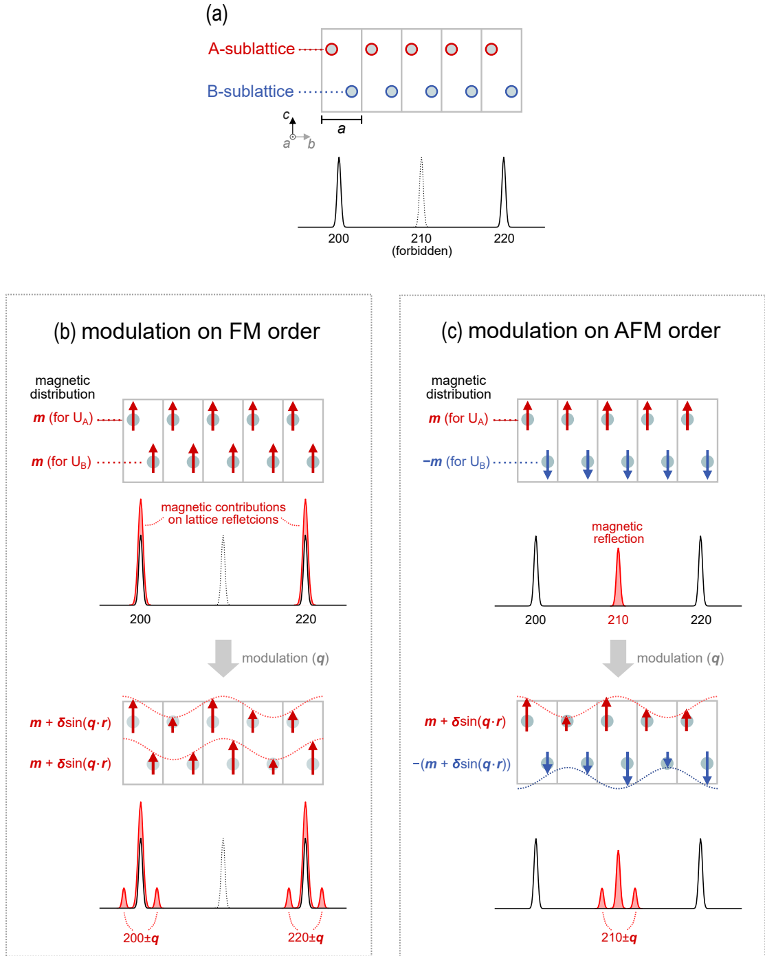
Figure 7.1: (Color online) (a) Schematic drawings of the crystal structure of UPt_2Si_2 and the diffraction pattern of the fundamental lattice reflections. The bold rectangles indicates the primitive unit cell in this crystal structure. The magnetic ordered states and the modulation on them with the propagation vector of q are shown for the case of (b) FM order and (c) AFM order. The expected diffraction peaks in each case are also depicted together.
