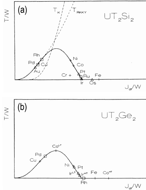
Figure 2.4: The comparison of experimental magnetic (or HO) transition temperatures in UT_2Si_2 and UT_2Ge_2 with the hybridization strength J_{df} estimated by Endstra et al [41]. The curve denotes the magnetic phase expected based on the Doniach model.
