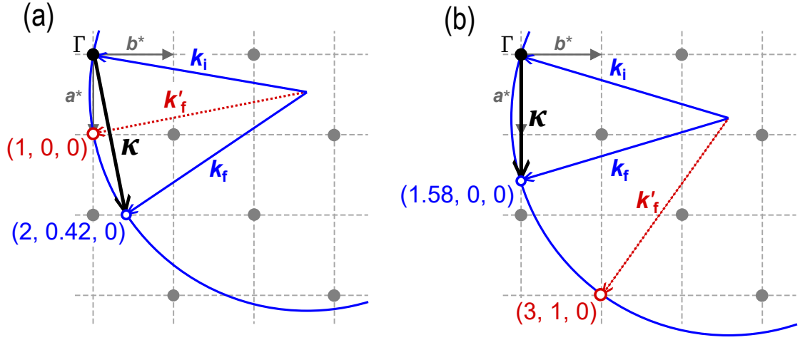
Figure 6.9: (Color online) The Ewald spheres on the (hk0) plane associated with the reflections at (a) (2, 0.42, 0, 0) and (b) (1.58, 0, 0, 0) in the unpolarized mode ( \lambda = 1.55 , k = 4.05 \text{ }^{-1} ) are represented by blue solid-line circles. The blue thin arrows indicate the wave vectors of the incident ( \mathbf{k}_i ) and scattered ( \mathbf{k}_f ) neutrons in the Bragg conditions for the target reflections. The scattering vectors are denoted by the black bold arrows. The red circle in each panel denotes a reflection present on the Ewald sphere besides the target reflection. Scattering from \mathbf{k}_i to both \mathbf{k}_f and \mathbf{k}'_f occurs simultaneously. Additionally, \mathbf{k}'_f can cause multiple scattering in the sample, such as diffracting to \mathbf{k}_f or diffracting back to \mathbf{k}_i and then to \mathbf{k}_f . These processes can lead to a non-essential enhancement of the scattering intensity in the target reflections.
