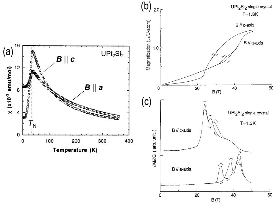
Figure 2.5: Data from magnetization measurements (under magnetic fields \parallel c - and a -axes) on the single crystal of UPt 2 Si 2 [45]: (a) the temperature dependence of the magnetic susceptibility, (b) the magnetization process, and (c) the field dependence of the differential susceptibility derived from the data in (b).
