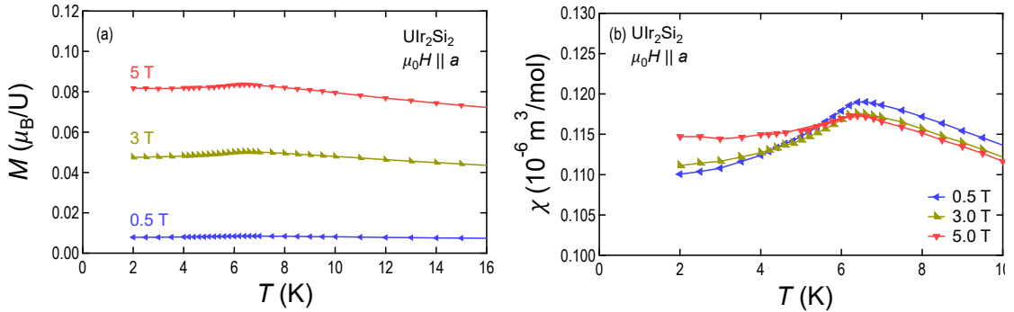
Figure 8.4: (Color online) (a) Temperature dependences of the magnetization under the magnetic field of 0.5–5 T along the a -axis. (b) The magnetic susceptibilities \chi converted from the measured magnetizations.
