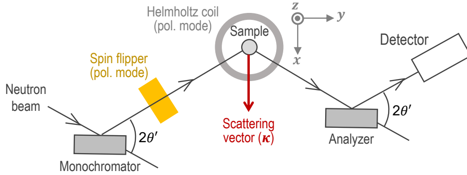
Figure 6.2: (Color online) A Schematic view of a triple-axis spectrometer (PONTA). The Cartesian coordinate xyz is introduced with the z -axis perpendicular to the scattering plane and the x -axis parallel to the scattering vector \kappa .
