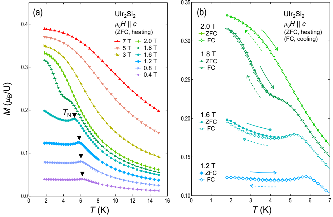
Figure 8.3: (Color online) (a) Temperature dependences of the magnetization under the magnetic field of 0.4–7 T along the c -axis, measured in a heating process after ZFC. The triangle marker indicates T_N under each magnetic field, which is evaluated as the temperature of the local maximum in the magnetization. (b) Enlarged magnetizations and the temperature hystereses in the magnetizations. The open symbols represent the data measured in the cooling processes after FC.
