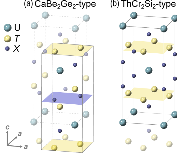
Figure 2.2: (Color online) Crystal structures of \text{RT}_2\text{X}_2 : (a) \text{CaBe}_2\text{Ge}_2 -type, (b) \text{ThCr}_2\text{Si}_2 -type. The colored shaded areas enhance the visibility of the difference between these structures.
