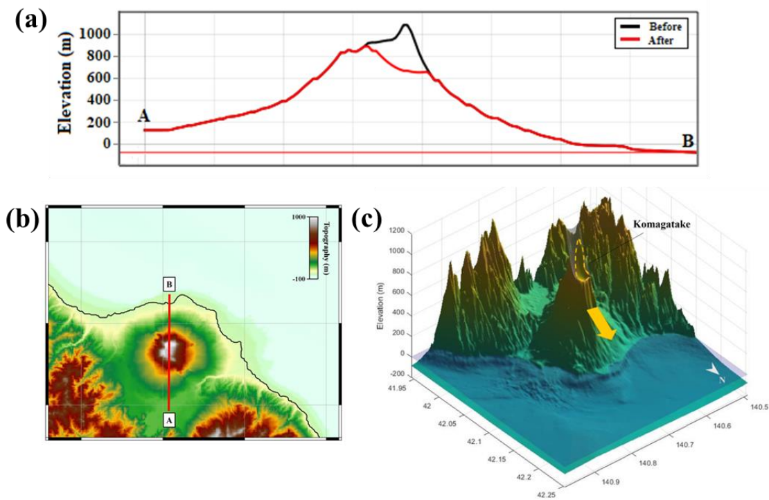
Figure 5.16 Collapse plane of the hypothetical collapse scenario 2 with total collapse volume of 0.63 \text{ km}^3 . (a) Elevation profile from the cross-section A-B indicated in (b) . (c) Main collapse plane at the north part of Komagatake volcano.
