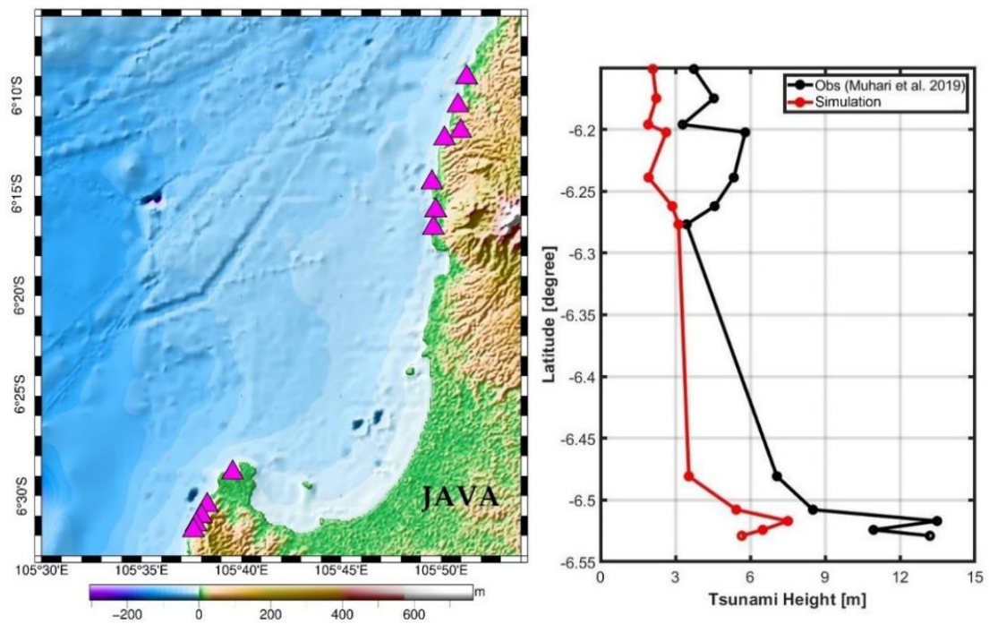
Figure 4.5. Runup height comparison between simulation (red) and observation (black) from the 2018 event along the coast of Java. The triangles in magenta color indicate the surveyed locations by Muhari et al. (2019).
