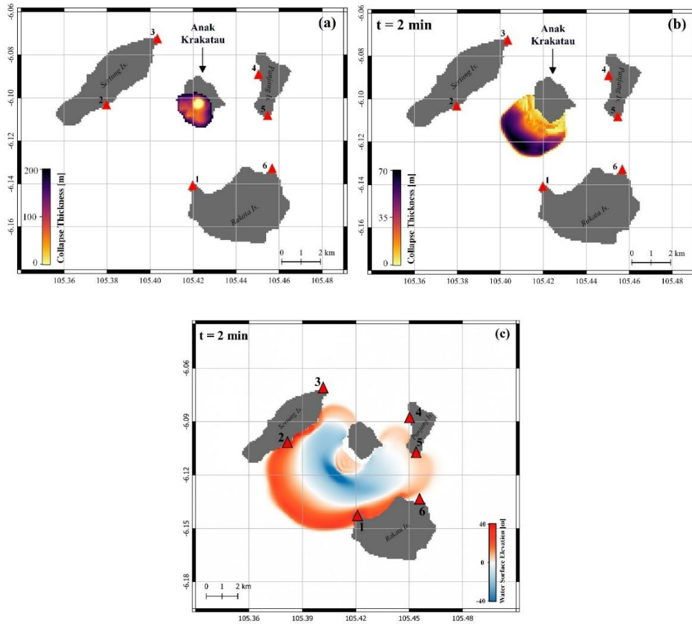
Figure 4.2. The landslide and tsunami generation at 2 min using VolcFlow model. (a) Initial collapse with 0.24 km 3 volume. (b) Collapse thickness at 2 min after the initial collapse. (c) Tsunami propagation simulation at 2 min.
