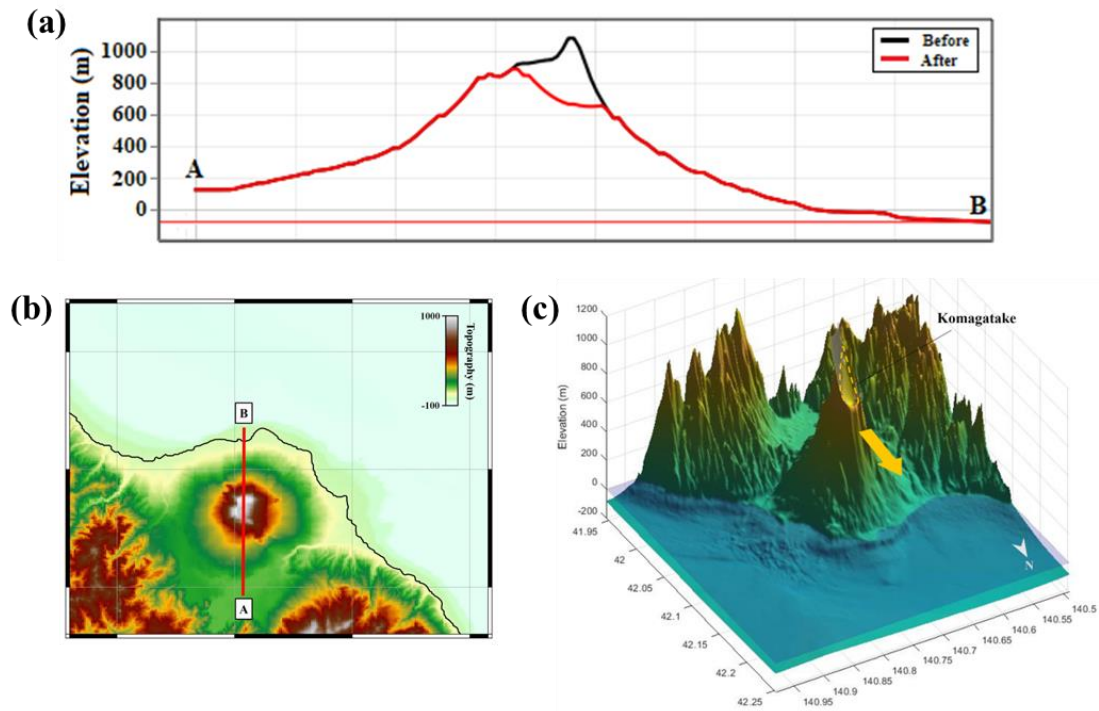
Figure 5.20 Collapse plane of the hypothetical collapse scenario 3 with total collapse volume of 0.72 \text{ km}^3 . (a) Elevation profile from the cross-section A-B indicated in (b). (c) Main collapse plane at the northwest part of Komagatake volcano.
