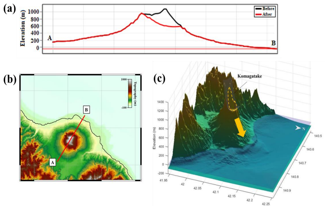
Figure 5.12 Collapse plane of the hypothetical collapse scenario 1 with total collapse volume of 0.87 \text{ km}^3 . (a) Elevation profile from the cross-section A-B indicated in (b). (c) Main collapse plane at the northeast of Komagatake volcano.
