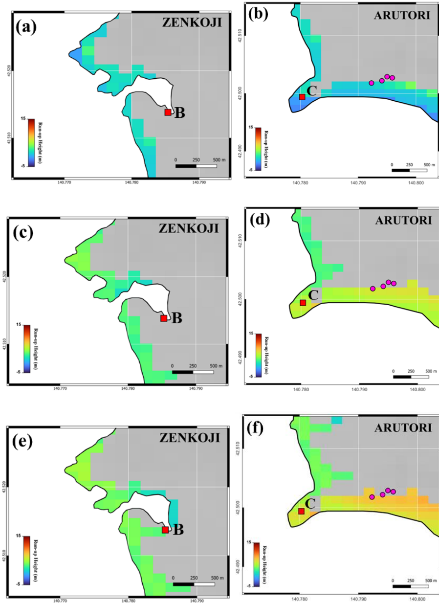
Figure 5.10 Inundation simulation at Zenkoji (left) and Arutori (right) using different collapse volumes of 1.2 \text{ km}^3 (a-b), 1.8 \text{ km}^3 (c-d), and 2.4 \text{ km}^3 (e-f).
