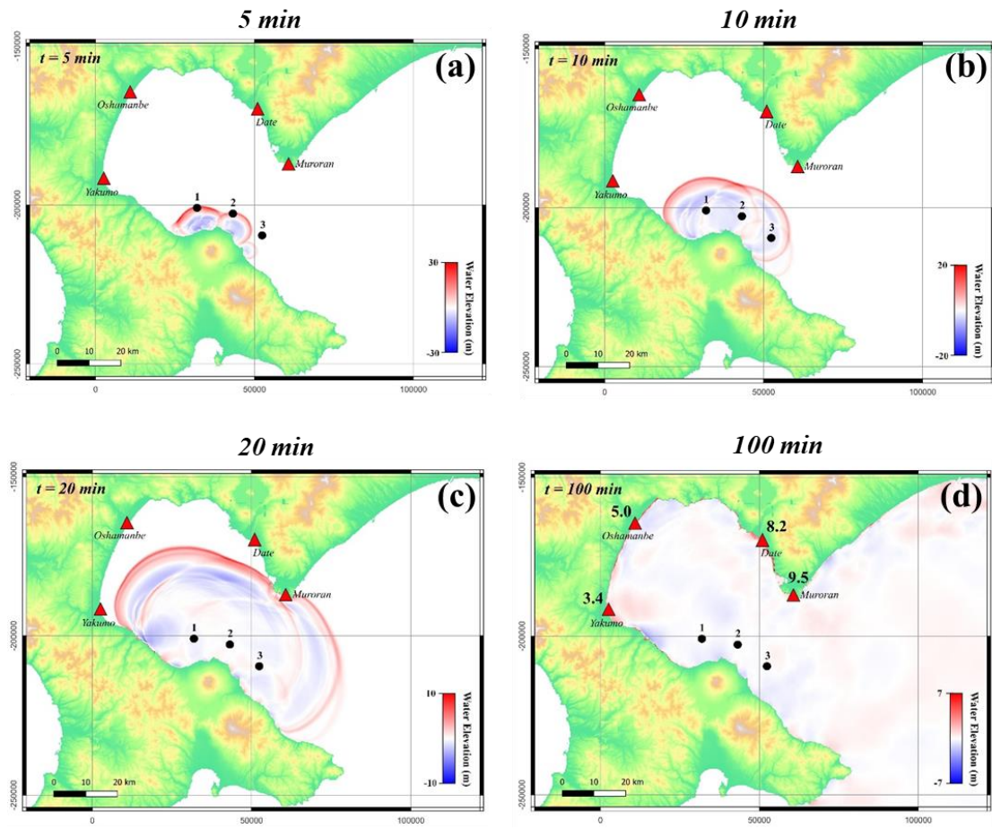
Figure 5.22 Snapshots of tsunami propagation simulation from hypothetical collapse scenario 3 at 5 min (a), 10 min (b), 20 min (c), and 100 min (d). The black circle indicates the three virtual observation points. The red triangles and label in the fig (d) indicate the maximum tsunami height at those locations.
