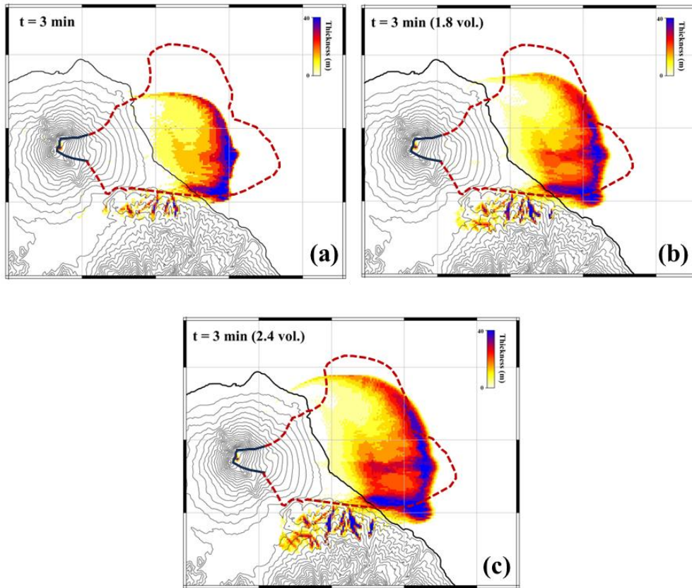
Figure 5.11 Collapse thickness deposit of 1.2 km 3 (a), 1.8 km 3 (b), and 2.4 km 3 (c) collapse volumes from 3 minutes landslide simulation. Red-dashed line indicates the depositional area from the study of Yoshimoto et al. (2003).
