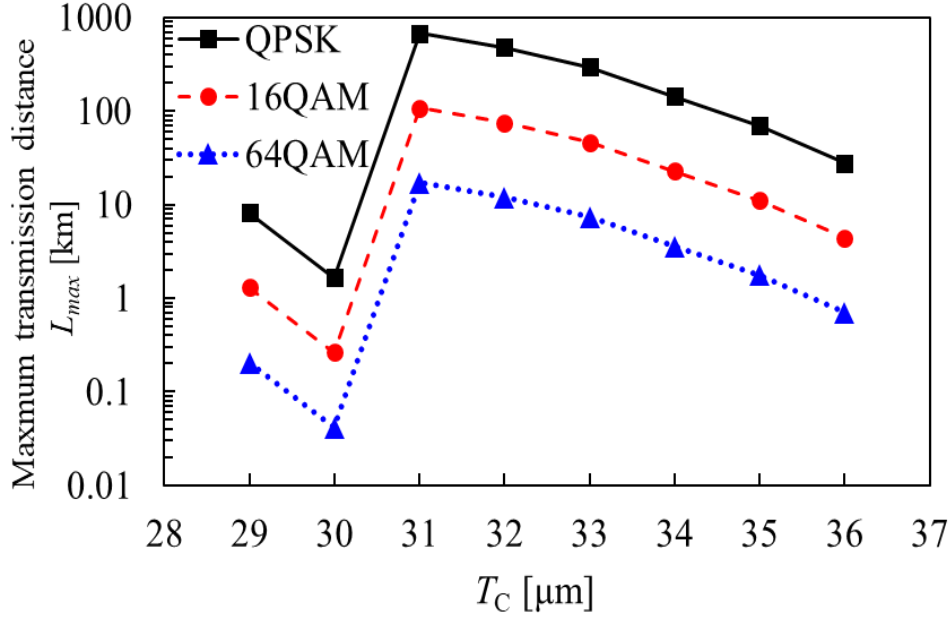
Fig. 7. The Maximum transmission distance L_{\text{QPSK}} , L_{16\text{QAM}} , and L_{64\text{QAM}} as a function of T_C , where N = 6 , \lambda = 1550 nm, d = 1 m, and R_b = 140 mm.
