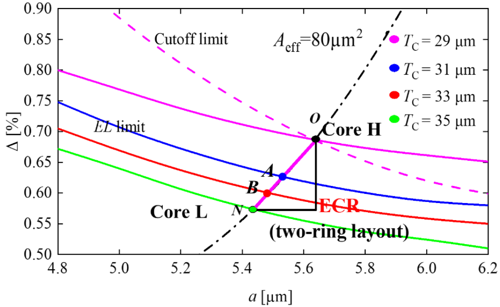
Fig. 10. Distribution of the core parameters for core H and core L for the C-band, where T_C = 29, 31, 33 , and 35\text{ }\mu\text{m} .
