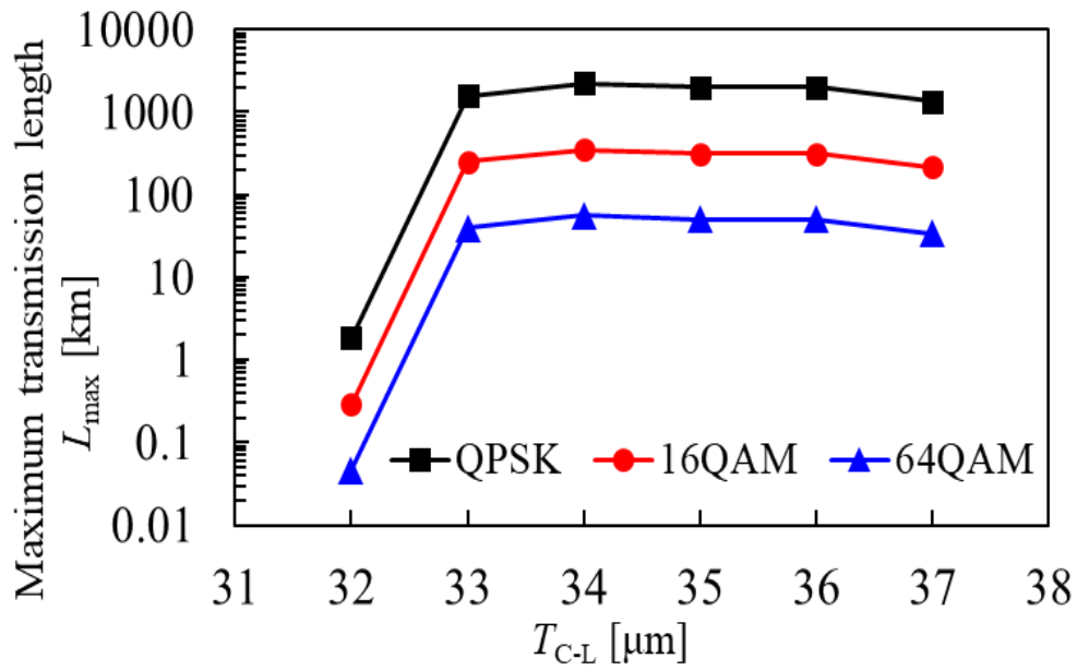
Fig. 37. Comparison of transmission length between the different format signals for Hetero-MCFs with the two-ring core layout for C+L-band.
