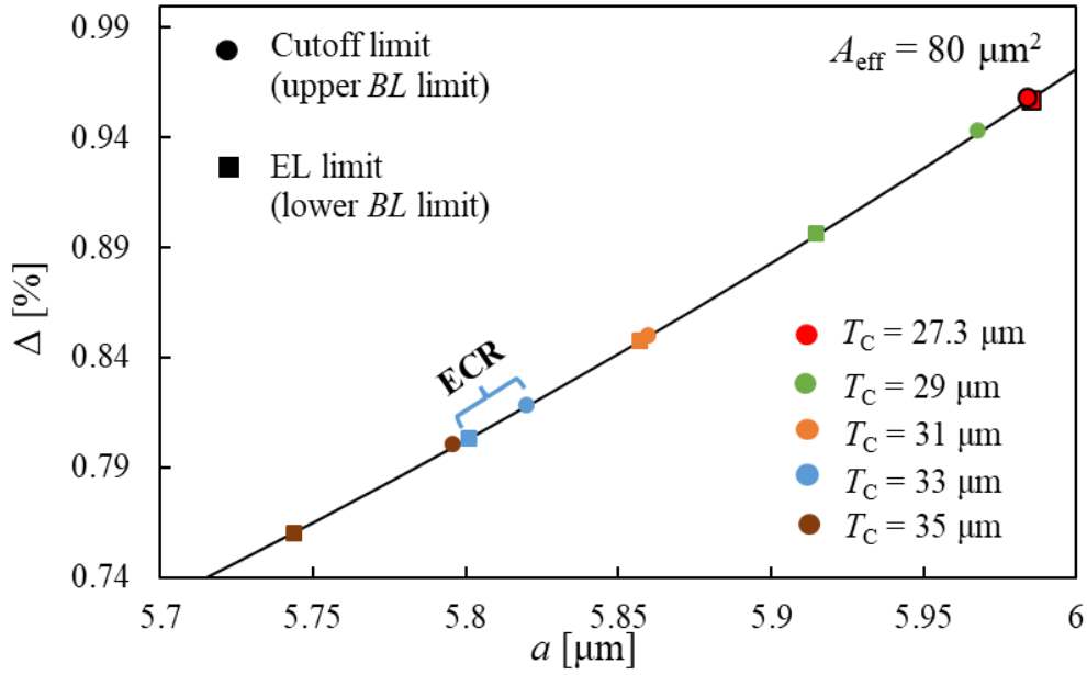
Fig. 21. The core parameters (core radius a and \Delta ) and their relationship of cutoff limit, EL limit, and A_{\text{eff}} at \lambda = 1550 nm, where T_C = 27.3, 29, 31, 33 , and 35 \mu\text{m} .
