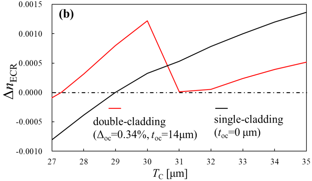
Fig. 17. n_{\text{eff}} and \Delta n_{\text{ECR}} for \text{LP}_{11} modes between ECR limit points in single- and double-cladding Hetero-MCF as a function of T_C ( T_C = 27.3\text{-}35 \mu\text{m} ). (a) n_{\text{eff}} as a function of T_C . (b) \Delta n_{\text{ECR}} as a function of T_C .
