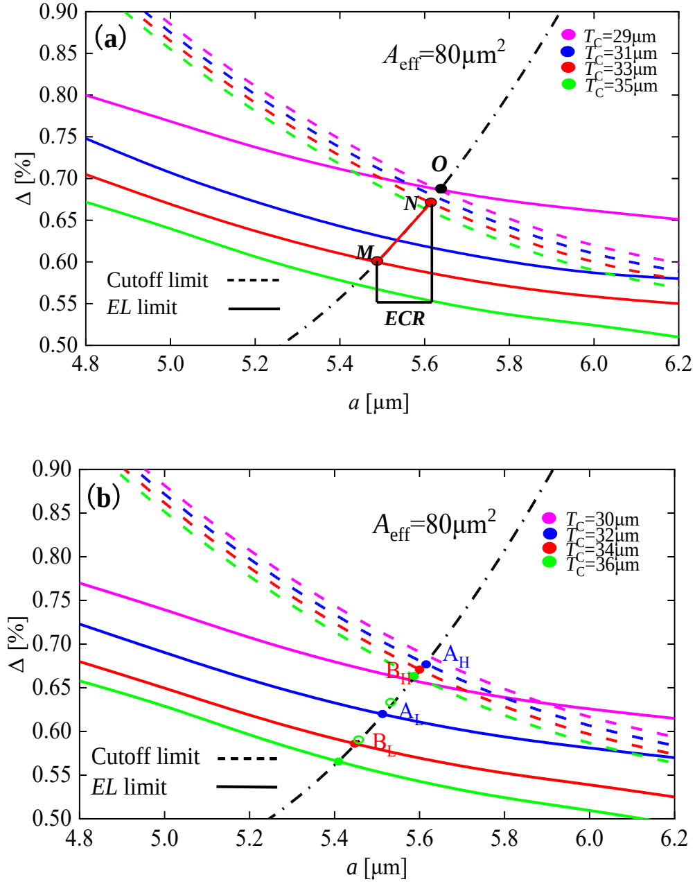
Fig. 3. Relationship between the core parameters and effective indices for the C-band: (a) T_C = 29, 31, 33, \text{ and } 35 \mu\text{m} ; (b) T_C = 30, 32, 34, \text{ and } 36 \mu\text{m} .
