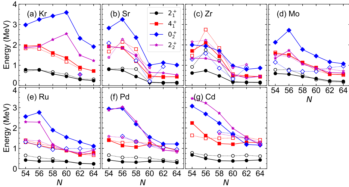
FIG. 2. Calculated excitation spectra of the 2_1^+ , 4_1^+ , 0_2^+ , and 2_2^+ states of the even-even Kr, Sr, Zr, Mo, Ru, Pd, and Cd isotopes (solid symbols connected by solid lines). The experimental data (open symbols connected by dotted lines) are adopted from the NNDC database [73].
