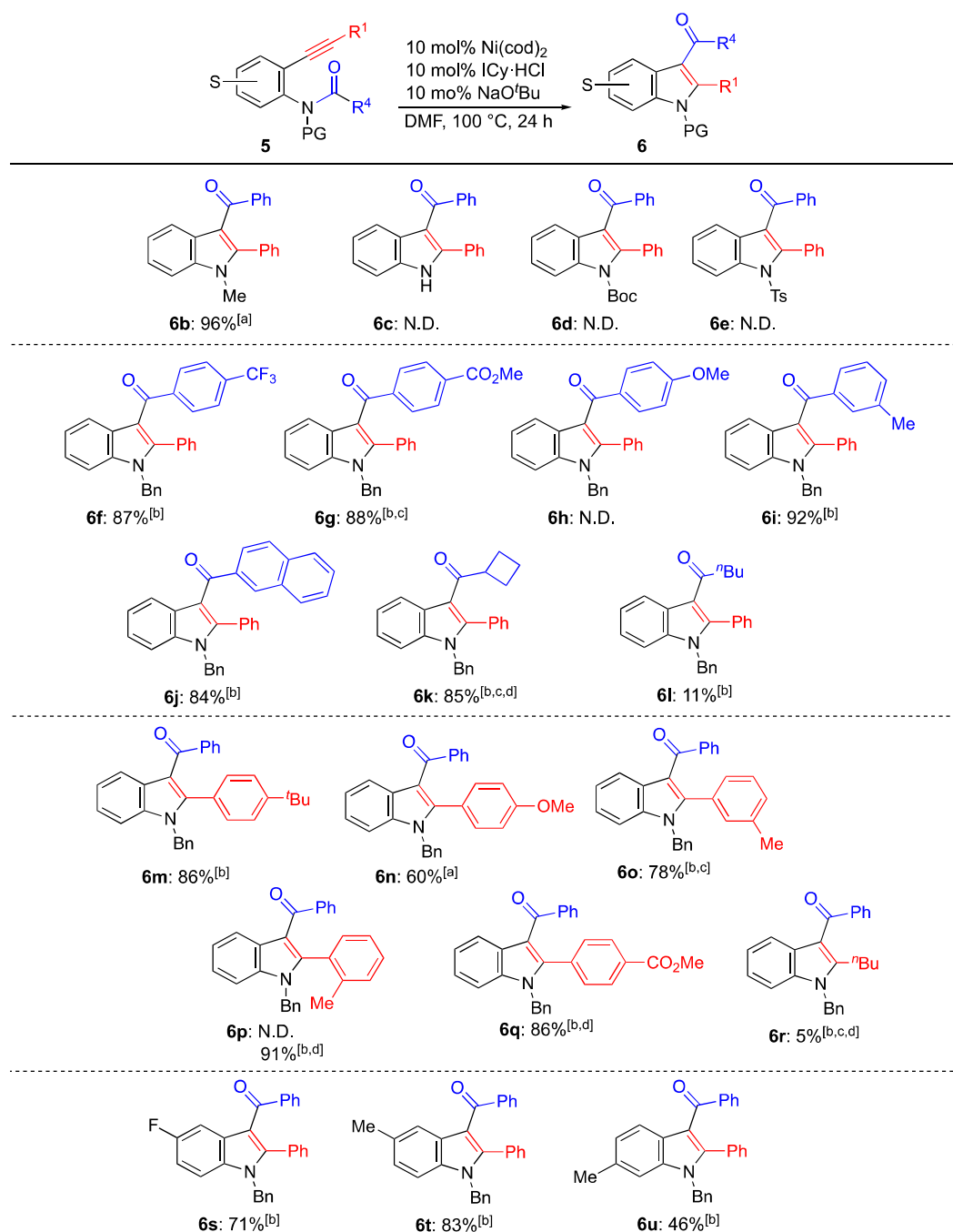
Figure 1. Scope and limitations of the reaction.
