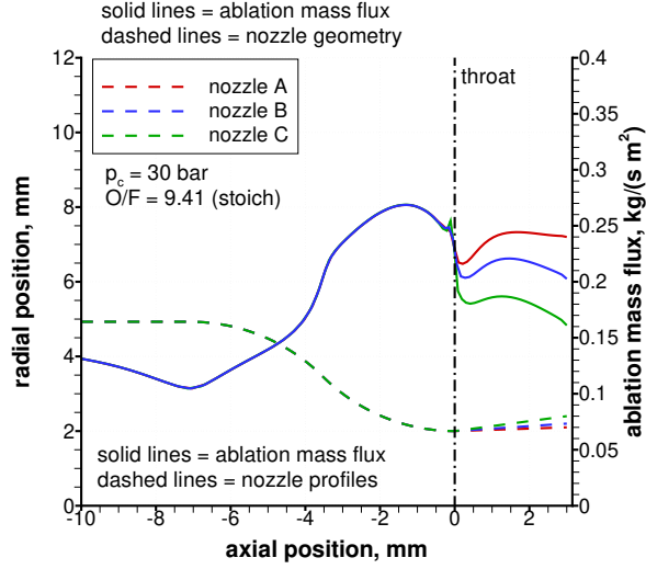
Figure 8 Effects of the nozzle divergent angle on the ablation mass flux distribution along the nozzle length.
