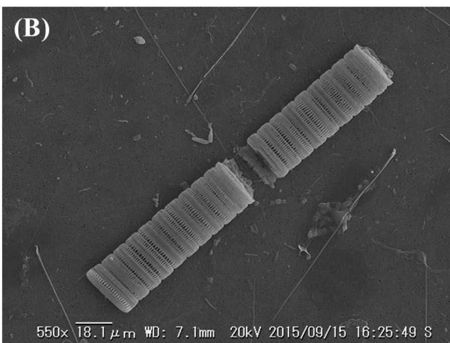
Figure 8. Scanning electron micrographs of the pennate diatom Neodenticula seminae with elongated chains from the +DFB bottles (A) at stations C5 and (B) A5.
