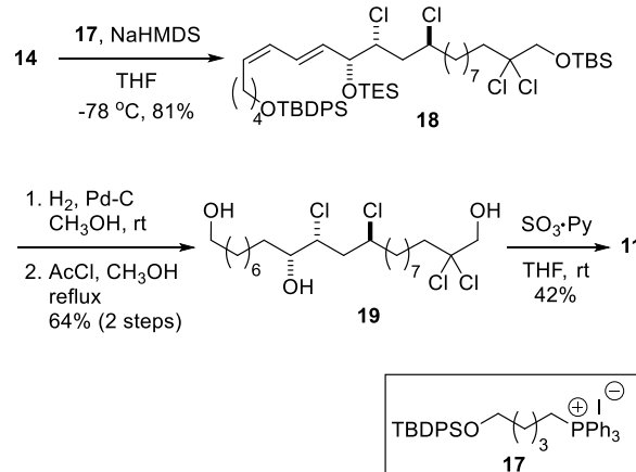
Scheme 3. Synthesis of trisulfate derivative 11 .
