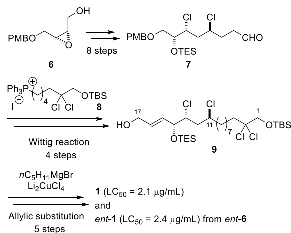
Scheme 1. Previous total synthesis of 1 .
