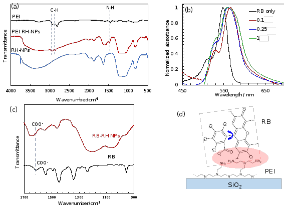
Figure 3 (a) FT-IR spectra of PEI, PEI RH-NPs, and RH-NPs. (b) Normalized absorption spectra of free RB and suspensions of RB-RH NPs with different values of X_{RB/PEI} ( X_{RB/PEI} = 0.1, 0.25 , and 1 ). (c) FT-IR spectra of RB and RB- RH NPs. (d) Schematic picture of possible interaction between the electrostatic interaction between the carboxylate groups of RB and PEI-modified silica surface.
