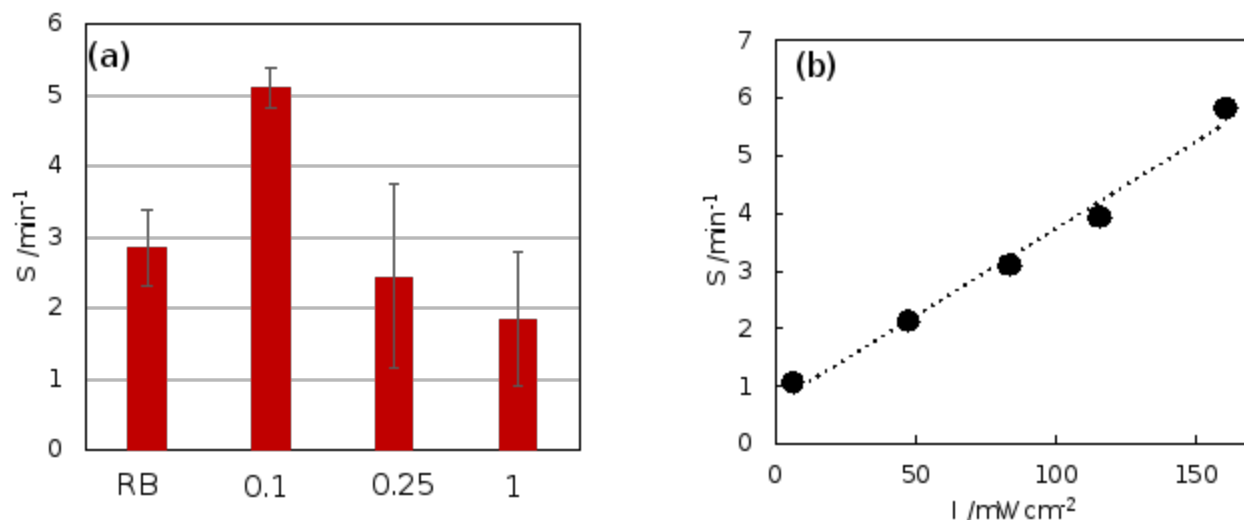
Figure 5 (a) ^1\text{O}_2 generation efficiency ( S ) of RB and RB-RH NPs ( X_{\text{RB/PEI}} = 0.1, 0.25 , and 1.0 ). (b) The values of S as a function of the white light irradiation intensity.
