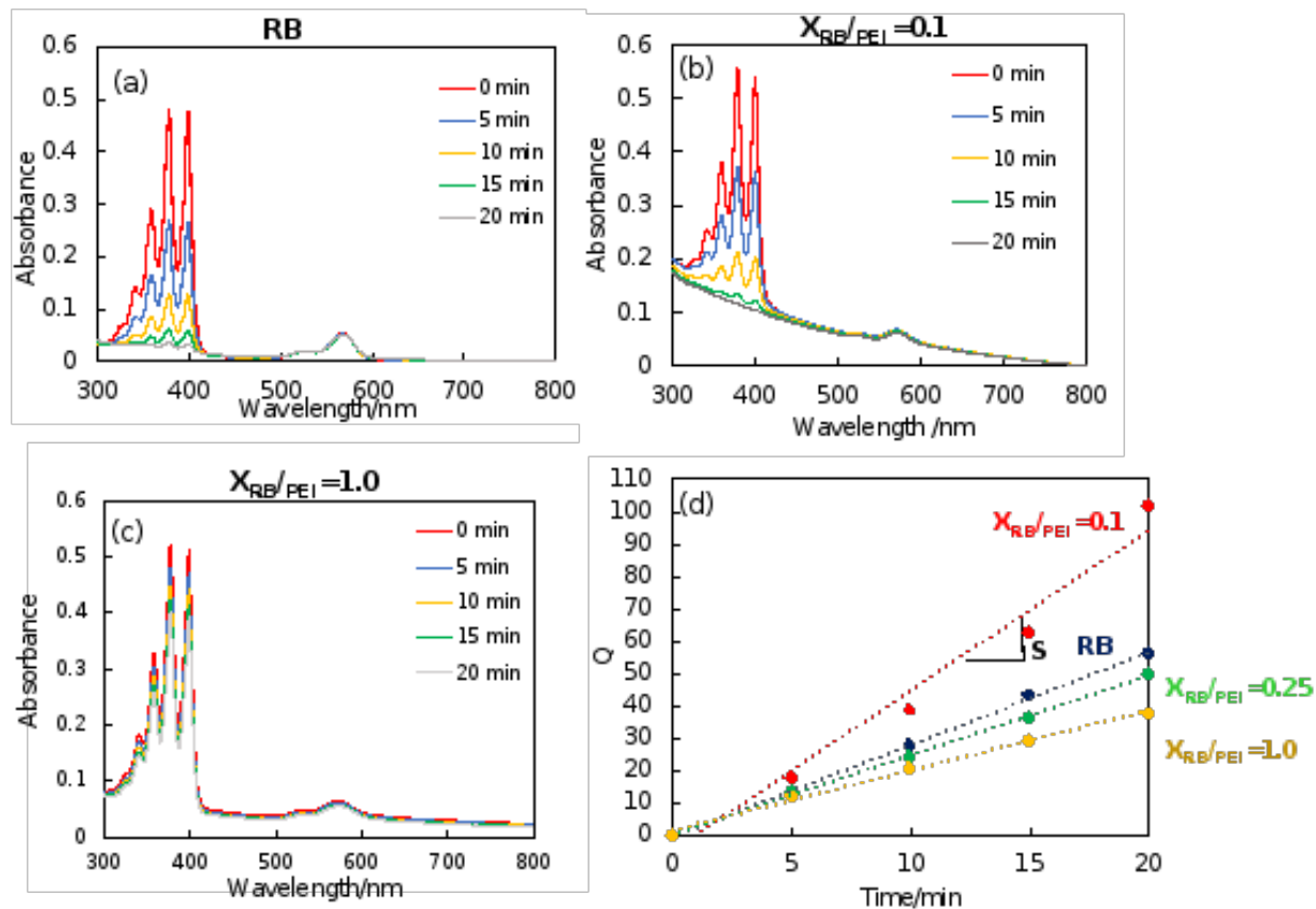
Figure 4 UV-Vis spectra of ABDA during white LED irradiation in the presence of (a) RB, (b) RB-RH NPs ( X_{RB/PEI} = 0.1 ), and (c) RB-RH NPs ( X_{RB/PEI} = 1.0 ). (d) Normalized ABDA absorbance at 378 nm ( Q ) as a function of irradiation time in the presence of RB or RB-RH NPs ( X_{RB/PEI} = 0.1, 0.25 , and 1.0 ).
