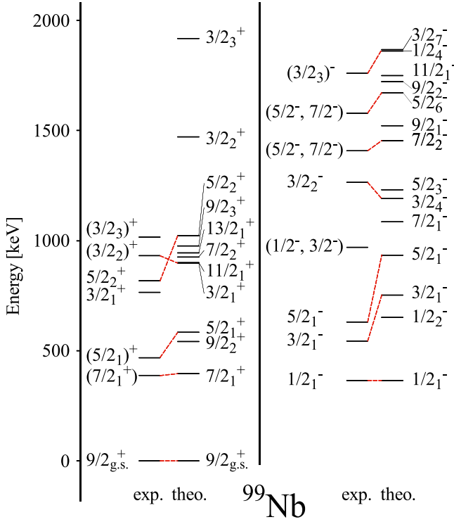
FIG. 5. Experimental [38] vs theoretical low energy level scheme of ^{99}\text{Nb} using IBFM-CM calculations. Positive (left) and negative parity (right) states are shown. Theoretically calculated states of the K = 1/2^- band originating at 0.745 MeV are omitted for better clarity.
