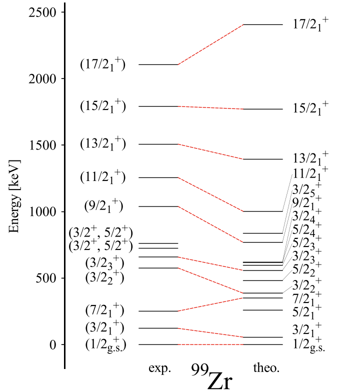
FIG. 6. Experimental [38] vs theoretical low energy level scheme of ^{99}\text{Zr} using SCMF-IBFM calculations. Here, only a selected choice of theoretical energy levels are displayed for better clarity.
