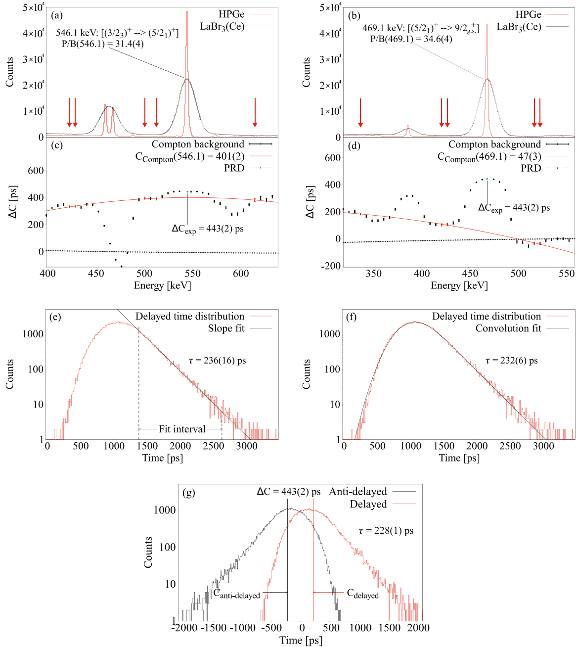
FIG. 4. (a) Energy spectra from HPGe and \text{LaBr}_3(\text{Ce}) detectors showing the 546.1 keV feeding transition of the (5/2_1)^+ state in ^{99}\text{Nb} , gated on the (5/2_1)^+ \rightarrow 9/2_{\text{g.s.}}^+ (469.1 keV) transition in a spectrum measured by another \text{LaBr}_3(\text{Ce}) detector. (b) Energy spectra from HPGe and \text{LaBr}_3(\text{Ce}) detectors showing the 469.1 keV decaying transition of the (5/2_1)^+ state in ^{99}\text{Nb} , gated on the (3/2_3)^+ \rightarrow (5/2_1)^+ (546.1 keV) transition in a spectrum measured by another \text{LaBr}_3(\text{Ce}) detector. (c) Interpolated Compton background time response of the feeding transition. Data points in red [also labeled in the corresponding energy spectrum (a)] are used for the fitted curve. (d) Interpolated Compton background time response of the decaying transition. Data points in red [also labeled in the corresponding energy spectrum (b)] are used for the fitted curve. (e) Slope and convolution (f) method for the delayed time distribution of the (5/2_1)^+ state using gates on the (3/2_3)^+ \rightarrow (5/2_1)^+ feeding transition at 546.1 keV and the (5/2_1)^+ \rightarrow 9/2_{\text{g.s.}}^+ decaying transition at 469.1 keV. The antidelayed distribution was mirrored and summed up to increase statistics. The dashed lines in (e) represent the fit interval for the slope method. (g) Delayed and antidelayed time distribution for the (5/2_1)^+ state using \text{LaBr}_3(\text{Ce}) gates on the (3/2_3)^+ \rightarrow (5/2_1)^+ feeding transition at 546.1 keV and on the (5/2_1)^+ \rightarrow 9/2_{\text{g.s.}}^+ decaying transition at 469.1 keV.
