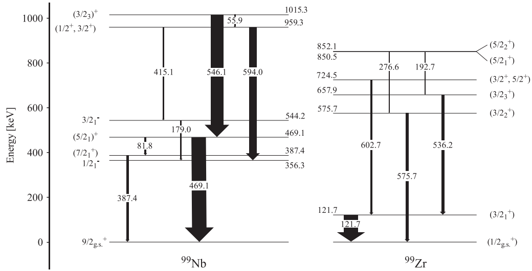
FIG. 3. Partial energy level scheme after \beta decay for both nuclei, ^{99}\text{Nb} and ^{99}\text{Zr} , respectively [38]. The scheme only contains transitions used to determine the lifetimes of this work.
