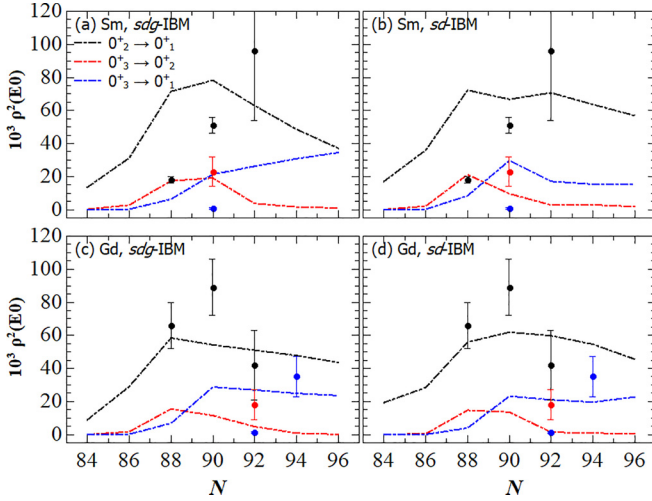
FIG. 18. \rho^2(E0; 0_1^+ \rightarrow 0_2^+) values as functions of the neutron number N for Sm and Gd isotopes, calculated with the mapped sdg -IBM (left column) and sd -IBM (right column). Experimental values are adopted from Refs. [38,44], and are plotted as solid circles.
