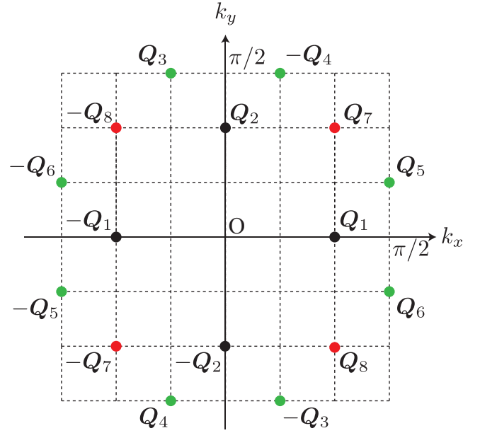
FIG. 1. Ordering wave vectors that give the dominant contributions in the momentum-resolved interactions. The coupling constants in the (\pm \mathbf{Q}_1, \pm \mathbf{Q}_2) , (\pm \mathbf{Q}_3, \pm \mathbf{Q}_4, \pm \mathbf{Q}_5, \pm \mathbf{Q}_6) , and (\pm \mathbf{Q}_7, \pm \mathbf{Q}_8) components of the momentum-resolved interactions are given by J_1 , J_2 , and J_3 in the model in Eq. (1), respectively.
