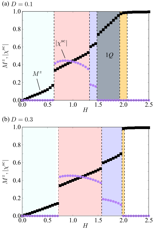
FIG. 5. H dependence of the z component of the magnetization M^z and the scalar chirality |\chi^{\text{sc}}| for (a) D = 0.1 and (b) D = 0.3 . The other parameters are the same as those in Fig. 3. 1Q represents the single- Q conical spiral state. The vertical dashed lines represent the phase boundaries between different magnetic phases.
