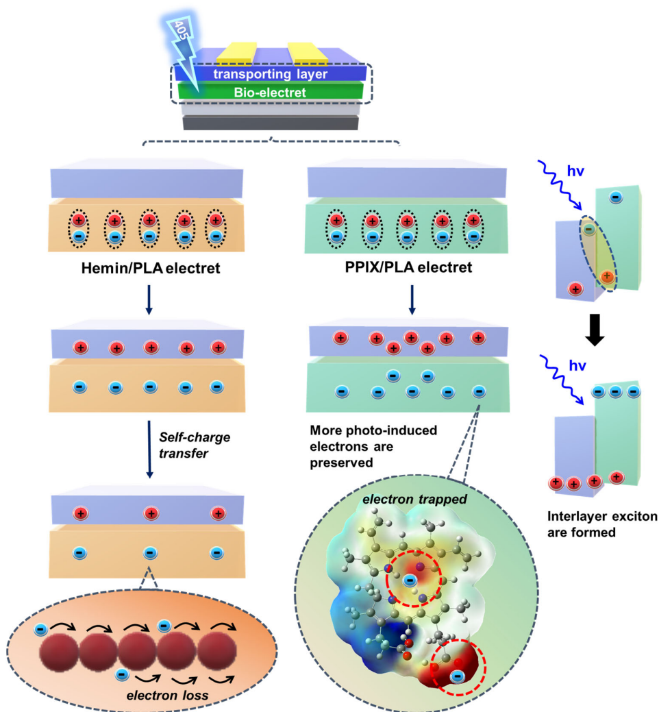
Figure 3. Schematic illustrations depicting the working mechanism of hemin/PLA and PPIX/PLA-based memories under light illumination and removal of light source. Optimization of PPIX by density functional theory and ESP on the 0.02 a.u. contours of the electronic density of three repeating units. The negative ESP regions are denoted in red and the positive regions are denoted in blue.
