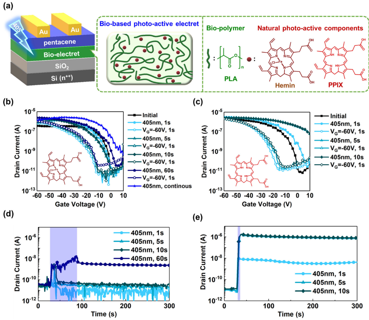
Figure 1. (a) Schematic illustration of the photo memory of the bio-based photoactive electrets.
