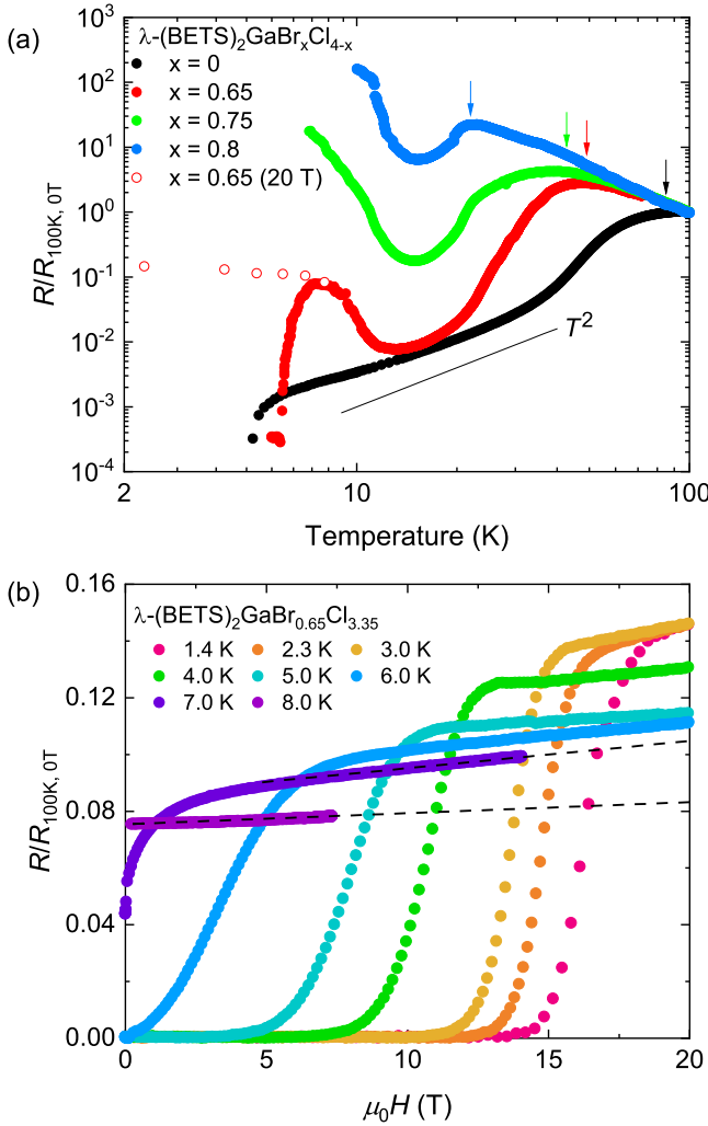
FIG. 3. (a) Temperature dependence of the scaled resistance R/R_{100K, 0T} of \lambda -(BETS) _2 GaBr _x Cl _{4-x} . The open red symbols are the resistivity of the compound with x = 0.65 in the normal state at 20 T. (b) Magnetic field dependence of the resistivity of the compound with x = 0.65 measured up to 20 T at each temperature.
