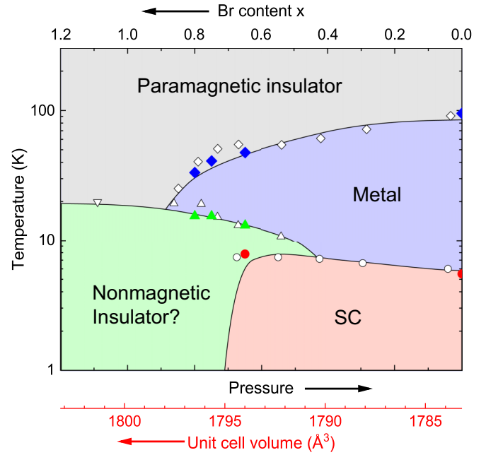
FIG. 2. p - T phase diagram of \lambda -(BETS) 2 GaBr x Cl 4- x . The red horizontal axis indicates the unit cell volume at room temperature [23]. The points marked with blue diamonds, green triangles, and red circles were determined in this study. The points marked with white diamonds, circles, triangles, and inverted triangles were determined by electrical resistivity and magnetic susceptibility measurements in previous studies [23].
