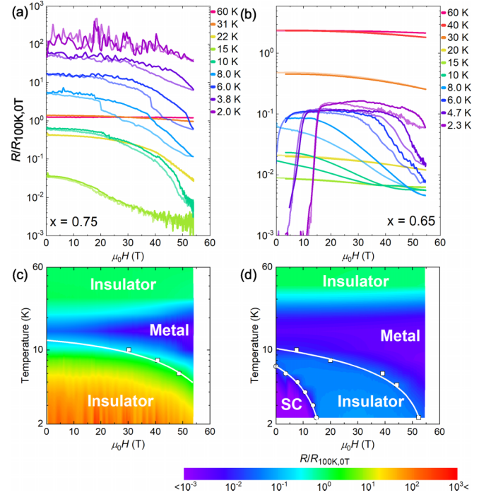
FIG. 4. (a), (b) Magnetic field dependence of the resistivity of the compound with x = 0.75 and 0.65 up to about 55 T. (c), (d) H - T phase diagram of the compound with x = 0.75 and 0.65 . The colors correspond to the value of the resistivity.
