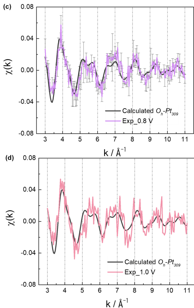
Figure 3-9. The fitting spectra based on O_h\text{-Pt}_{309} model for simulation potentials. Pt-Pt bond distance is set as 2.76 \text{ \AA} , DW=0.09 \text{ \AA} , S_0^2 = 1.0 , CN = 9.6 . Colored solid lines are observed EXAFS spectra with error, the black solid line is the calculated EXAFS spectra for Pt/HOPG model catalyst.
