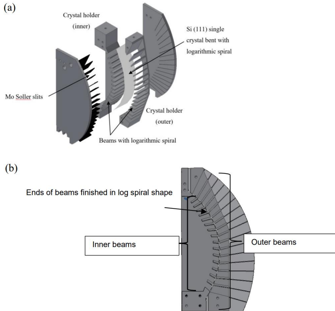
Figure 4-2. Home-made BCLA. (a) overall structures of home-made BCLA and (b) side view. The ends of the log-spirally shaped inner and outer beams sandwiched the thin Si crystal. [18]
