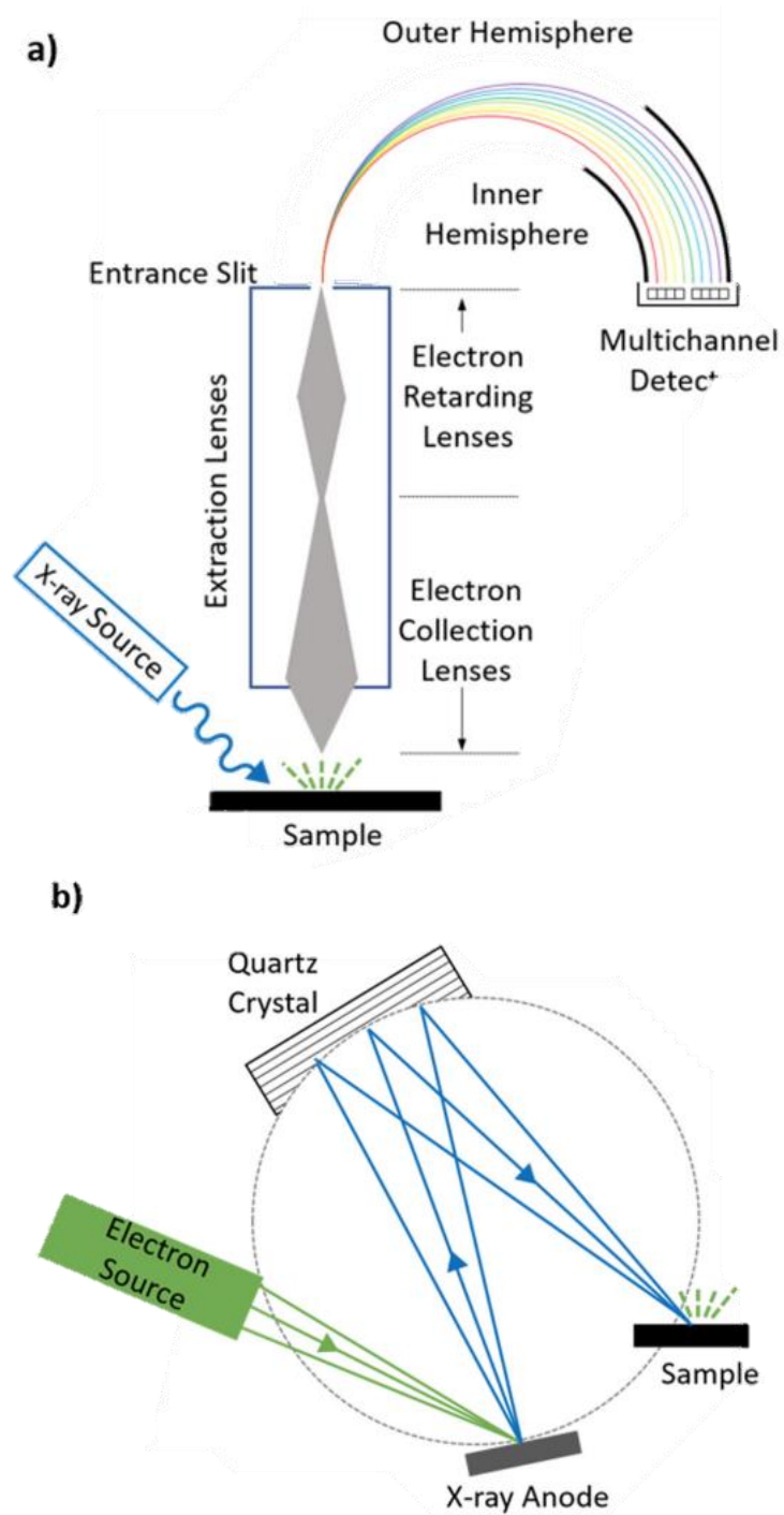
Figure 2-13 (a) XPS components and (b) monochromator configuration[10].
