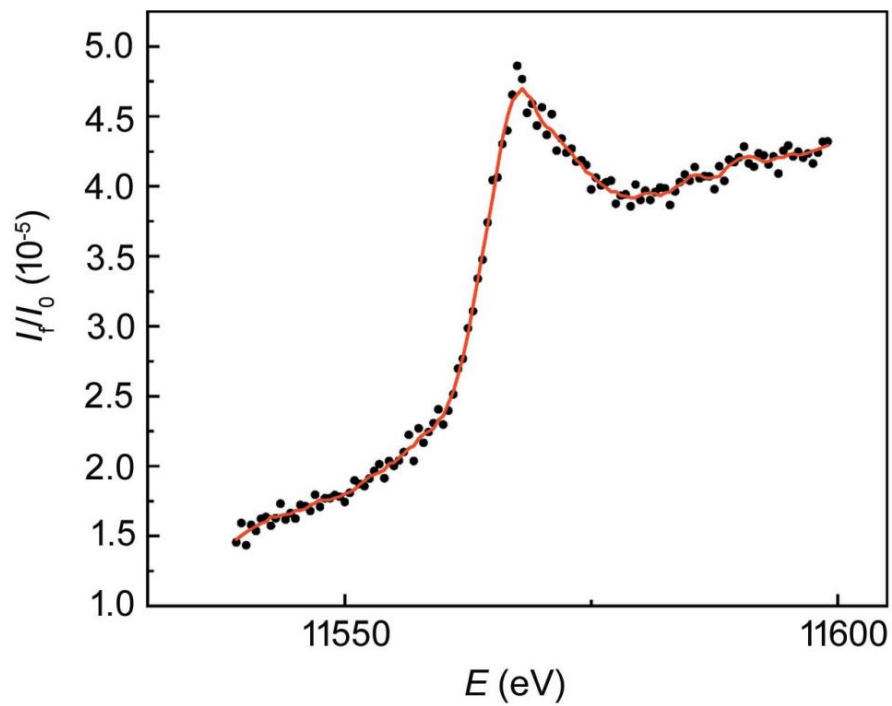
Figure 4-11. XANES spectra of 0.1 ML Pt on Au under -0.16 \text{ V}_{\text{AgAg/Cl}} in 0.1 \text{ M HClO}_4 . [18]
