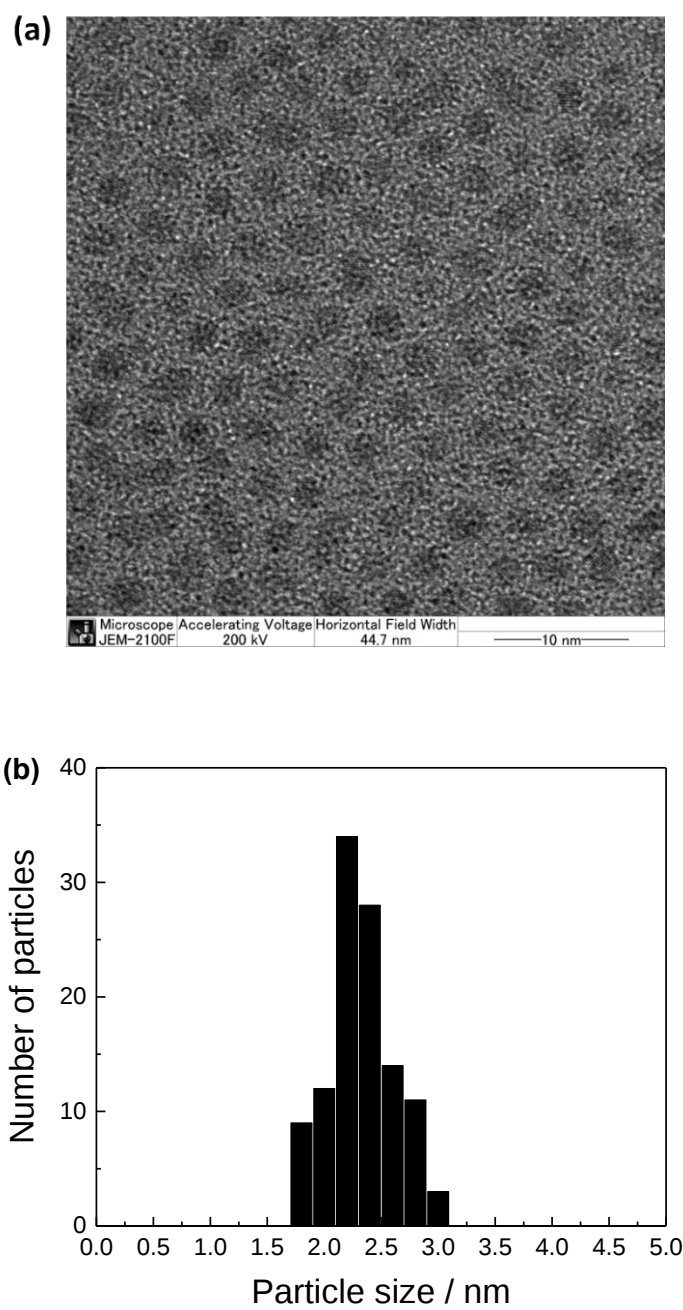
Figure 3-3. (a) TEM image of Pt NPs prepared via a two-phase liquid reduction method, (b) size histogram for Pt NPs in (a).
