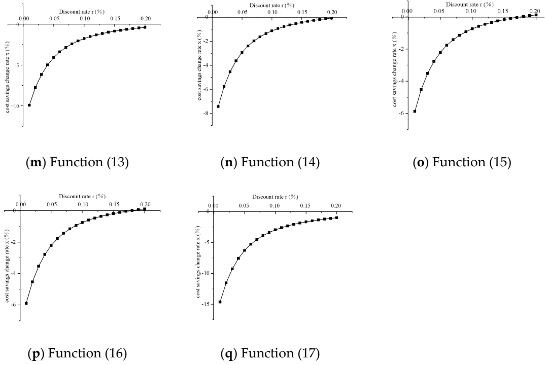
Figure 24. Two-factor sensitivity incremental cost and discount rate analysis graph in Changchun City.
