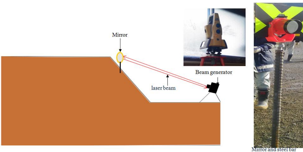
Fig.2.9: Schematic illustration of APS operation.
