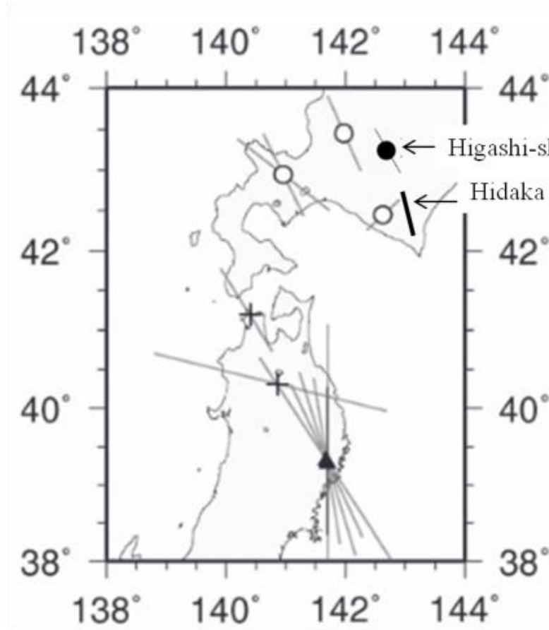
Fig.4.17: The estimated and measured regional stress as adopted from Naga et al., 2009.
