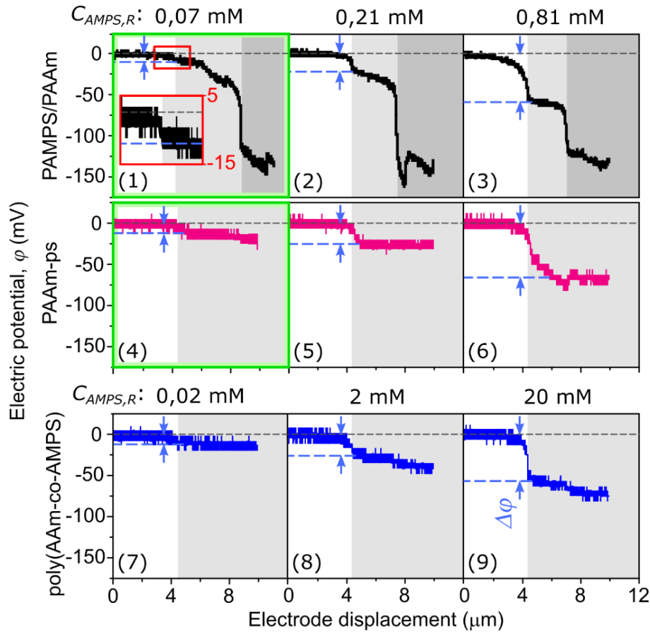
Figure 3: Electric potential profiles of hydrogels \Delta\phi measured by MET. DN hydrogels (PAMPS/PAAm, 1-3), the corresponding PAAm hydrogel synthesized from the AAm precursor solution (PAAm-ps, 4-6), and the co-polymer hydrogel (poly(AAm-co-AMPS), 7-9). The profile backgrounds in white, grey, and dark grey indicate the potential in the bathing solution, in the hydrogel surface layer, and in the hydrogel bulk, respectively. The potential differences between blue arrows indicate the electric surface potential \Delta\phi of hydrogels relative to bath solution ( C_s = 10^{-4} M NaCl aq. solution). (1 and 4) The green frames indicate the samples prepared with pre-washed PAMPS-w as the 1 st network.
