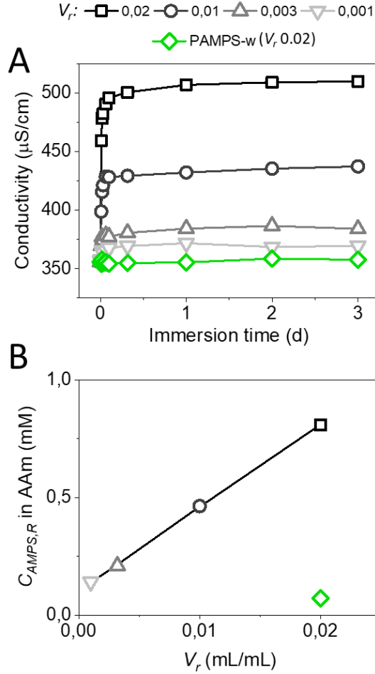
Figure 2: Determining the concentration of the 1st network monomer in the 2 nd network precursor solution. (A) The time profiles of ionic conductivity after the immersion of the as-prepared PAMPS hydrogels in AAm solutions with volume ratios ( V_r ) ranging from 0,02 to 0,001. (B) The equilibrium residual AMPS monomer concentration in AAm solutions C_{AMPS,R} as a function of the volume ratios ( V_r ). C_{AMPS,R} was calculated from conductivity. For comparison, the results after the immersion of the pre-washed PAMPS-w at V_r 0,02 was also shown.
