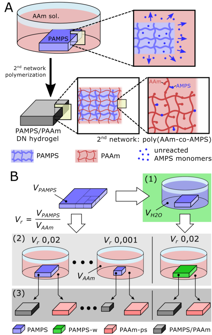
Scheme 1: (A) The scheme and (B) the methodology to prove the incorporation of unreacted residual 1 st network monomers (AMPS) in the 2 nd polymer network (PAAm). Performed by (1) monitoring the removal of unreacted monomers of as-prepared PAMPS hydrogel, (2) the detection of unreacted AMPS monomers in the 2 nd network precursor solution, and (3) the quantification of surface charge density of the synthesized PAMPS/PAAm DN and corresponding SN hydrogels.
