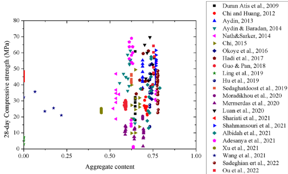
Fig. 4.7. Effect of aggregate content on strength
