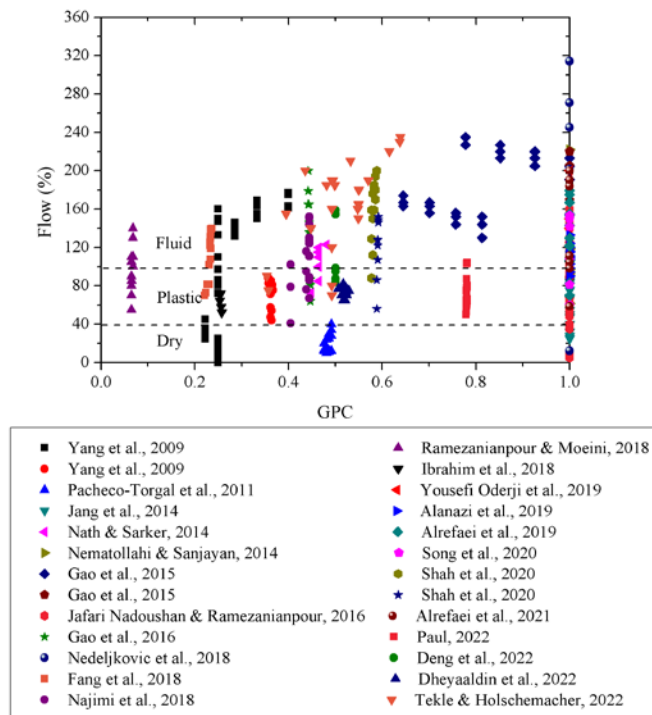
Fig. 3.7. Effect of GPC on workability
