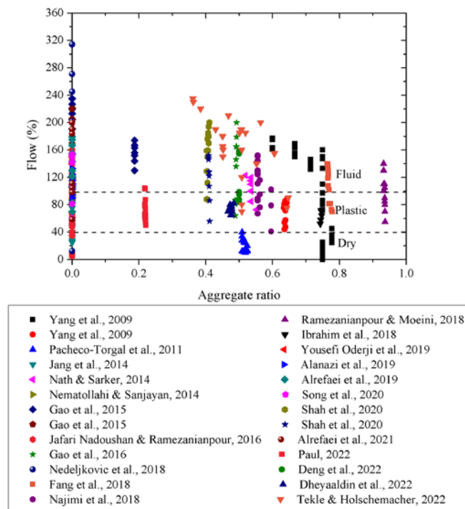
Fig. 3.8. Effect of aggregate content on workability
