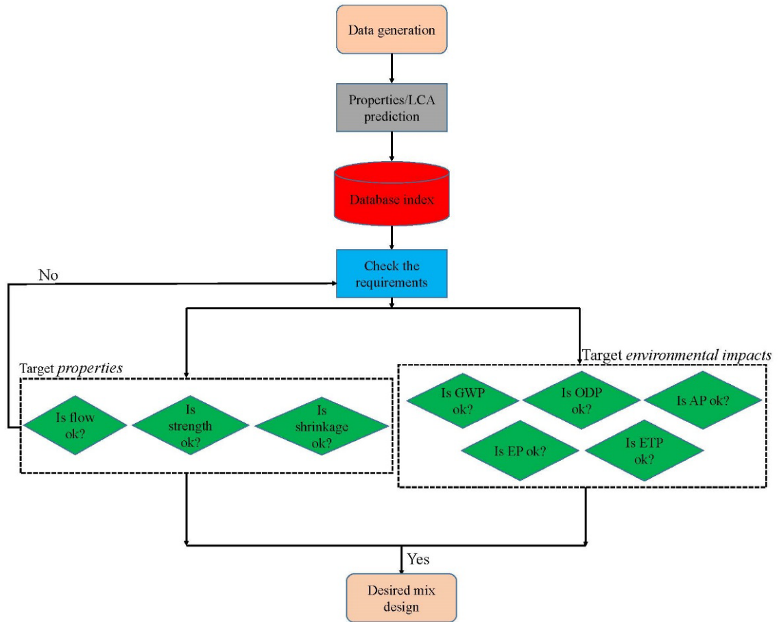
Fig. 6.15. Workflow for determining the sustainable AAM mix design
