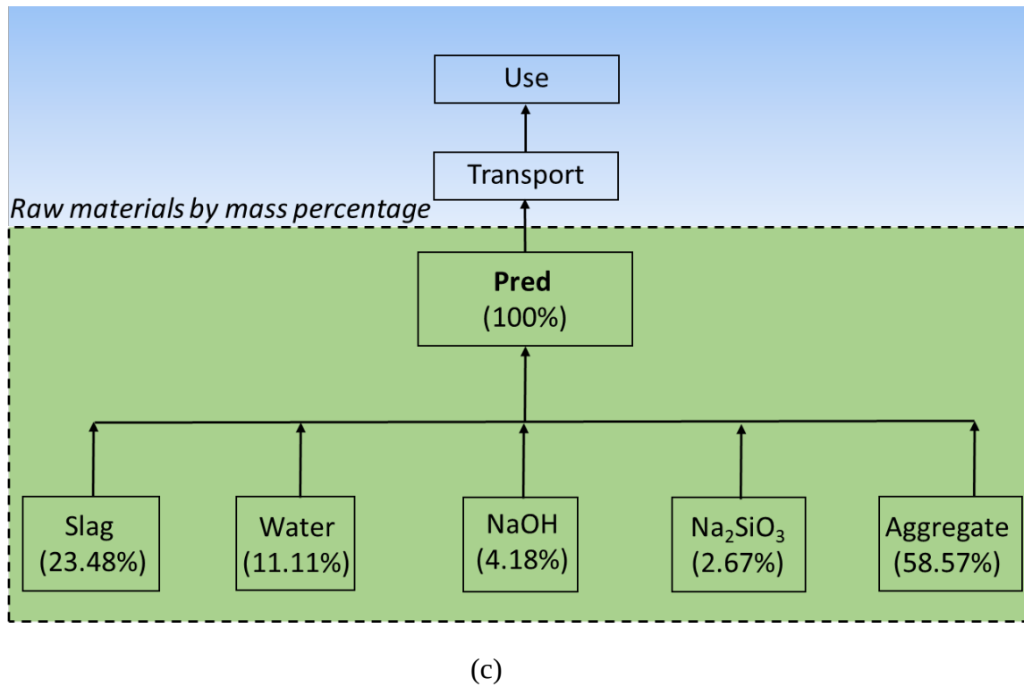
Fig. 6.9. Flow diagrams for production of (a) Conv, (b) Norm, and (c) Pred.
