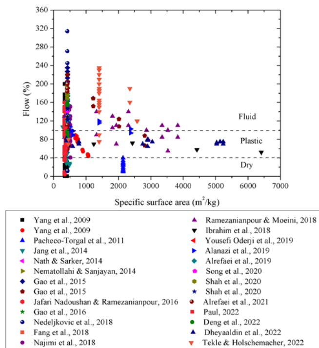
Fig. 3.3. Effect of specific surface area of precursor on workability
