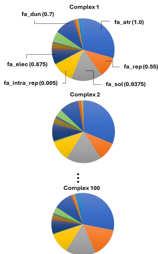
Figure 6: Parametric Contributions to the Total Energy Score in Rosetta Scoring.
