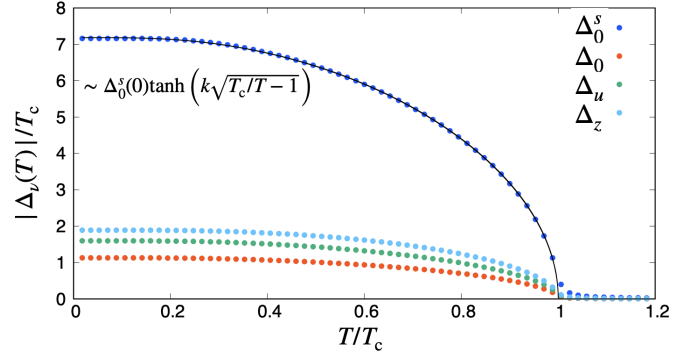
FIG. 1. Temperature dependence of the pair potential in the polar system. The black solid line shows the fitting line of \Delta_0^s(T) by \Delta_0^s(0) \tanh(k\sqrt{T_c/T - 1}) with the fitting parameter k . The critical temperature is T_c \simeq 2.85 \times 10^{-3} .
