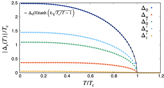
FIG. 3. Temperature dependence of pair potential in ferroaxial ordering. The black solid line shows the fitting line of \Delta_0(T) by \Delta_0(0)\tanh(k\sqrt{T_c/T-1}) . The critical temperature is T_c \simeq 6.55 \times 10^{-2} .
