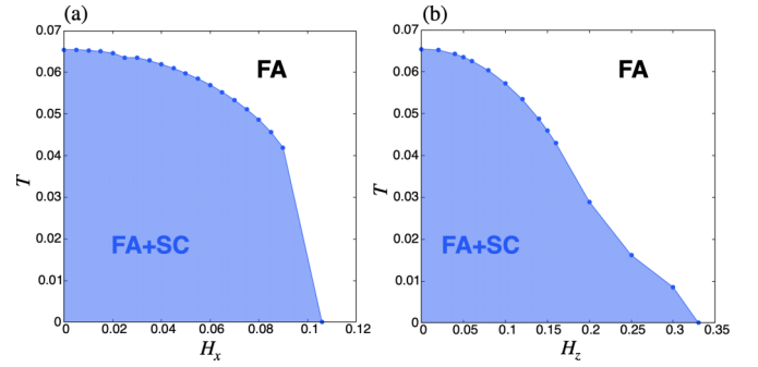
FIG. 4. SC phase diagrams under the ferroaxial (FA) molecular field. The panels (a) and (b) show the result for applied in-plane and perpendicular magnetic fields, respectively.
