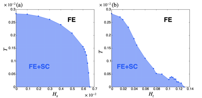
FIG. 2. SC phase diagrams under the ferroelectric (FE) molecular field. The panels (a) and (b) show the result for applied in-plane and perpendicular magnetic fields, respectively.
