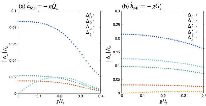
FIG. 5. The molecular field strength dependence of the amplitude of pair potentials for (a) the polar field and (b) the axial field with density n = 0.8 at zero temperature.
