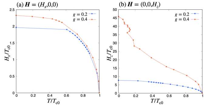
FIG. 6. The phase boundary (T_c, H_c) for (a) in-plane and (b) perpendicular magnetic field under the polar molecular field at n = 0.8 . T_{c0} is the critical temperature without the magnetic field.
