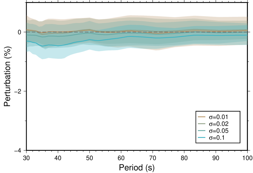
Figure 3.15: Same as Fig. 3.14 but for Love wave.
