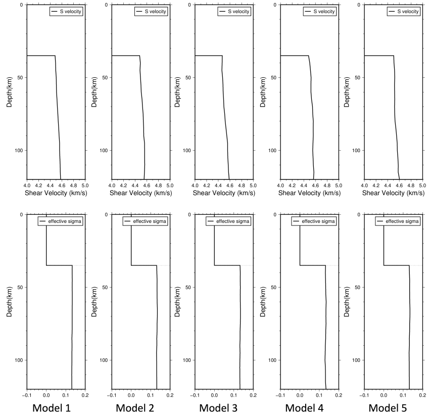
Figure 3.11: Vertically-smoothed average 1-D S-wave models and effective velocity fluctuations \sigma_{eff} for 5 random models used in Fig. 3.10 with different random seeds. Top: average 1-D S-wave model calculated from 1-D vertical profiles at various locations. Bottom: corresponding \sigma_{eff} for the heterogeneity in the depth range of 35–120 km.
