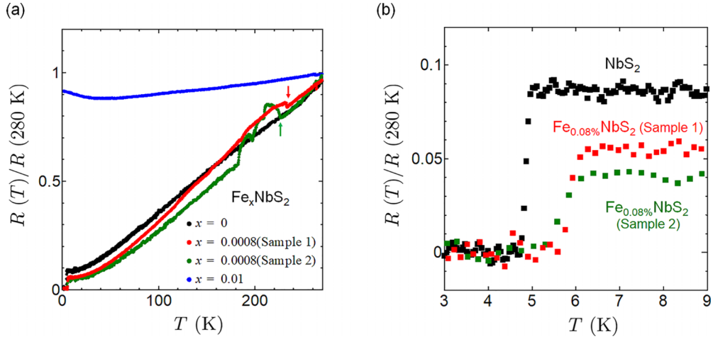
FIG. 1. Electric transport properties in \text{Fe}_x\text{NbS}_2 . (a) Temperature dependence of normalized resistance R(T)/R(280\text{ K}) for pure ( x=0 ), \text{Fe}_{0.08\%}\text{NbS}_2 , and \text{Fe}_{1\%}\text{NbS}_2 . (b) Enlargement of the dependence of normalized resistance R(T)/R(280\text{ K}) on temperature around T_c for \text{NbS}_2 and \text{Fe}_{0.08\%}\text{NbS}_2 .
