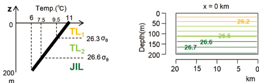
Fig. 8. (a) Horizontal distribution of sea level at steady state, simulated by a single-layer model that was forced by the inflow-outflow through the strait (Iino et al., 2009). (b) Plane and vertical views of the channel model with a shallow sill topography in the present study. (c) Vertical profile of temperature (left) and cross-sectional distribution of density (right), which was determined based on a typical stratification in spring, assumed as the initial condition throughout the model domain, and imposed on the western open boundary.
