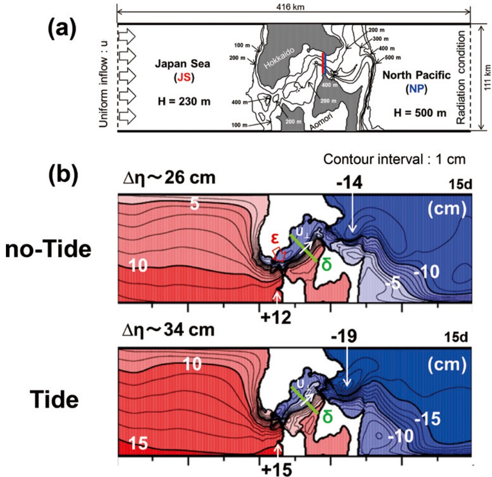
Fig. 17. (a) Model topography with real bathymetry around the Tsugaru Strait. The northern and southern boundaries were closed by artificial wall (solid line). A uniform inflow with a constant volume transport of Q is imposed on the western open boundary. (b) Horizontal distributions of sea level in Cases no-Tide (upper panel) and Tide (lower panel) at steady state.
