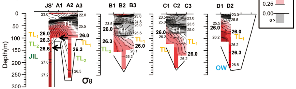
Fig. 6. Vertical distributions of potential density and AOU along the four observation lines from A to D in (a) April 2021 and (b) August 2022. Counter interval is 0.1 \sigma_\theta . Symbols to indicate a kind of water masses (TH, TL 1 , TL 2 , JIL, OW, and CO) are marked in the vicinity of the location where each water mass was observed.
