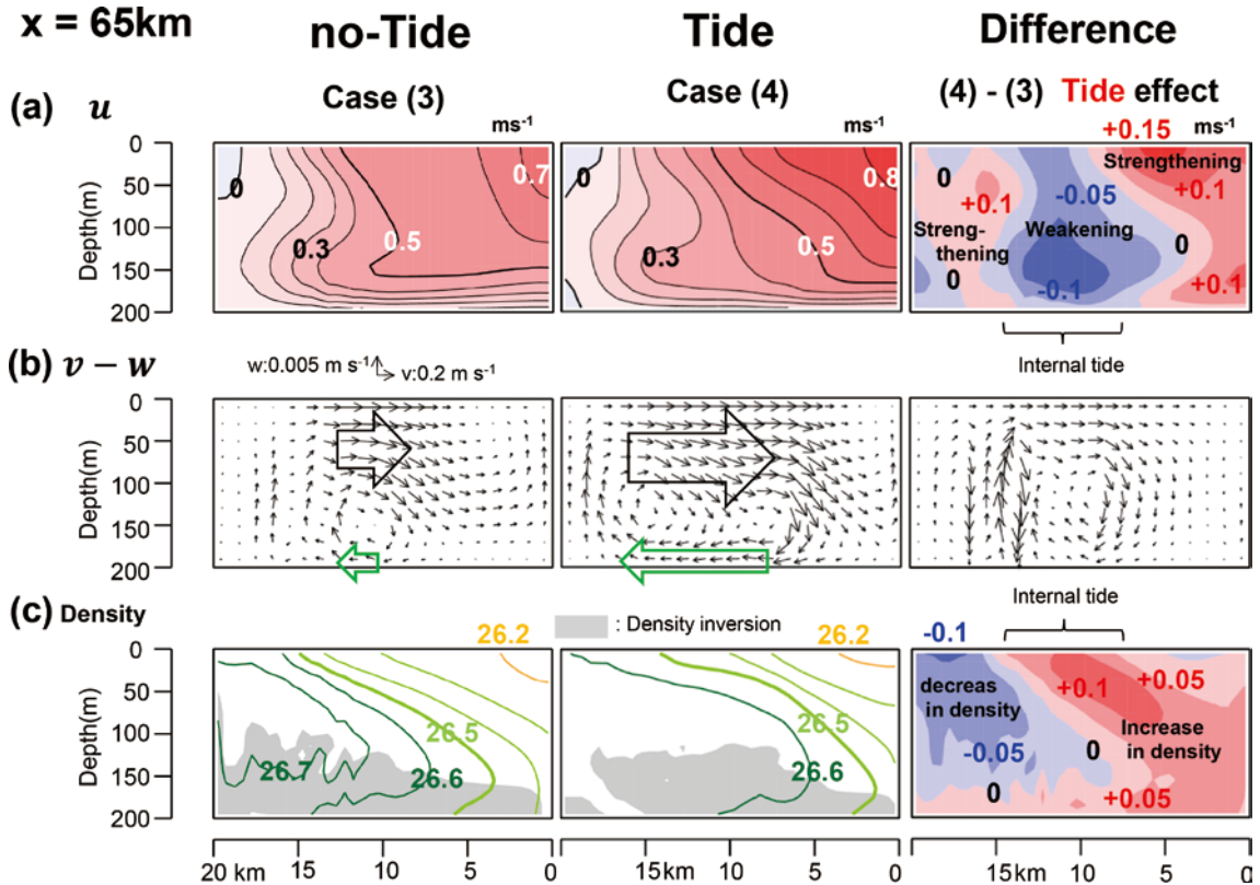
Fig. 16. Vertical section of (a) across-sectional velocity u , (b) velocity vectors parallel to the section v-w , and (c) potential density along x = 65 \text{ km} in Fig. 10. Three kinds of sections are displayed; Case no-Tide (left panel; Case (3)), Case Tide (middle panel; Case (4)), and their Difference (right panel).
