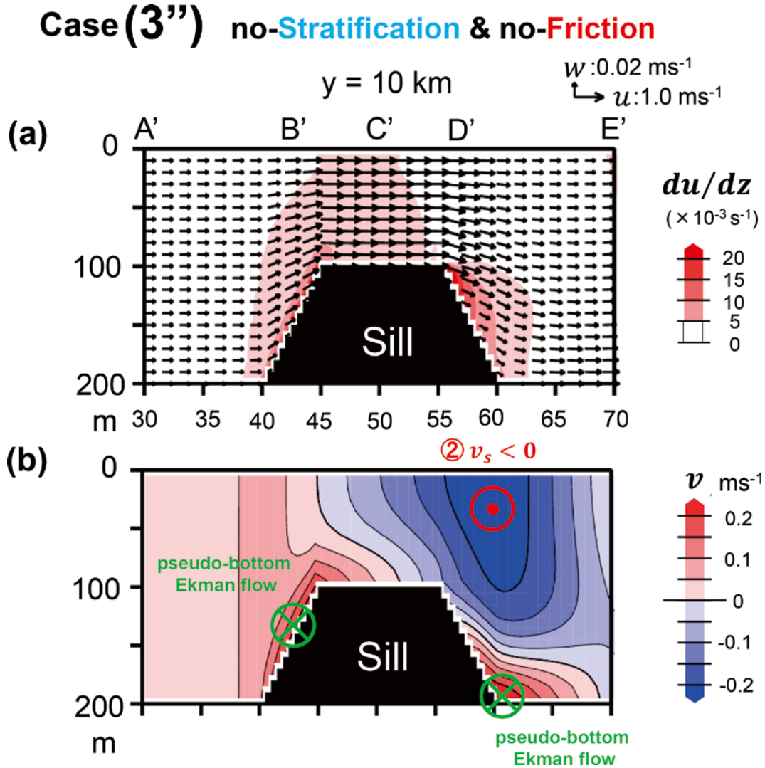
Fig. 12. Vertical section of (a) velocity vectors parallel to the section u-w , and (b) velocity component perpendicular to the section v from A' to E' lines of Case (3'') shown in Fig. 11(c). Pseudo-bottom Ekman flows (schematic green arrows in (b)) are trapped on the slopes on both sides of the sill.
