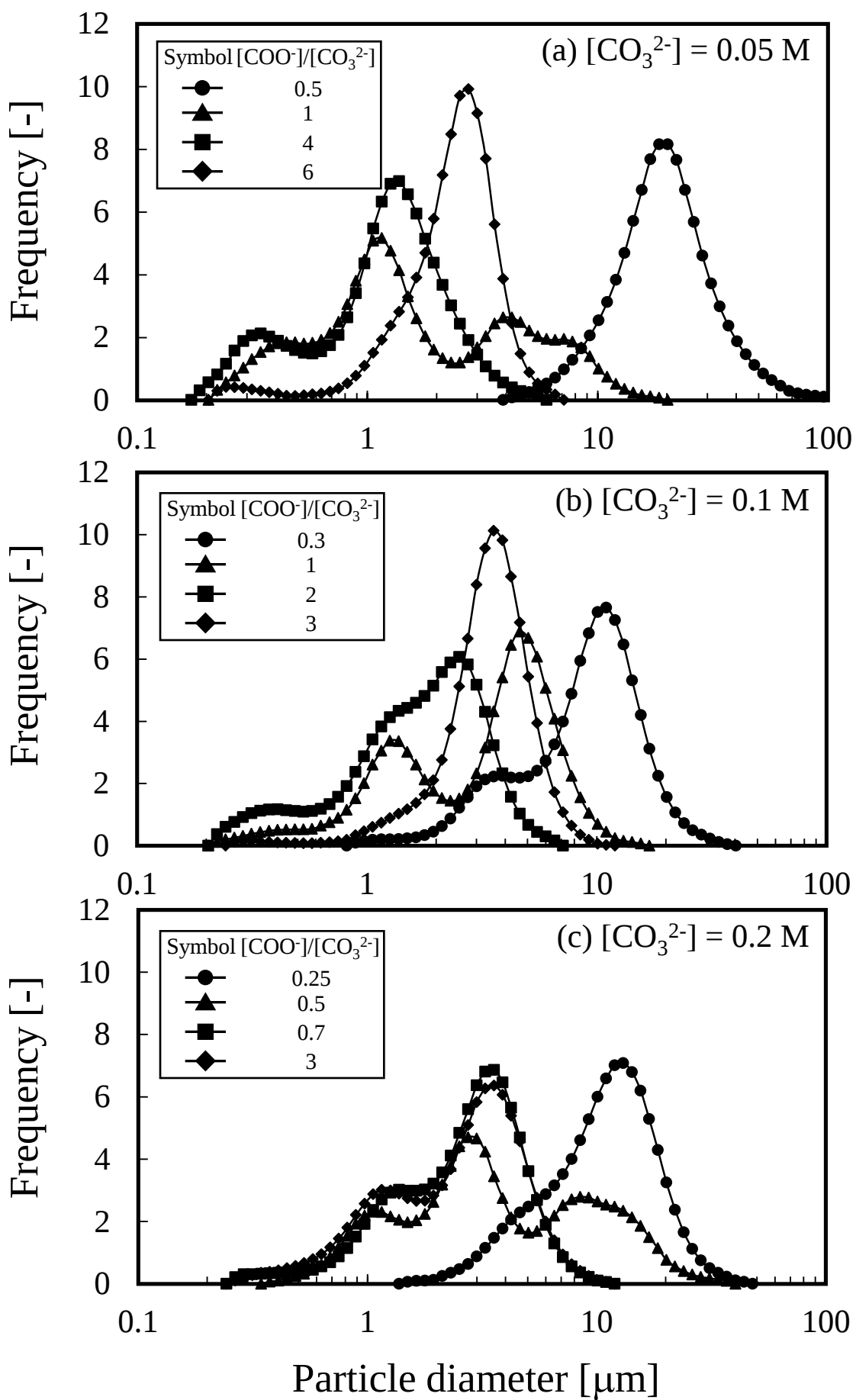
Fig. 1. Typical result of particle diameter distribution in the case of using the diluted CaCS solution with adding sodium oxalate as a bicarboxylate. In the case of (a) [\text{CO}_3^{2-}] = 0.05\text{M} , (b) [\text{CO}_3^{2-}] = 0.1\text{M} , and (c) [\text{CO}_3^{2-}] = 0.2\text{M} , \text{Na}_2\text{CO}_3 was employed in the mixture solution.
