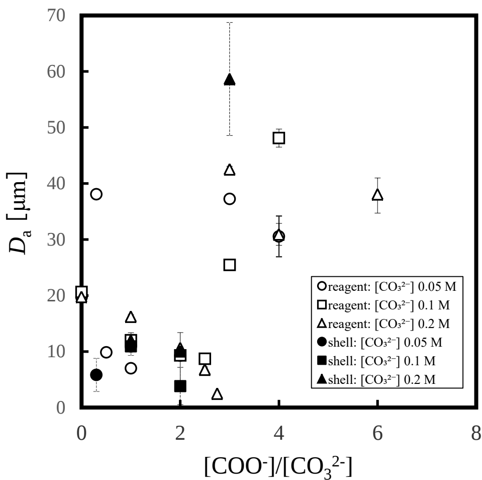
Fig. 4. Change in the average diameter of particles by addition of potassium hydrogen phthalate with varying the molar ratio of carboxyl group and carbonate ion, [\text{COO}^-]/[\text{CO}_3^{2-}] in the initial solution.
