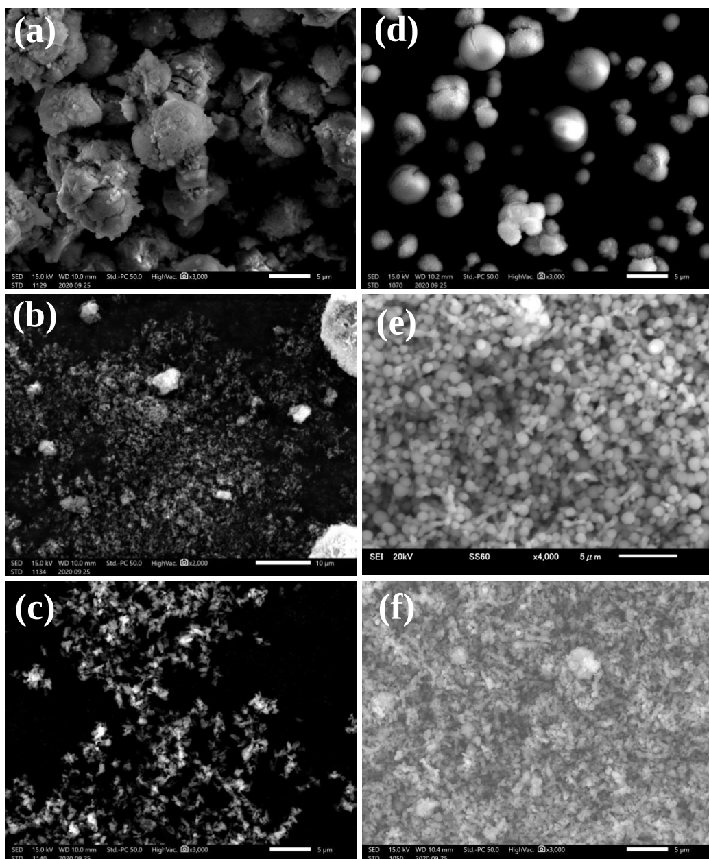
Fig. 12. SEM images of the particles generated by adding sodium oxalate (a, b, c) and sodium citrate (d, e, f). The experimental conditions: (a) [\text{CO}_3^{2-}] 0.1 M, molar ratio 0.3; (b) [\text{CO}_3^{2-}] 0.1 M, molar ratio 1; (c) [\text{CO}_3^{2-}] 0.1 M, molar ratio 2; (d) [\text{CO}_3^{2-}] 0.05 M, molar ratio 1.98; (e) [\text{CO}_3^{2-}] 0.1 M, molar ratio 3.98; (f) [\text{CO}_3^{2-}] 0.2 M, molar ratio 3.98.
