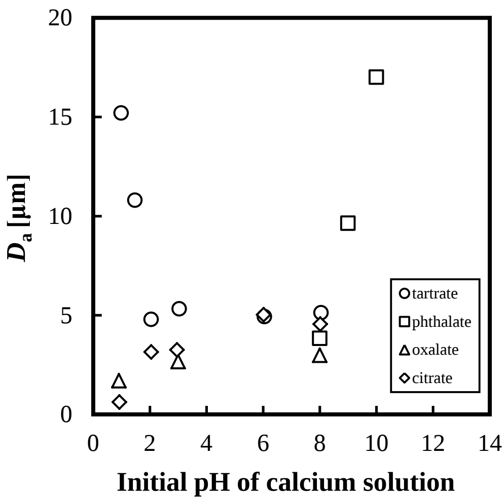
Fig. 2. Influence of the initial pH value on the average diameter, D_a , of particles.
