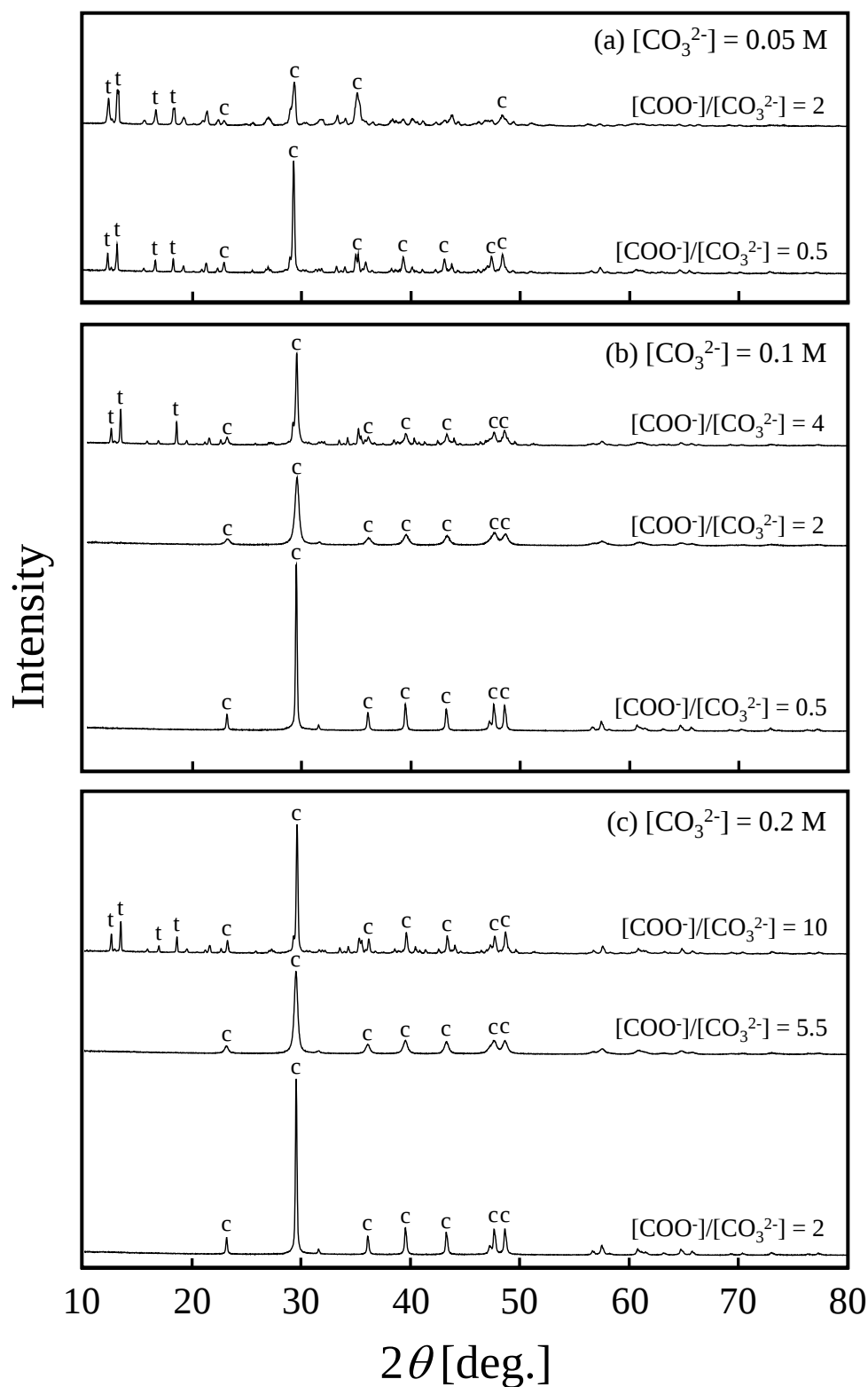
Fig. 7. XRD patterns of the particles generated with potassium sodium tartrate. The calcium solution was used CaSC solution. The characters correspond to calcite (c) and calcium tartrate tetrahydrate (t), respectively.
