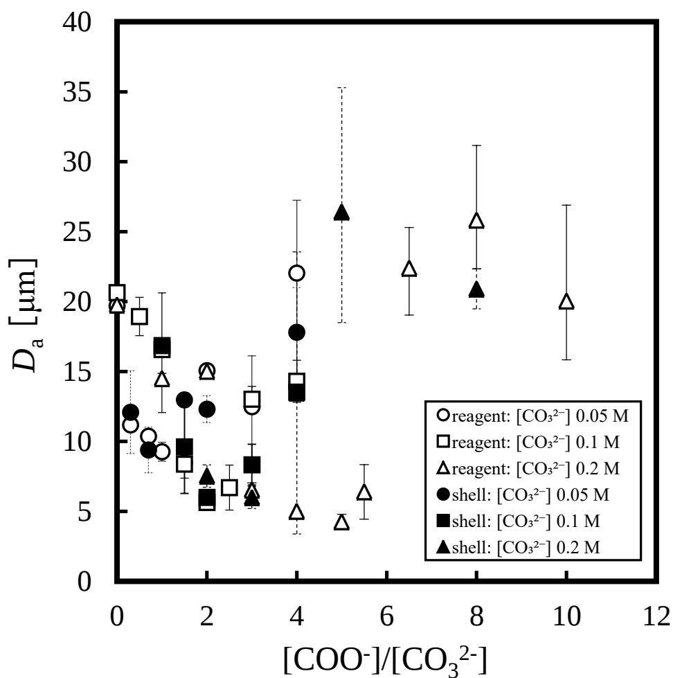
Fig. 3. Change in the average diameter of particles by addition of potassium sodium tartrate with varying the molar ratio of carboxyl group and carbonate ion, [\text{COO}^-]/[\text{CO}_3^{2-}] in the initial solution.
