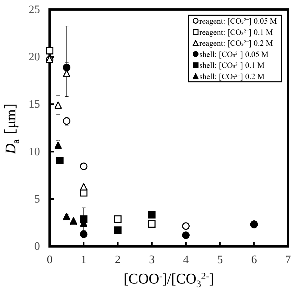
Fig. 5. Change in the average diameter of particles by addition of sodium oxalate with varying the molar ratio of carboxyl group and carbonate ion, [\text{COO}^-]/[\text{CO}_3^{2-}] in the initial solution.
