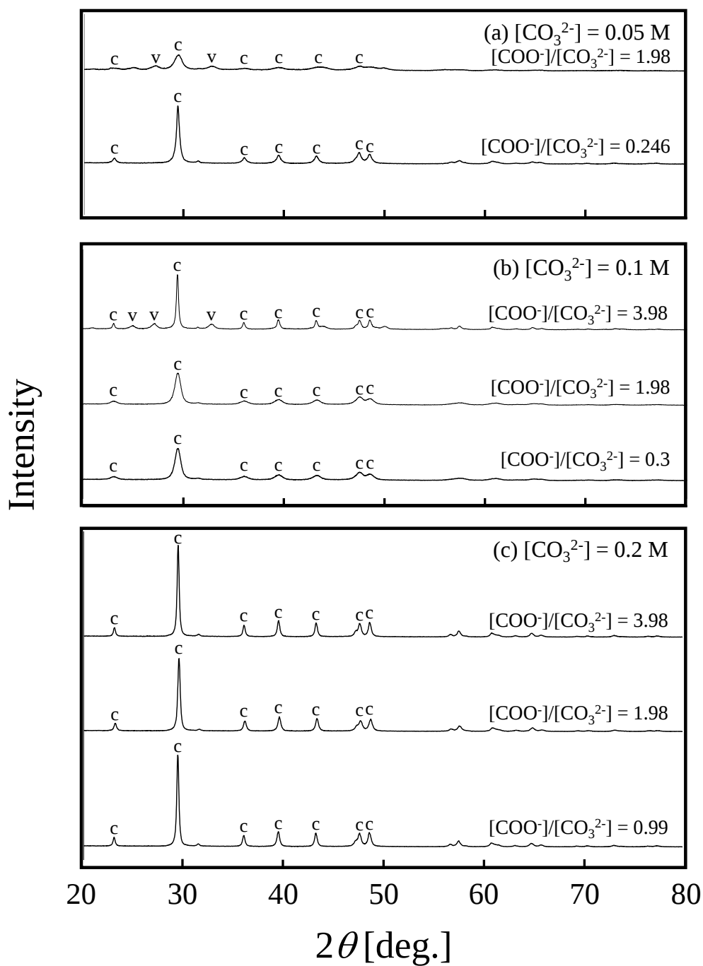
Fig. 10. XRD patterns of the particles generated with sodium citrate. The calcium solution was used CaSC solution. The characters correspond to calcite (c) and vaterite (v), respectively.
