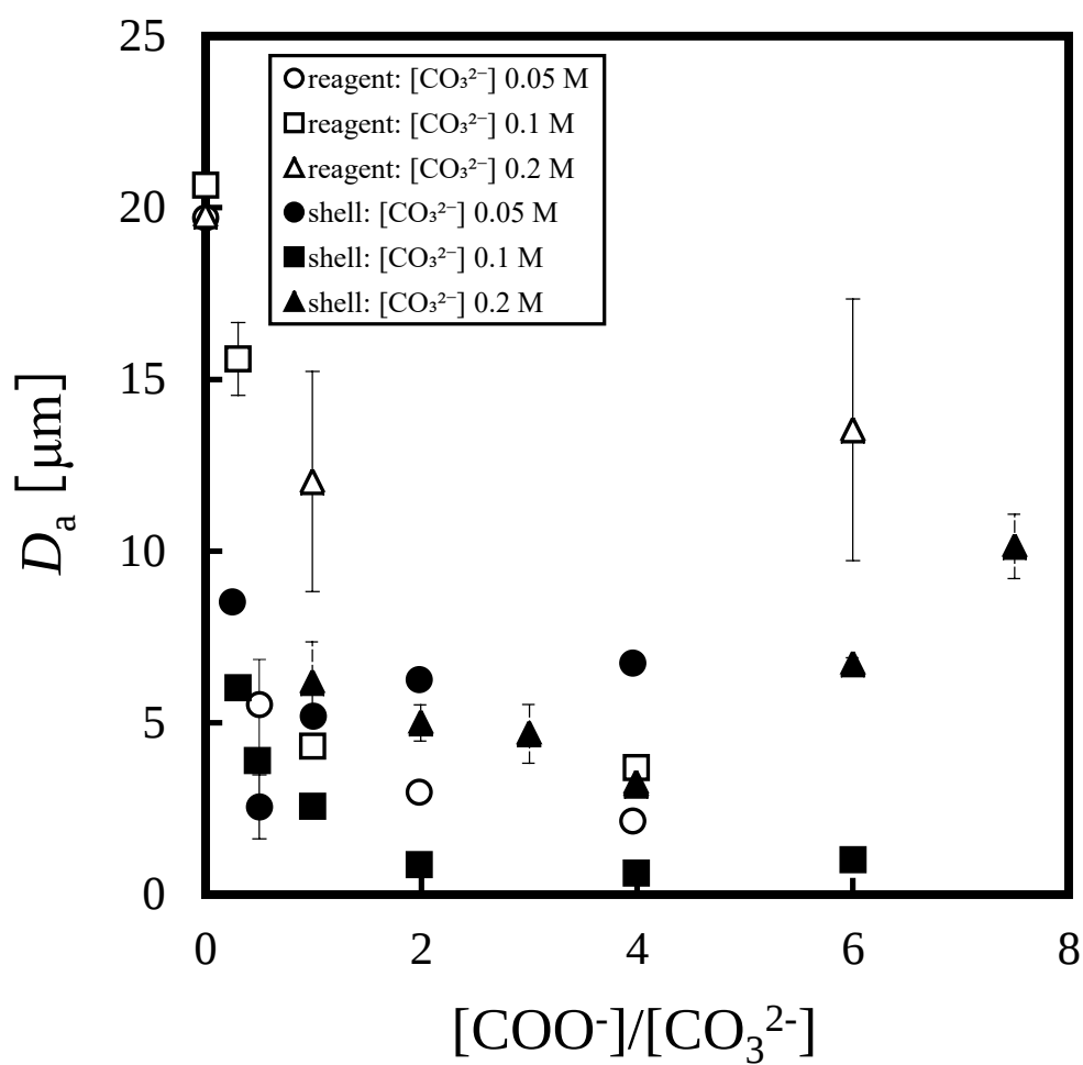
Fig. 6. Change in the average diameter of particles by addition of sodium citrate with varying the molar ratio of carboxyl group and carbonate ion, [\text{COO}^-]/[\text{CO}_3^{2-}] in the initial solution.
