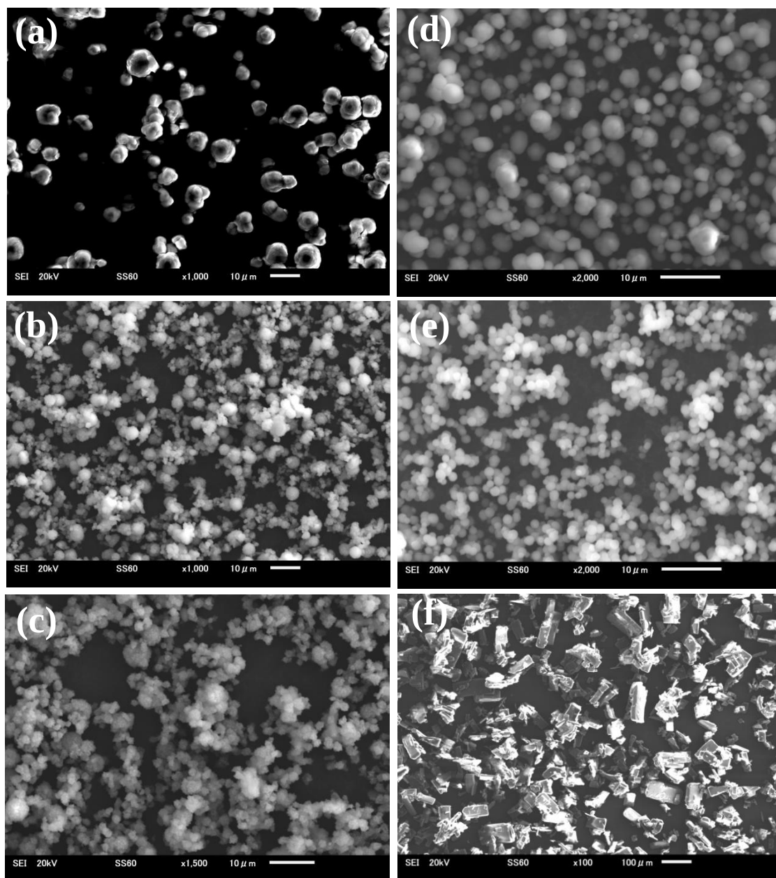
Fig. 11. SEM images of the particles generated by adding sodium tartrate (a, b, c) and potassium hydrogen phthalate (d, e, f). The experimental conditions: (a) [\text{CO}_3^{2-}] 0.05 M, molar ratio 0.3; (b) [\text{CO}_3^{2-}] 0.1 M, molar ratio 4; (c) [\text{CO}_3^{2-}] 0.2 M, molar ratio 5; (d) [\text{CO}_3^{2-}] 0.05 M, molar ratio 1; (e) [\text{CO}_3^{2-}] 0.2 M, molar ratio 2; (f) [\text{CO}_3^{2-}] 0.2 M, molar ratio 3.
