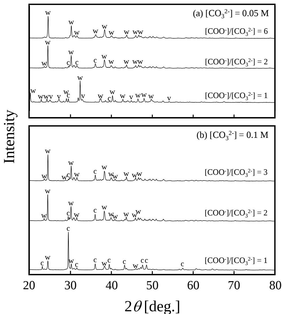
Fig. 9. XRD patterns of the particles generated with sodium oxalate. The calcium solution was used CaSC solution. The characters correspond to calcite (c), vaterite (v), and whewellite (w), respectively.
