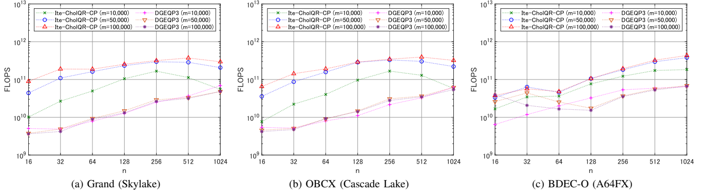
Fig. 5: Obtained FLOPS.
