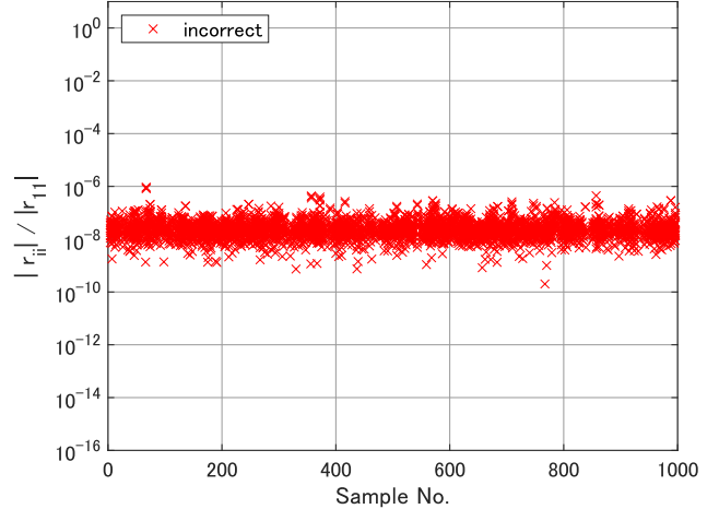
(c) Distribution of incorrect pivot selections
