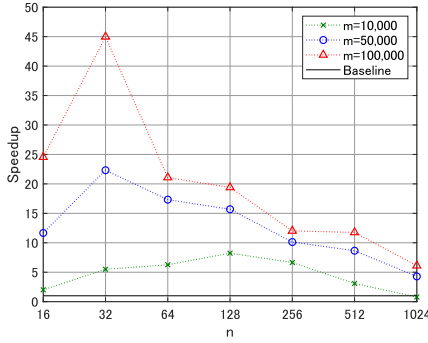
(a) Grand (Skylake)
