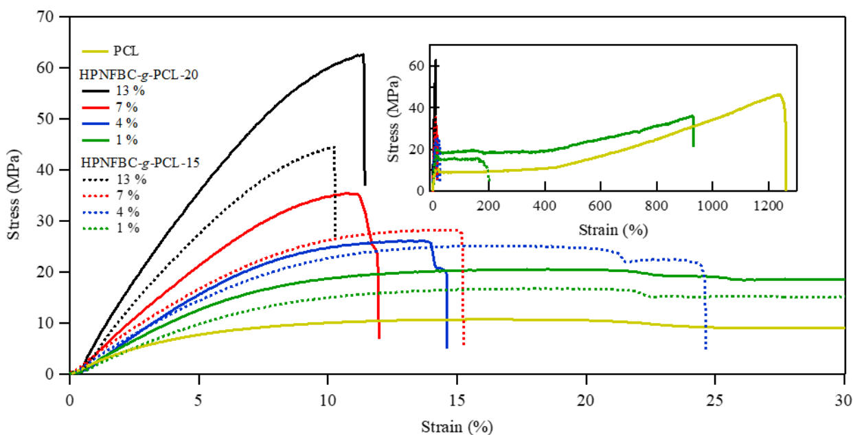
Figure 4. Stress-Strain curves of HPNFBC-g-PCL-20/PCL, HPNFBC-g-PCL-15/PCL nanocomposites with 13, 7, 4, and 1 wt.% cellulose and neat PCL.
