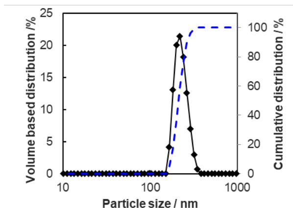
Fig. S1. Volume-based DLS profile of CNH-rTPA(1:1) in 10 mM HEPES solution of H 2 O. Histogram average value is 228 \pm 38 nm, and polydispersity index (PDI) is 0.053.
