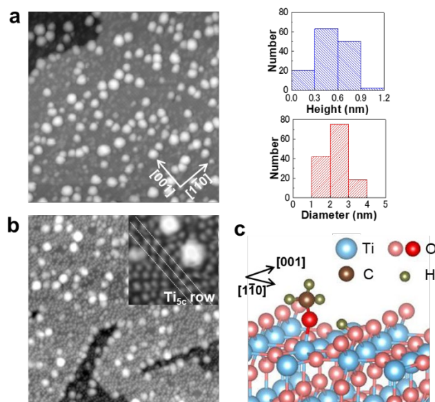
Figure 1. (a) STM image ( 50 \times 50 \text{ nm}^2 ) of a \text{Pt/TiO}_2(110) surface and histograms of the apparent height and diameter of the Pt nanoparticles. The \text{Pt/TiO}_2(110) surface was prepared by Pt deposition (0.11 ML) at room temperature, followed by annealing at 473 K for 10 min. The particle density was 5.4 \times 10^{16} / \text{m}^2 . (b) STM image ( 50 \times 50 \text{ nm}^2 ) of the \text{Pt/TiO}_2(110) surface after exposure to 5 L methanol vapor at room temperature. The inset is magnified image of another area ( 7.4 \times 7.4 \text{ nm}^2 ). The methoxy coverage was 0.14 ML. (c) Methoxy intermediate adsorbed on a \text{Ti}_{5c} site of a \text{TiO}_2(110) surface.
