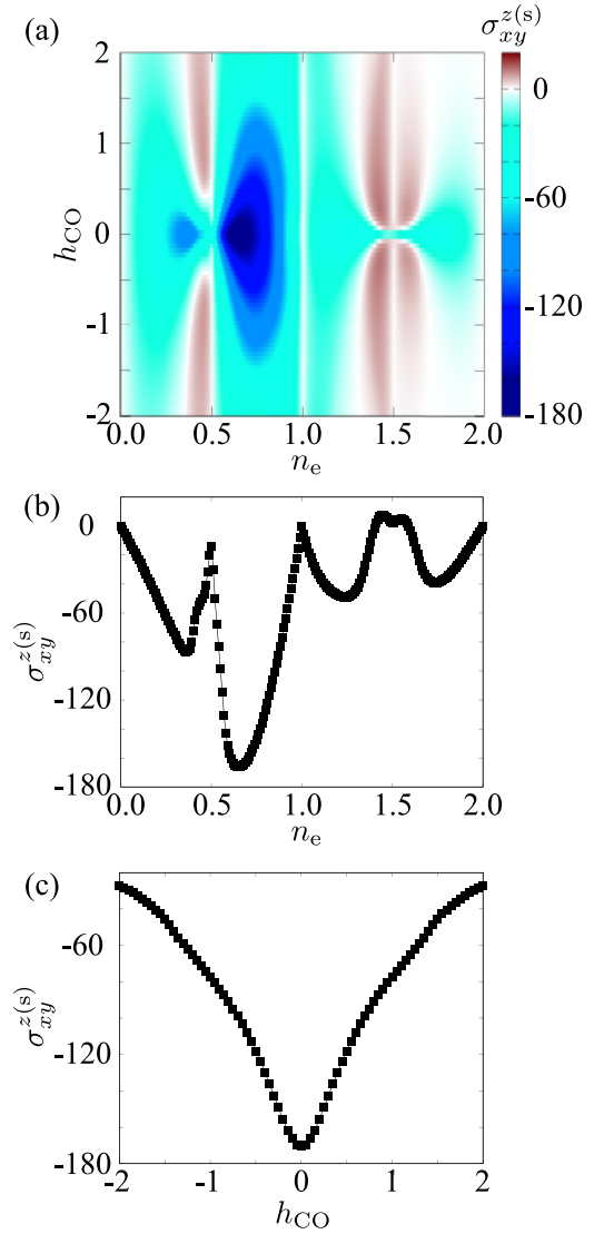
FIG. 3. (a) Contour plots of \sigma_{xy}^{z(s)} in the plane of n_e and h_{\text{CO}} at t_a = 1 , t_b = 0.9 , t'_a = 0.3 , t'_b = 0.27 , and h_{\text{AFM}} = 3 . It is noted that \sigma_{xy}^{z(s)} values are small but nonzero values in the white region for 0 < n_e < 2 owing to the interband process; see the text for details. (b) n_e dependence of \sigma_{xy}^{z(s)} at h_{\text{CO}} = 0.1 . (c) h_{\text{CO}} dependence of \sigma_{xy}^{z(s)} at n_e = 0.65 .
