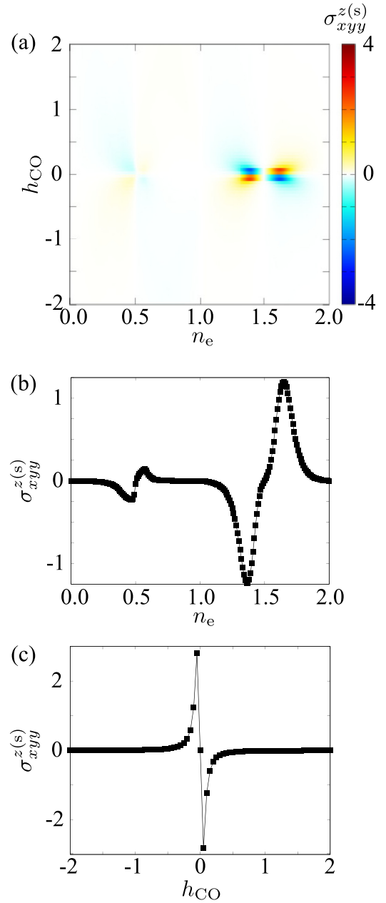
FIG. 4. (a) Contour plots of \sigma_{xyy}^{z(s)} in the plane of n_e and h_{CO} at t_a = 1 , t_b = 0.9 , t'_a = 0.3 , t'_b = 0.27 , and h_{AFM} = 3 . (b) n_e dependence of \sigma_{xyy}^{z(s)} at h_{CO} = 0.1 . (c) h_{CO} dependence of \sigma_{xyy}^{z(s)} at n_e = 1.36 .
