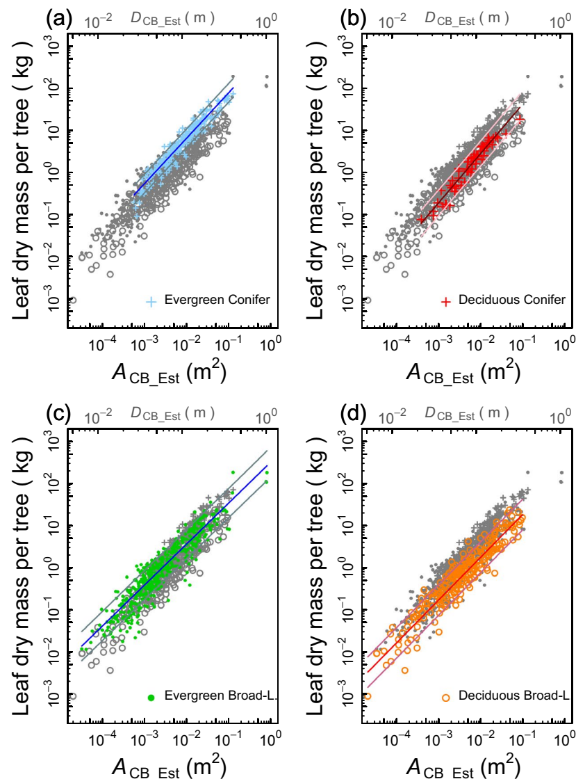
Figure 4. qPipe model allometries between A_{\text{CB\_Est}} and the leaf mass (LM) for (a) EC, (b) DC, (c) EB and (d) DB PFTs. The allometry obtained using the GLMM was selected in (a), (c), and (d), where species were designated as the random effect for the elevation of the regression line. For (b), an ordinary linear regression model pooling all species data was selected. See Table 1 for coefficients of each allometric equation, Table 2 for the coefficients of the equation approximating the 95% prediction intervals, and Supplementary Information S1 and S2 for the method of determining/approximating the prediction interval equations.
