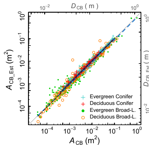
Figure 1. Relationship between A_{CB} and A_{CB\_Est} obtained using SMA regression. PFTs are included as the categorical variable of an SMA regression equation, and their elevation (values of A_{CB\_Est} at A_{CB} = 1 \text{ m}^2 ) and slope are given in Table 1. Regression lines are drawn between horizontal data ranges of respective PFTs, where the blue solid line is for the EC PFT, the black solid line for the DC PFT, blue dashed line for the EB PFT, and black dashed line for the DB PFT. D_{CB} and D_{CB\_Est} indicate scales of diameter converted from A_{CB} and A_{CB\_Est} , respectively.
