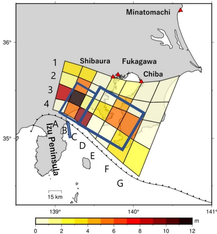
Figure S1 The best fault model of the Kanto earthquake by Aida (1993), three blue rectangles. The slip distribution estimated in this study is also shown by colored quadrilaterals.
