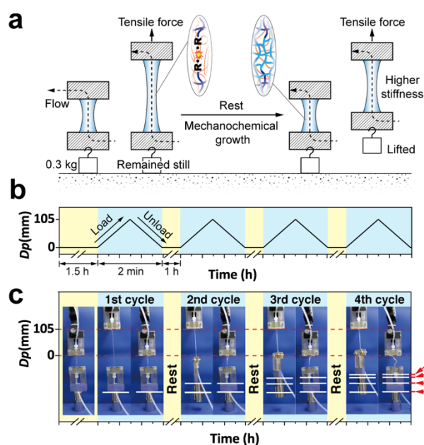
Fig. 4 Muscle-like behaviours of the c-DN hydrogel under repeated mechanical deformations. (a) Illustration of the training process of the c-DN hydrogel by mechanochemical growth. The upper jig is fixed to the tensile tester and repeatedly lifted up to a displacement of 105 mm, the lower jig is connected to a weight (0.3 kg). After the “training” sustained independently by the vascular perfusion, the c-DN hydrogel is able to lift up the weight. (b) Protocol of the upper crosshead displacement during the cyclic deformation of the c-DN gel (gauge length = 15 mm). (c) Demonstrations of the muscle-like behaviours of a c-DN hydrogel supplied by 0.10 M NaAMPS monomer and 0.10 M MBAA crosslinker ( M_{0.10}C_{0.10} ) showing repetitive stretch-triggered mechanical growth.
