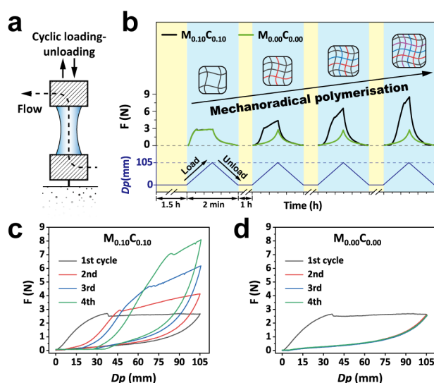
Fig. 5 Stretch-triggered repetitive self-growth of c-DN gel by continuous monomer supply from the internal channel. (a) Illustration of the cyclic loading–unloading setup. (b) Force–time curves of M_{0.10}C_{0.10} under a repeated tensile force trigger shown in the loading–unloading protocol underneath: the upper crosshead displacement ( Dp ) is lifted up to 105 mm and then returned to the original position ( Dp = 0 mm) during the cyclic deformation of the c-DN gel (gauge length = 15 mm). The gel shows a noticeable strengthening due to repeated network deconstruction–reconstruction. M_{0.00}C_{0.00} implies the flow of pure water as a reference, which indicates no self-growth without monomers supply from the channel. Samples are coded by the concentrations of monomer and cross-linker in the flowing solution as M_aC_b , where “a” stands for the monomer (NaAMPS) concentration and “b” the cross-linker (MBAA) concentration (all in mol/L). (c, d) Force–displacement curves of the M_{0.10}C_{0.10} (c), and M_{0.00}C_{0.00} (d) samples, respectively, under four times of repeated tensile force trigger as shown in the lower panel in ‘b’.
