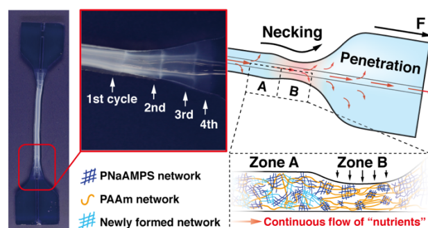
Fig. 6 Appearance of M_{0.10}C_{0.10} sample after four times of self-growth and the illustration of the unevenly distributed structure which caused the whitening phenomenon. As the gauge region yielded by stretch, it became stiffer by self-strengthening. Therefore, the relatively “weaker part” outside the yielded zone starts to yield in the next stretch. Thus, translucent “scars” of “training” that distinctly indicates the occurrence of four times of self-strengthening were left.
