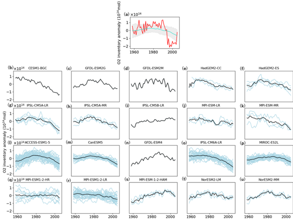
Figure 2. Anomalies in the O 2 inventory from the surface to depths of 1000 m in the North Pacific from 1958 to 2005. In panel (a), the red and cyan lines indicate observed and MMEM inventories, respectively, whereas the shaded area indicates the range between the 95 and 5 percentiles among model ensembles for each year. In panel (b) to (u), the light blue lines represent the ensemble members, respectively and the black line is the ensemble mean.
