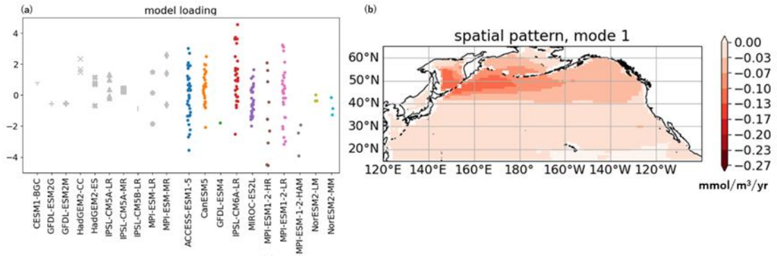
Figure 7. (a) Loading of the first EOF mode of the vertical averaged O 2 concentration trend from 1958 to 2005 in model ensembles, (b) spatial distribution of the first mode. The color bar in (b) shows a different range from the color bars in Figures 3 and 6. In (a), symbols are the same as Figure 4.
