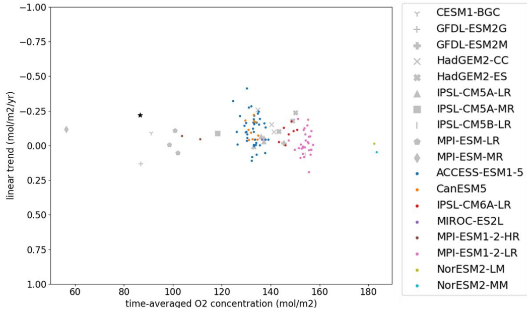
Figure 12. The scatter plot of the trend of vertically integrated O 2 concentration against the time-averaged vertically integrated O 2 concentration at Station P. Symbols are the same as Figure 4. Star symbol shows the observation.
