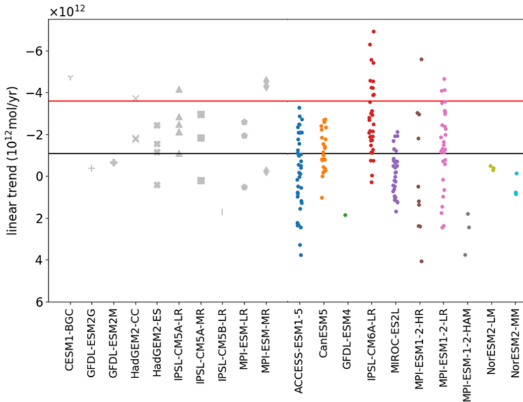
Figure 4. Trends of O 2 inventory anomalies from 1958 to 2005 in the North Pacific from the surface to depths of 1000 m, with negative trends represented by upward bars. The red line shows the observational trend, and the black line shows the MMEM trend. Gray symbols represent the CMIP5 models and colored symbols represent the CMIP6 models.
