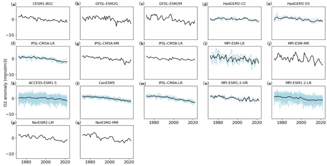
Figure 14. Area-averaged O 2 concentration anomalies at depths from the surface to 1000 m between 15°N and 34°N of the 137°E line. The light blue lines represent the ensemble members, respectively and the black line is the ensemble mean.
