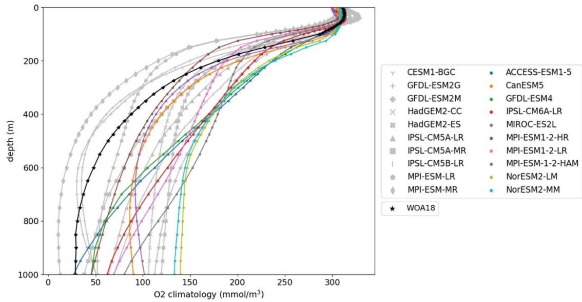
Figure 1. Vertical profile of regionally averaged O 2 climatology in the subarctic region (40° to 65°N). Gray symbols represent the CMIP5 models and colored symbols represent the CMIP6 models. The black line shows the climatology based on the World Ocean Atlas 2018 (WOA18).
