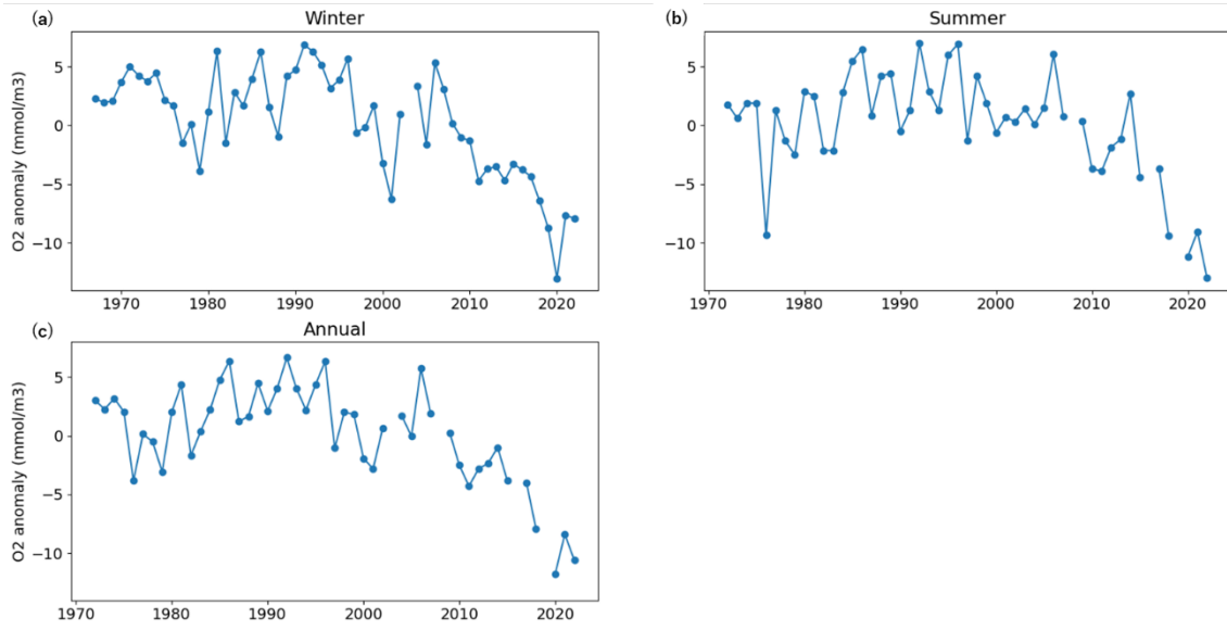
Figure 13. Area-averaged O 2 concentration anomalies at depths from the surface to 1000 m between 15°N and 34°N of the 137°E line. (a) Winter data is from 1967 to 2022, (b) summer data is from 1972 to 2022, and therefore, the annual average (c) is calculated from 1972 to 2022, when both winter and summer data are available. The anomalies for all seasons are based on the average value from 1972 to 2022.
