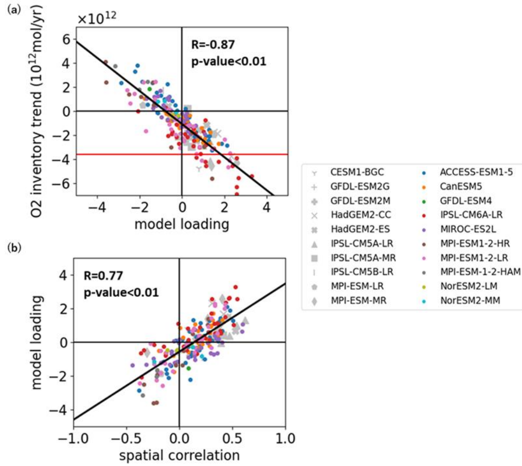
Figure 8. Scatter plots of the model loadings of the first EOF mode of the spatially distributed O2 trend and (a) the O2 inventory trend and (b) spatial correlation between the observation and each model ensemble member. The red line shows the observational trend. Gray symbols represent the CMIP5 models and colored symbols represent the CMIP6 models. Symbols are the same as Figures 4 and 7a.
