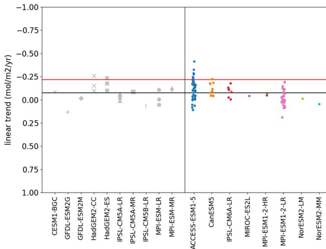
Figure 11. The trend of vertically integrated O 2 concentration at Station P. The red line shows the observational trend, and the black line shows the MMEM trend. Symbols are the same as Figure 4.
