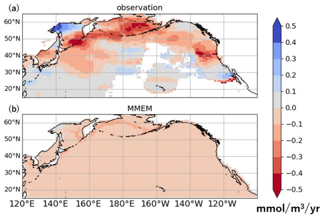
Figure 3. Vertical averages of O 2 concentration trend from 1958 to 2005 in (a) observations, and (b) MMEM.
