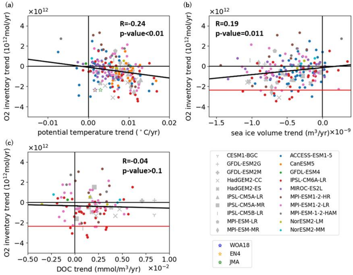
Figure 9. Scatter plots of the O 2 inventory trend in the subarctic North Pacific and (a) potential temperature trend, (b) sea ice volume trend, and (c) DOC trend averaged in the subarctic North Pacific (40° to 65°N). Symbols are the same as Figure 8. Star symbols in (a) show the trends of the observations. The red line in (b) and (c) shows the observational trend.
