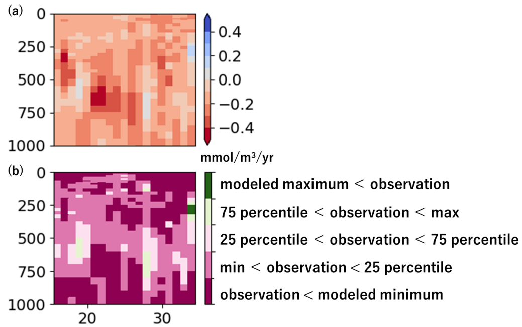
Figure 15. (a) Observed annual O 2 concentration trend from 1972 to 2022 of the 137°E line, and (b) a cross-sectional figure showing the position of the observed trends within the range of model trend variations for each grid. The vertical axis represents isobath depth (m) and the horizontal axis represents latitude from 15° to 34°N.
