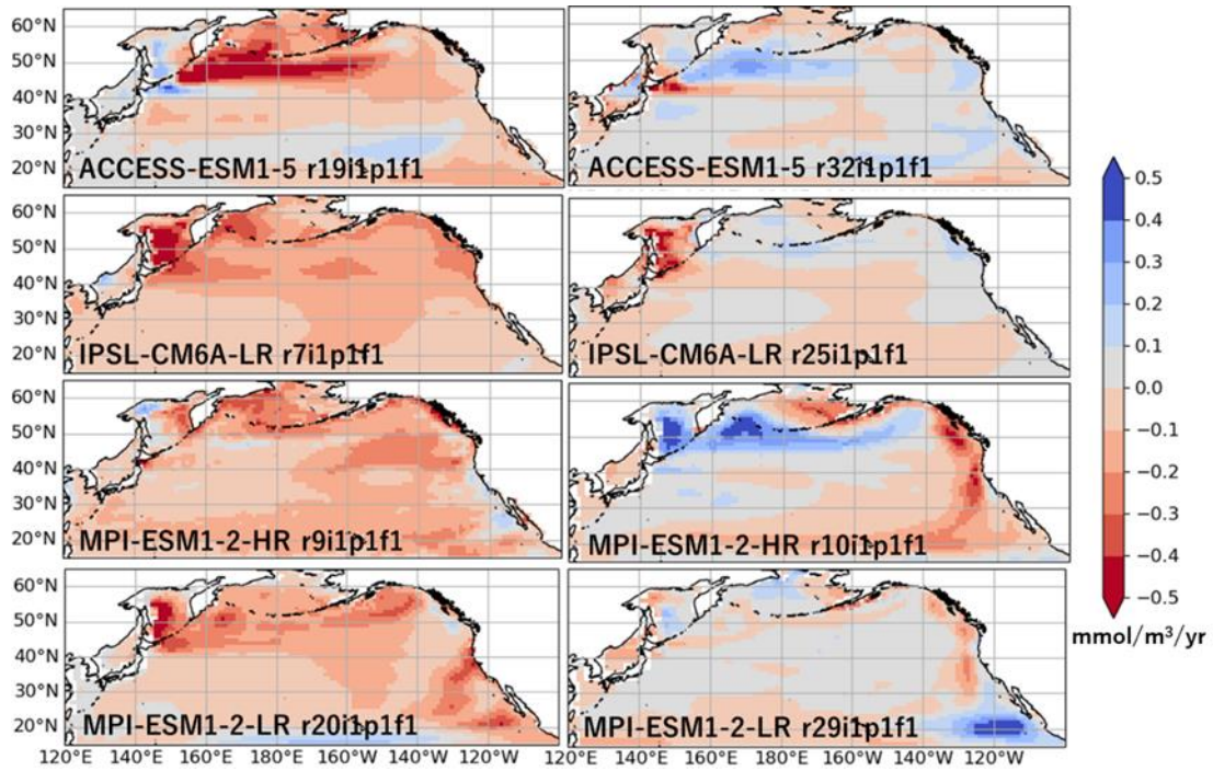
Figure 6. Vertical averages of O 2 concentration trends from 1958 to 2005 in the top four models known for their large variability in O 2 inventory trend (as shown in Figure 4). The left panels are the ensemble members characterized by the largest negative O 2 inventory trend, while the right panels exhibit the ensemble member with the largest positive O 2 inventory trend.
