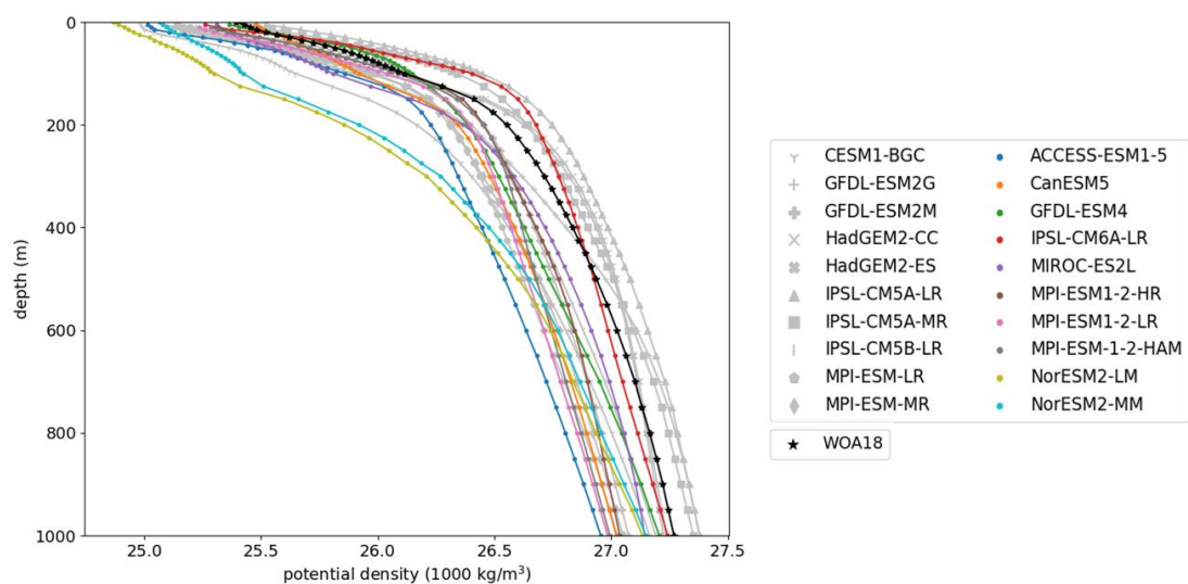
Figure 16. Vertical profile of regionally averaged potential density in the subarctic region (40° to 65°N). Symbols are the same as Figure 1.
