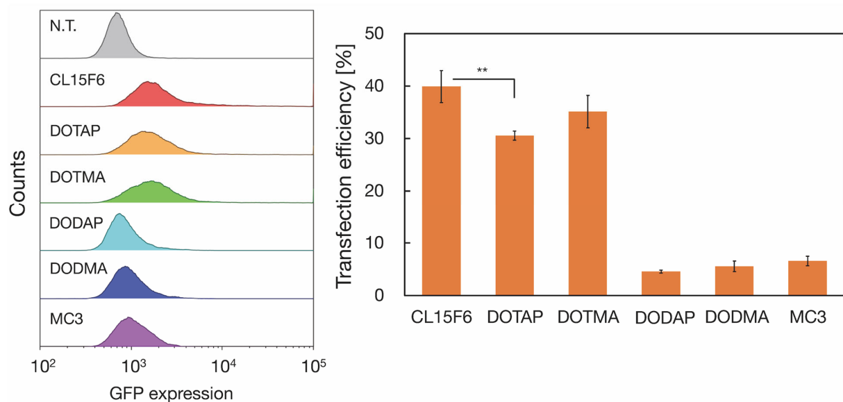
Fig. 7. Comparison of the transfection efficiency of the six types of LNP-polymer hybrid nanoparticles. (Left) GFP expression determined by flow cytometry. (Right) Average transfection efficiencies of each LNP. Ionizable lipids: CL15F6, DODAP, DODMA, and MC3; Cationic lipids:
