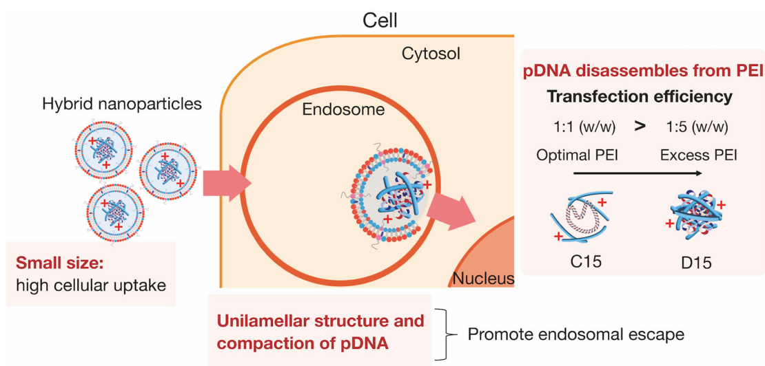
Fig. 8. Proposed mechanism illustrating the effective transfection of large-sized pDNA facilitated by lipid-polymer hybrid nanoparticles. Compaction of pDNA with PEI coupled with a unilamellar structure and a cationic nanoparticle charge can accelerate the endosomal escape of large-sized pDNA.
