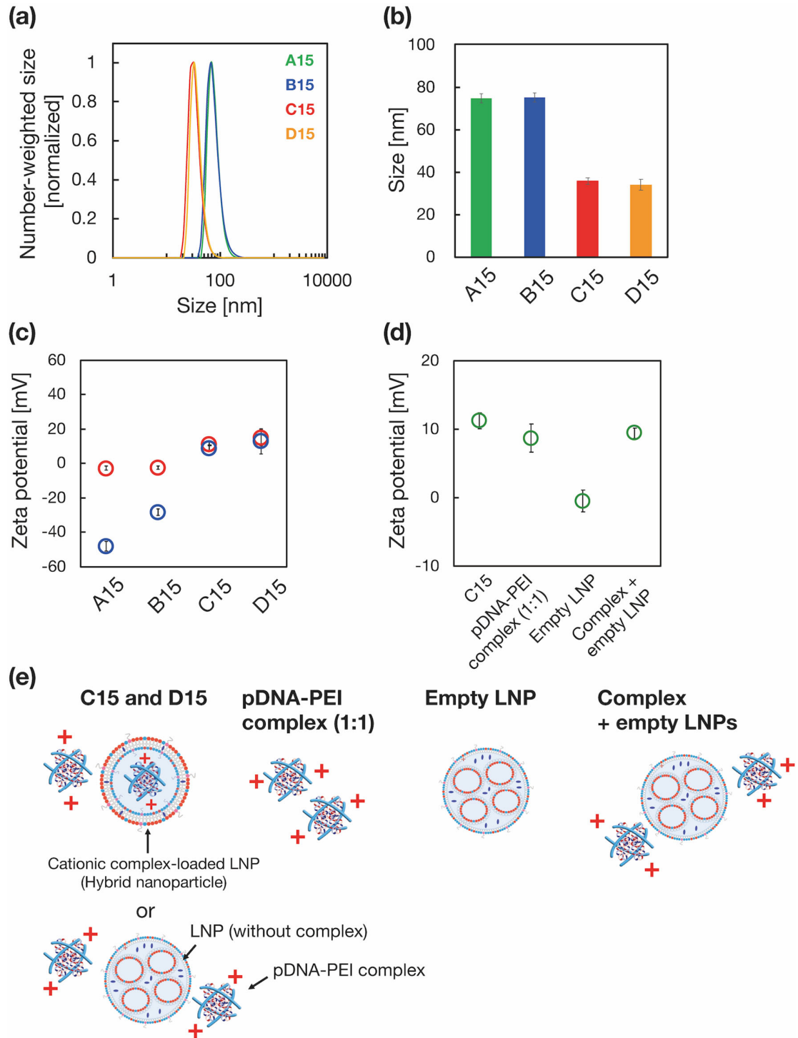
Fig. 2. Characterization of 15 kbp pDNA-PEI complex-loaded LNP with CL15F6 as the ionizable lipid. (a) Size distributions and (b) average sizes of 15 kbp pDNA-PEI complex-loaded LNP. CL15F6 was used as an ionizable lipid. The mass ratios of pDNA to PEI were 1:0, 1:0.1, 1:1, and
