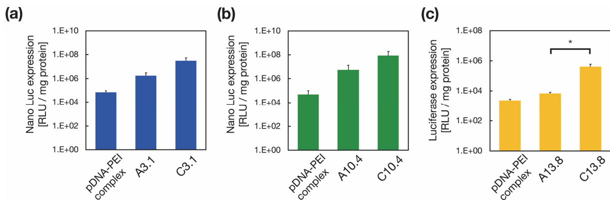
Fig. 5. Comparison of transfection efficiencies using three types of particles: pDNA-PEI complex, pDNA-loaded LNPs (A-LNP), and LNPs loaded with pDNA-PEI complex (1:1, C-LNP) using 3.1 kbp (blue), 10.4 kbp (green), and 13.8 kbp (yellow) pDNAs. Data are presented as the mean \pm SD ( n = 3 ). *: P < 0.05 . N.S.: not significant.
