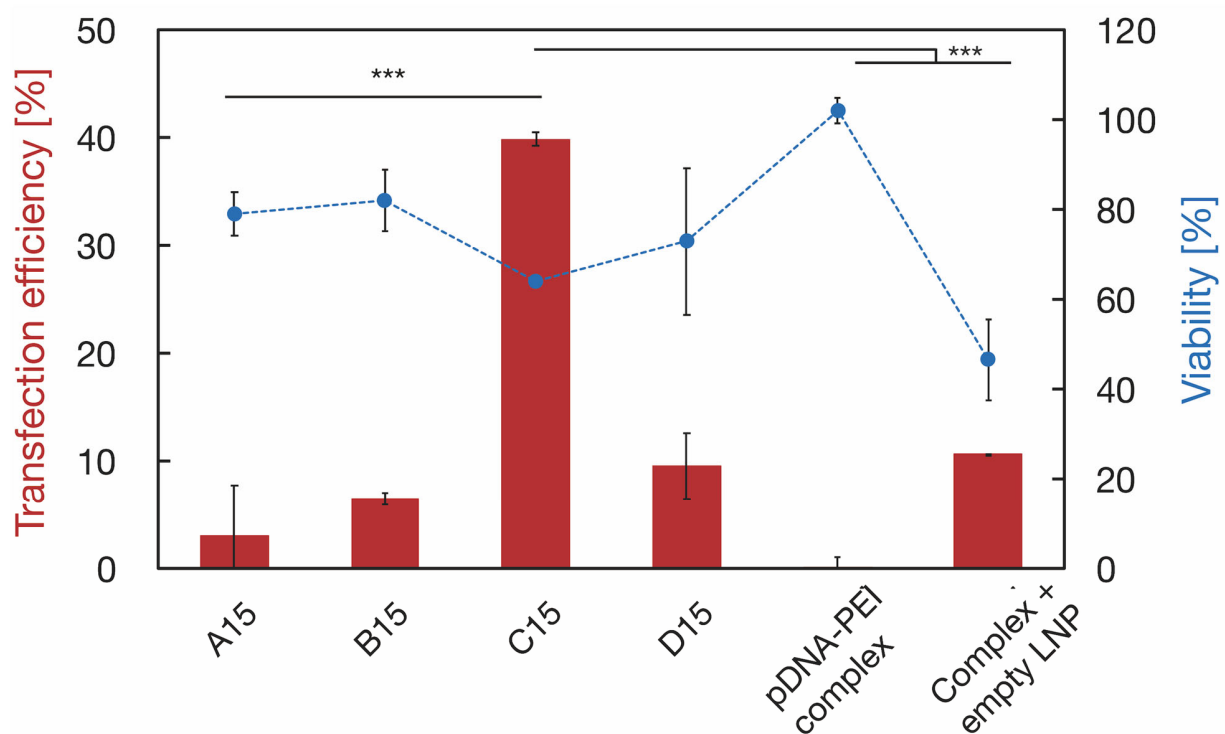
Fig. 4. Transfection efficiencies (bar chart) and cell viability (plots) of each LNP. Data are presented as the mean \pm SD (n = 3). ***: P < 0.001 (for transfection efficiency).
