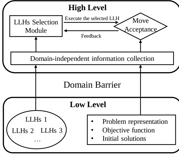
Fig. 1 A general structure of the HHs framework[19, 20].
