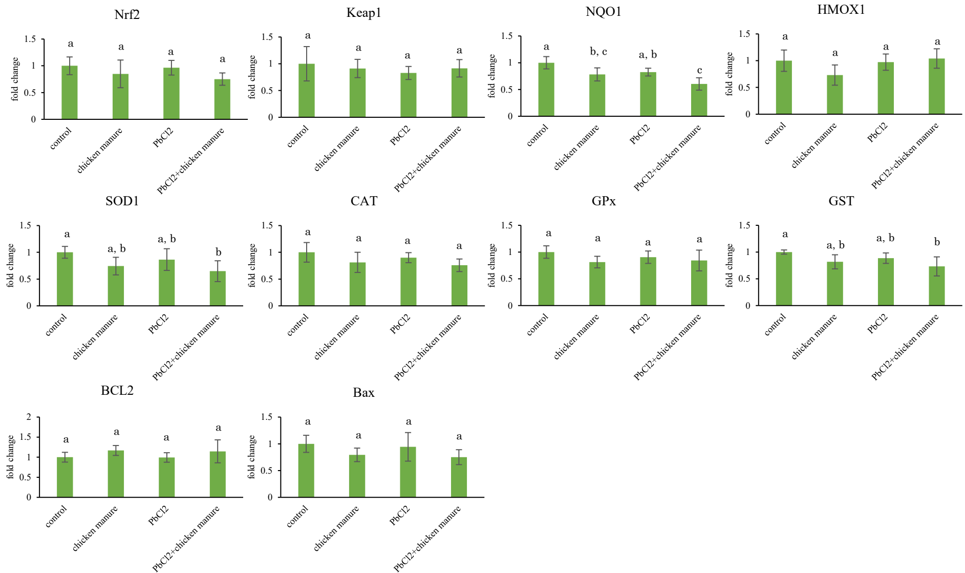
502 Figure 5. Expression of antioxidant enzymes and apoptosis related genes in the kidney at 98 days exposure (n=6) at p<0.05. Different letter symbols 503 among groups denote significant difference.
