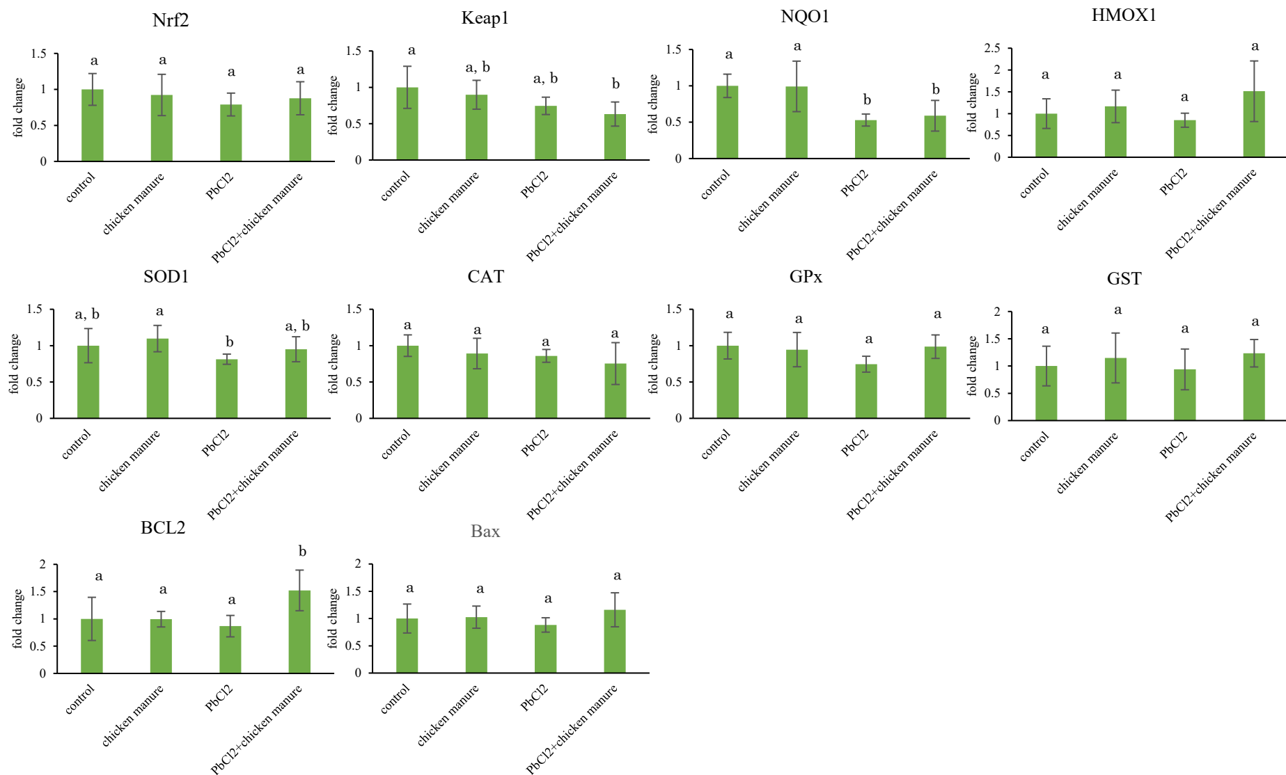
498 Figure 3. Expression of antioxidant enzymes and apoptosis related genes in the liver at 98 days exposure (n=6) at p<0.05. Different letter symbols 499 among groups denote significant difference.
