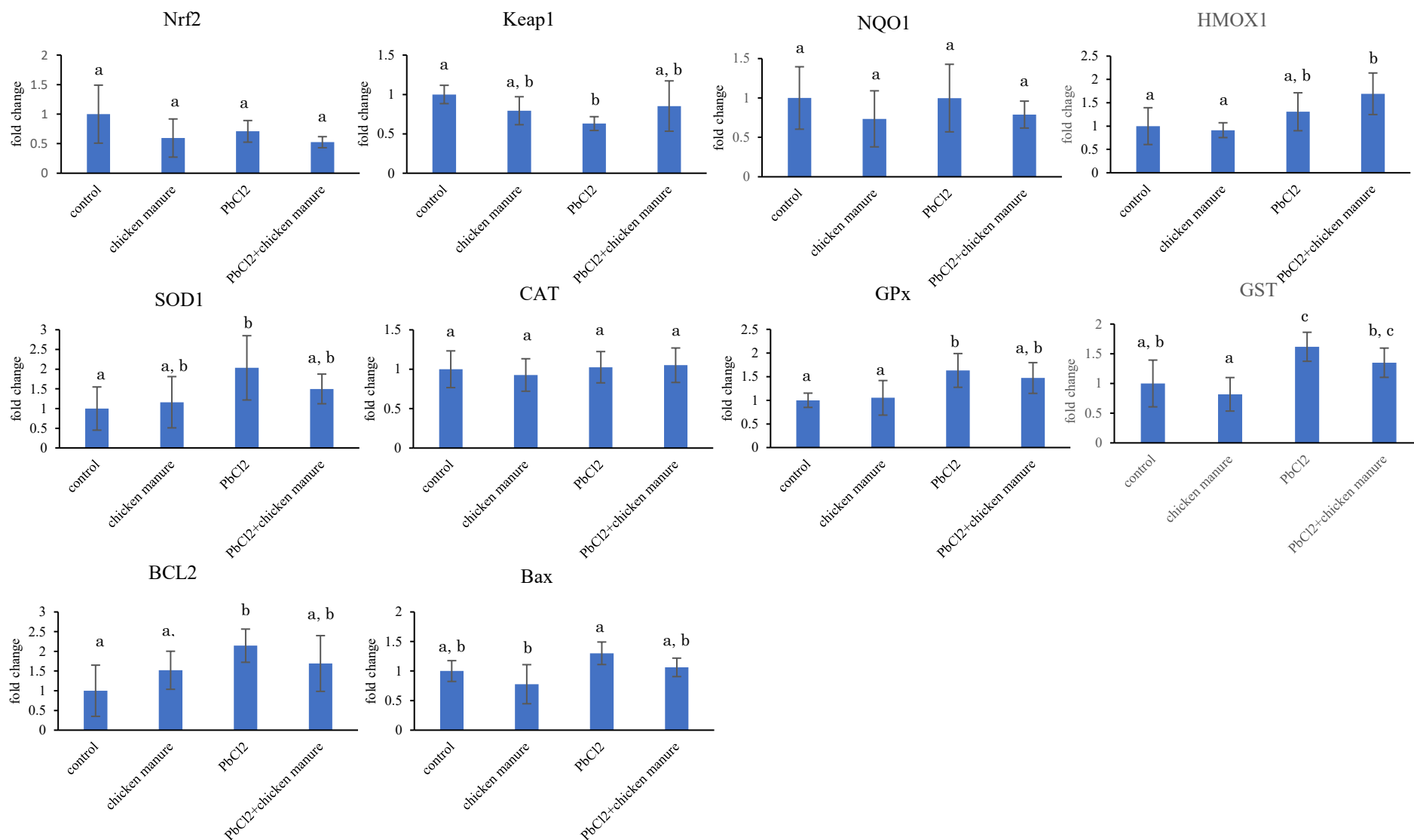
496 Figure 2. Expression of antioxidant enzymes and apoptosis related genes in the liver at 30 days exposure (n=6) at p<0.05. Different letter symbols 497 among groups denote significant difference.
