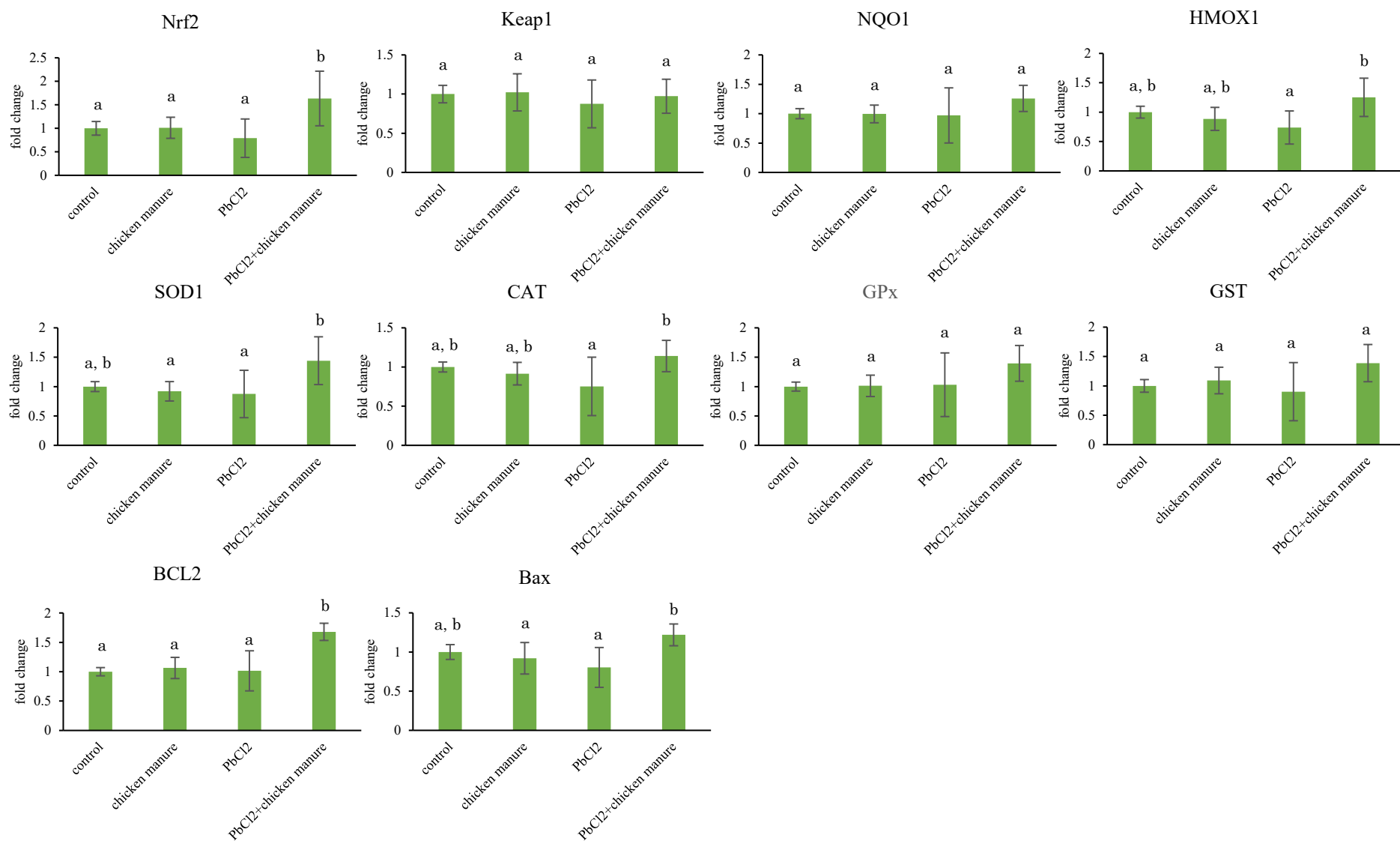
506 Figure 7. Expression of antioxidant enzymes and apoptosis related genes in the brain at 98 days exposure (n=6) at p<0.05. Different letter symbols 507 among groups denote significant difference.
