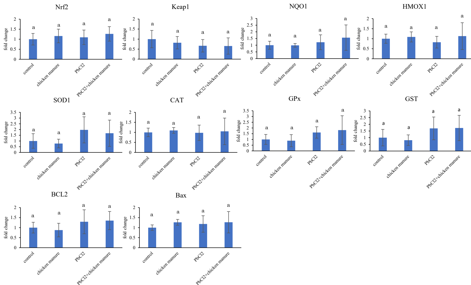
504 Figure 6. Expression of antioxidant enzymes and apoptosis related genes in the brain at 30 days exposure (n=6) at p<0.05. Different letter symbols 505 among groups denote significant difference.
