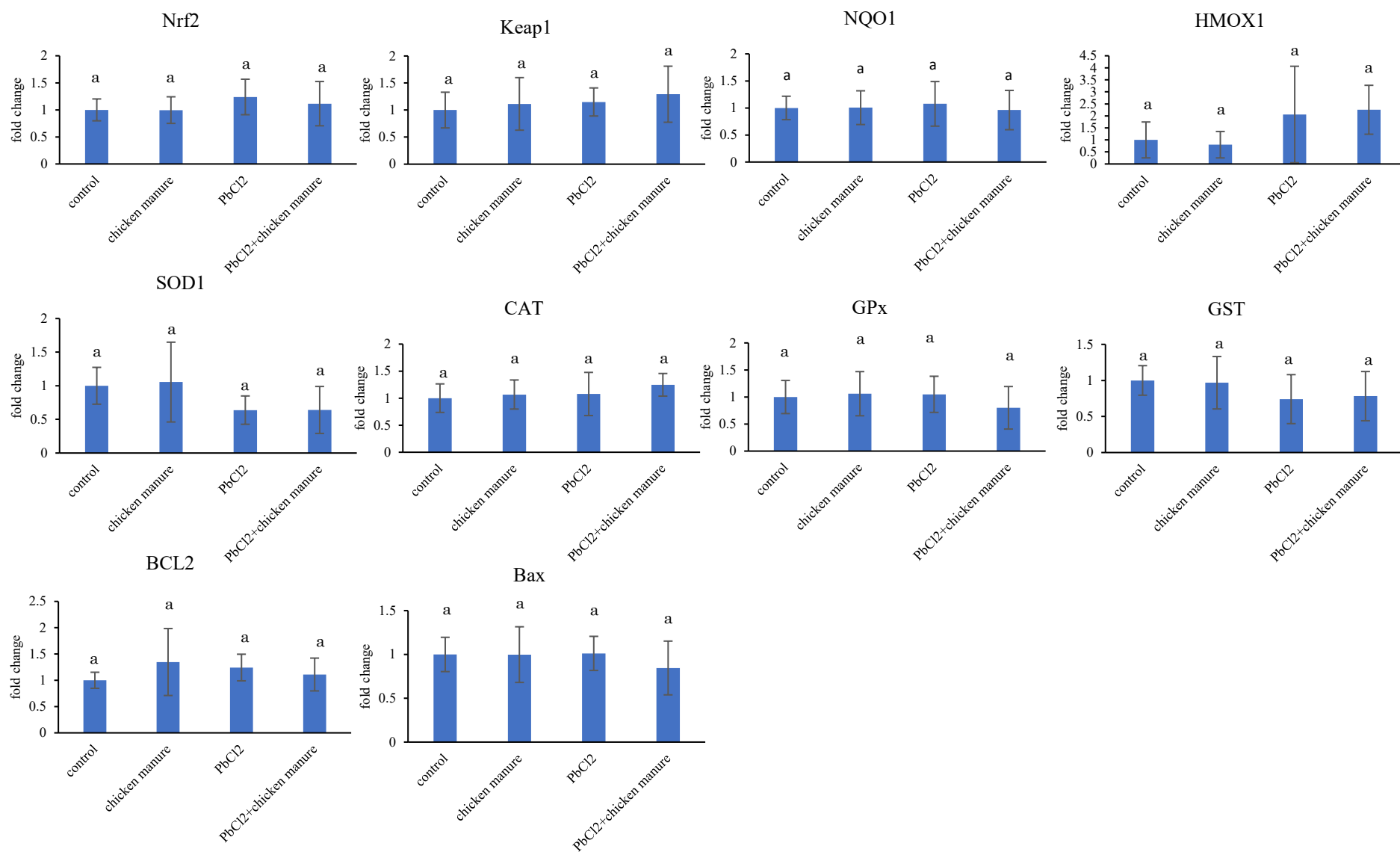
500 Figure 4. Expression of antioxidant enzymes and apoptosis related genes in the kidney at 30 days exposure (n=6) at p<0.05. Different letter symbols 501 among groups denote significant difference.
