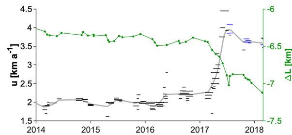
Figure 13. Surface ice speed and ice front position observed at Glacier O'Higgins between 2014 and 2018. Grey line indicates smoothed surface ice speed using a Gaussian smoothing routine with a time window of 90 days.
