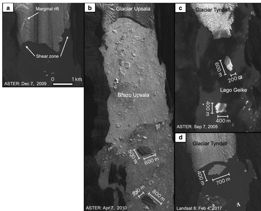
Figure 15. Tabular icebergs observed at (a) and (b) Glaciar Upsala, and (c) and (d) at Glaciar Tyndall. Note that the scale of the satellite images is different depending on the glacier.
