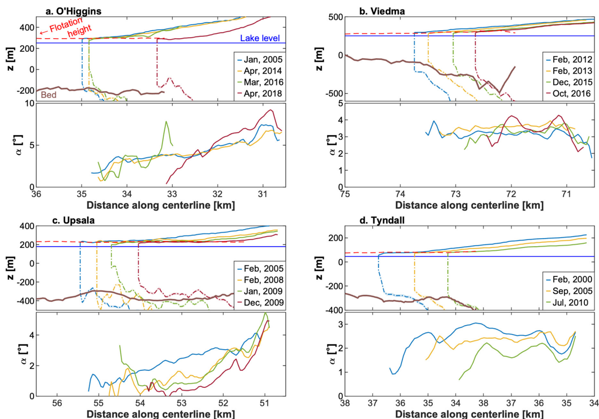
Figure 14. Longitudinal profiles of the ice surface elevations and slopes along the centreline at every 50 m in the horizontal interval for (a) Glaciar O'Higgins, (b) Glaciar Viedma, (c) Glaciar Upsala and (d) Glaciar Tyndall. The colour of the lines indicates the date. Red, blue and brown lines represent the flotation height, lake level and bed elevation, respectively. The dot-dashed line is the glacier base assuming hydrostatic equilibrium. The surface slope was calculated after applying the moving average on the surface elevation with a span of 2 km.
