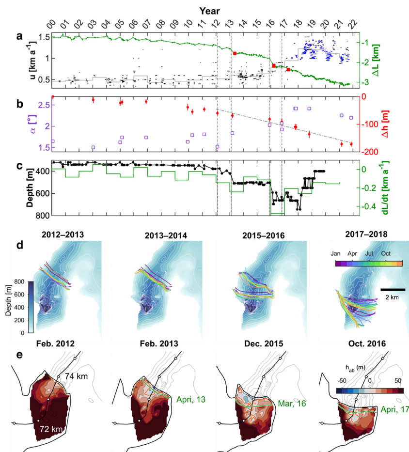
Figure 7. Similar plots as in Figure 6 for Glaciér Viedma. (d) Note that two years of ice-front positions are indicated.
