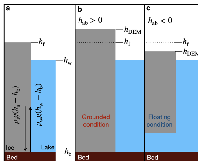
Figure 3. (a) Illustration of the overburden ice pressure and buoyancy force. (b) A higher ice surface elevation ( h_{DEM} ) than the flotation height ( h_f ) suggests a grounded condition, (c) while a lower h_{DEM} than h_f implies a floating condition. h_{ab} —height above buoyancy, h_w —water level, h_b —bed elevation, \rho_w —water density, \rho_i —ice density and g —gravitational acceleration.
