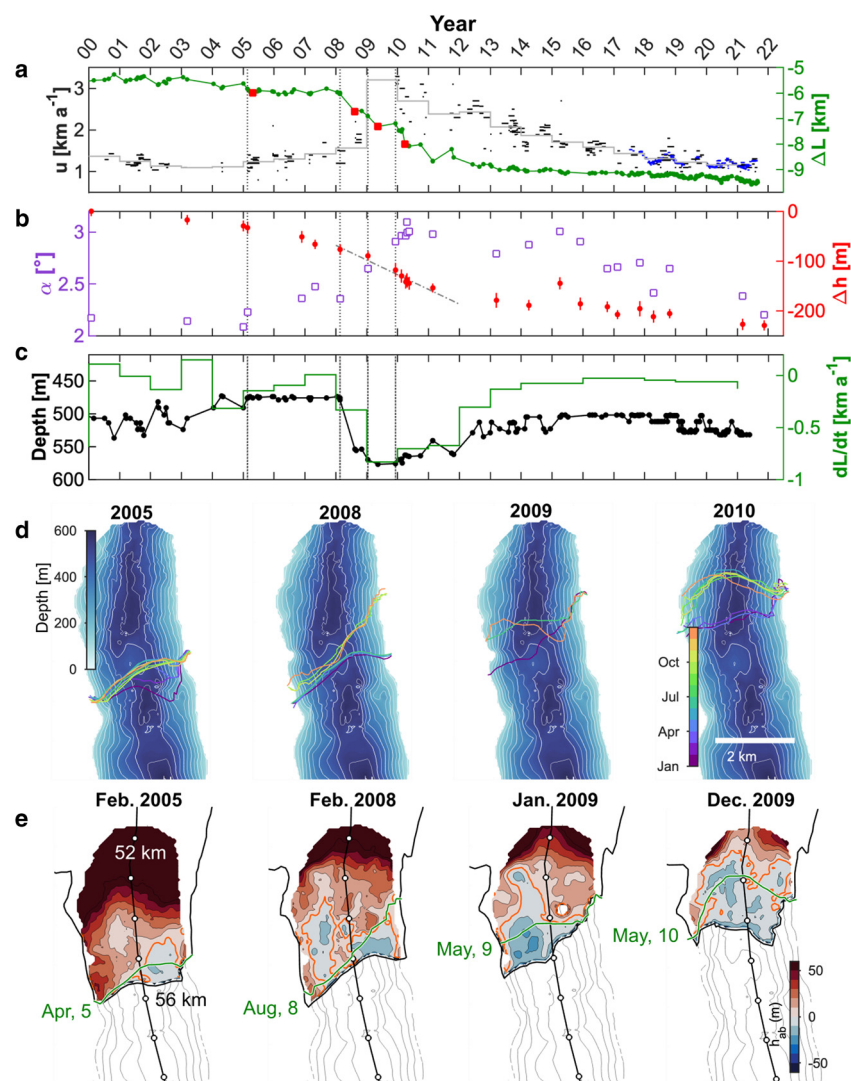
Figure 8. Similar plots as in Fig. 6 for Glacier Upsala. (e) Note that the bedrock bump was observed at 55 km along the centreline.
