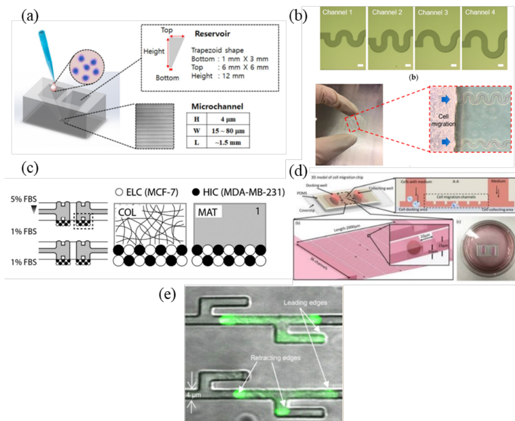
Fig. 3: Various microchannel designs. (a) Straight-shaped microchannel [29], (b) tortuous-shaped microchannel [16], (c) straight microchannel with microtracks [30], (d) microchannel with vertical micro-construction structures [35], and (e) branching microchannels [34]. Images reproduced with permission from references [16] [29] [30] [34] [35].
