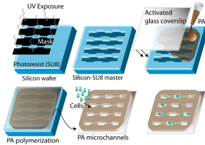
Fig. 5: Fabrication steps including fabrication of a silicon master, formation of a PA hydrogel, separation of the PA hydrogel from the master, and seeding of cells [42]. Images reproduced with permission from the reference [42].
