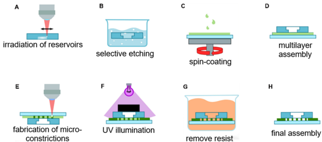
Fig. 6: Procedure for fabricating a multilayer device schematic using femtosecond laser micromachining (FLM) (modified from the reference [43]). (A) Irradiation of reservoirs inside the fused silica layer using fs-laser; (B) Selective etching of the irradiated structures in an HF solution; (C) Application of resist via spin-coating on the glass coverslip; (D) Assembly of the multilayer structure; (E) Fabrication of micro-constrictions using 2PP; (F) UV illumination; (G) Remove resist; (H) Final assembly.
