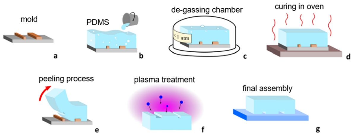
Fig. 4: Fabrication steps of PDMS-based microchannel (modified from the reference [41]). (a) A negative mold. (b) PDMS casting. (c) Deaeration. (d) PDMS cure. (e) Peeling off. (f) Plasma treatment. (g) A sealed PDMS device. Images reproduced with permission from the reference [41].
