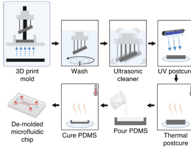
Fig. 7: Fabrication of microchannel using LCD 3D printing [18].
