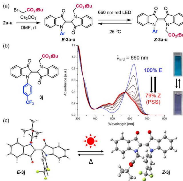
Figure 3. (a) Preparation of N -aryl- N' -alkylindigo photoswitches, (b) UV-vis spectrum and the color change in the photochromic study of indigo 3j (a 5.8 \times 10^{-5} M solution in toluene irradiated with 660 nm LED with spectra recorded every 30 s at 25 °C), (c) X-ray structures of indigo E - 3j and a DFT-computed structure of Z - 3j .
