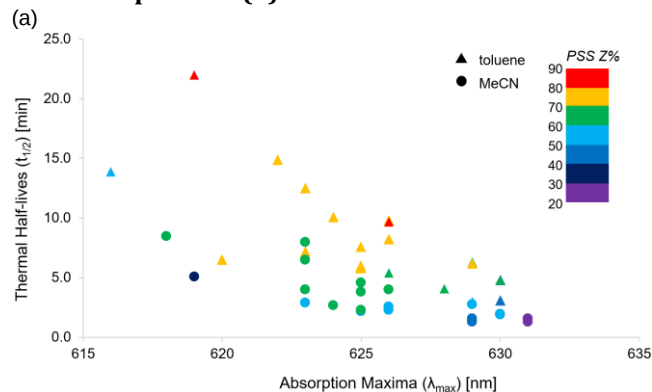
Scheme 4. Photochromic and thermal behavior of indigo photoswitches 3a–u in MeCN and toluene: (a) Overview plot and (b) tabulated data.
