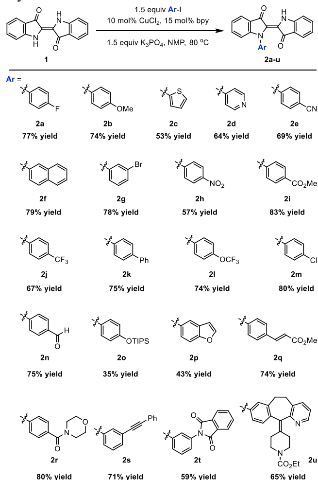
Scheme 1. Reaction scope of Cu-catalyzed indigo N -arylation a
