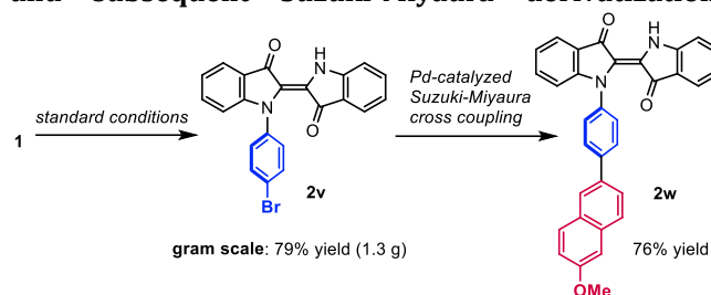
Scheme 2. Gram-scale reaction of indigo N -arylation and subsequent Suzuki-Miyaura derivatization
