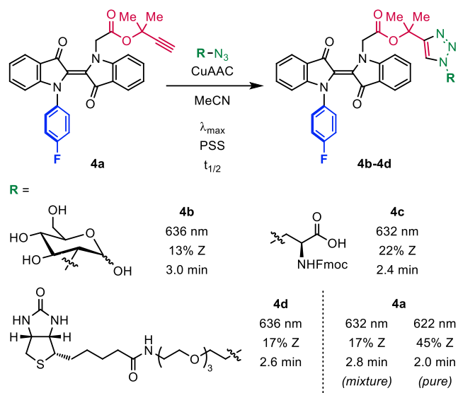
Scheme 5. Attachment of functional moieties through CuAAC and the photochromic properties of 4b–4d and 4a (pure and in reaction mixture) measured in MeCN.
