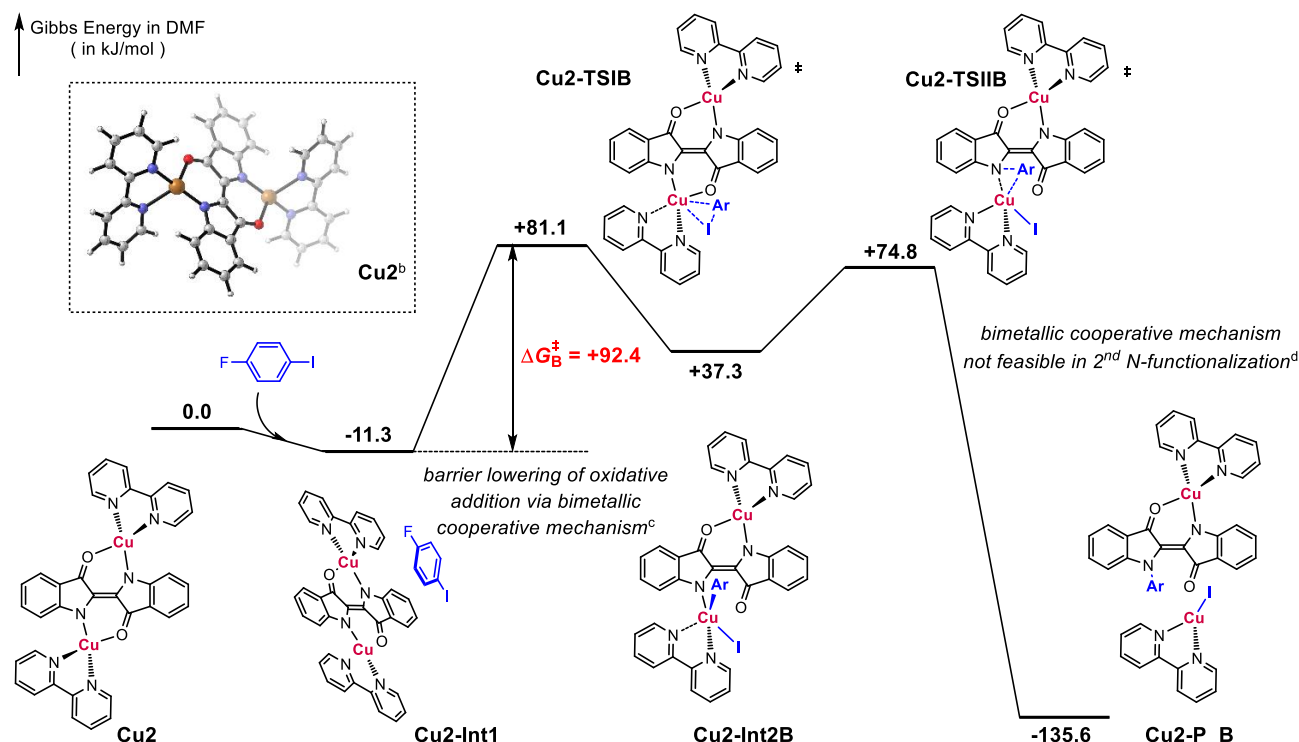
Scheme 3. Computed energy landscape of copper-catalyzed indigo N -arylation suggesting a minimum energy path via a bimetallic cooperative mechanism in the first N -arylation only a
