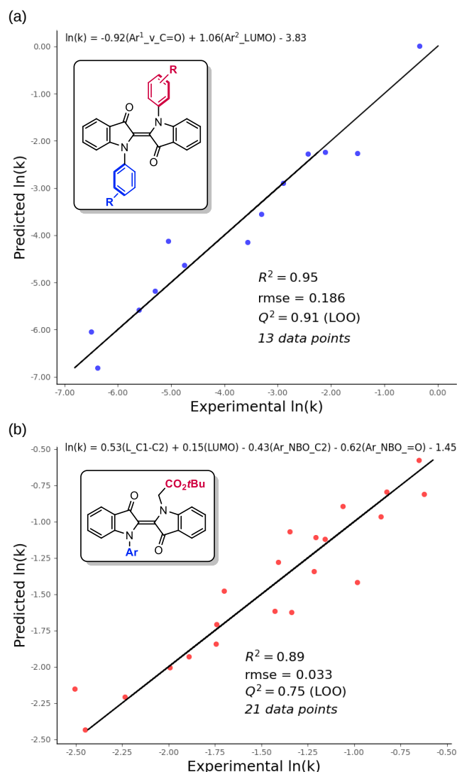
Figure 5. Multivariate regression models for thermal back-reaction rates ( k ) of (a) N,N' -diarylindigos ( R = p\text{-OMe}, H, p\text{-F}, p\text{-CF}_3, p\text{-CN}, p\text{-NO}_2, m\text{-OMe}, m\text{-CHO}, m\text{-CF}_3, m\text{-CN}, m\text{-NO}_2 ) and (b) N -aryl- N' -alkylindigos ( 3a-3u ). See SI for more information.
