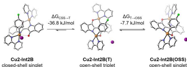
Figure 2. Electronic coupling of two Cu centers observed for Cu2-Int2B
