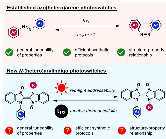
Figure 1. Development of new N -arylindigos as red-light photoswitches.
