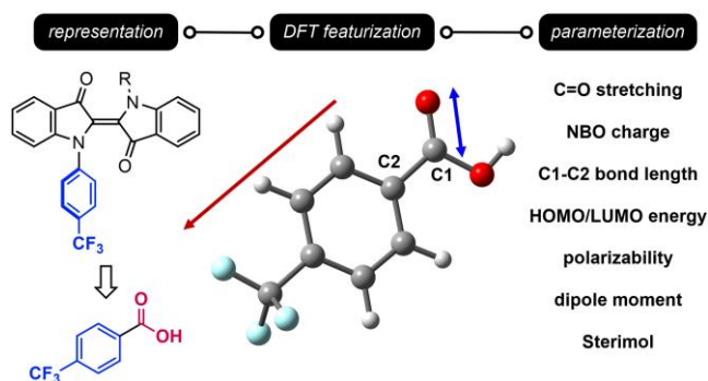
Figure 4. Workflow for correlating the N -aryl structures and rate of thermal back-reaction.
