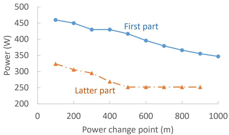
544 Fig. 4 Best combination of power levels for the windless and flat 1 km course.
