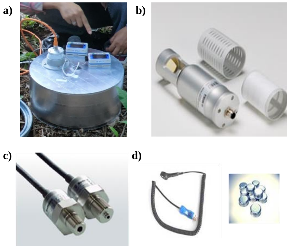
Fig. 3. Instruments for CO 2 emission and environmental factor measurement, (a) closed chamber system, (b) portable infrared CO 2 analyzer, (c) GWL sensor, and (d) soil temperature sensor.
