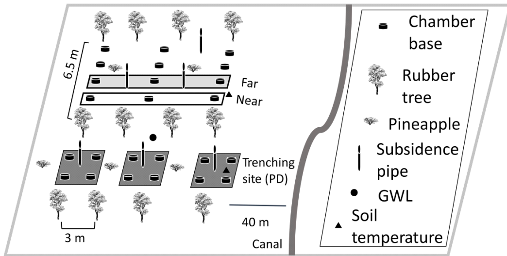
Fig. 1. Experimental plots and the distribution of chamber bases and ground sensors in Central Kalimantan.
