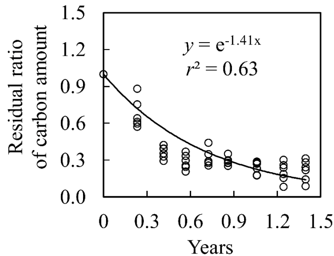
Fig. 19. C loss pattern of pruned fronds.
