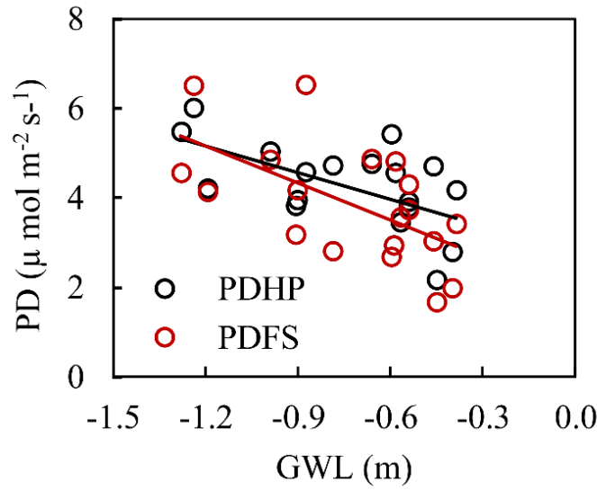
Fig. 16. Relationship between peat decomposition (PD) and groundwater level (GWL) on different management area: peat decomposition in the harvesting path (PDHP, black circle) and peat decomposition in the frond stack (PDFS, red circle). Each symbol denotes an average of 3 plots ( n = 3 ). A line is fitted for each management area ( p < 0.01 ). PDHP: y = -1.99x + 2.77 ( r^2 = 0.34 ), and PDFS: y = -2.78x + 1.84 ( r^2 = 0.36 ).
