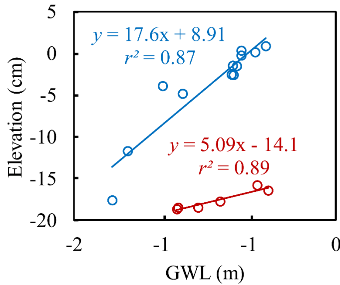
Fig. 18. Relationship between peat elevation and groundwater level (GWL) from October 2018 to September 2019 (blue circle), and October 2019 to March 2020 (red circle). A line was fitted for each period.
