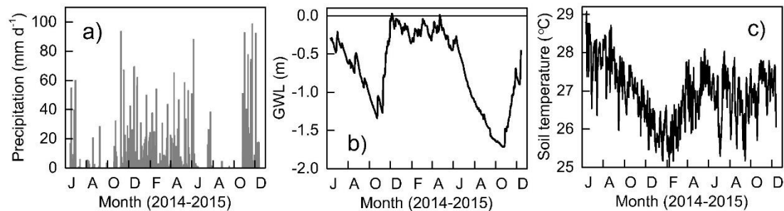
Fig. 4. Variations in daily values of (a) precipitation, (b) groundwater level (GWL) and (c) soil temperature inside (black) and outside (grey) the trenching from June 2014 to December 2015. Precipitation was measured in Palangkaraya (Hirano et al., 2009), which was about 25 km distant from the study site.
