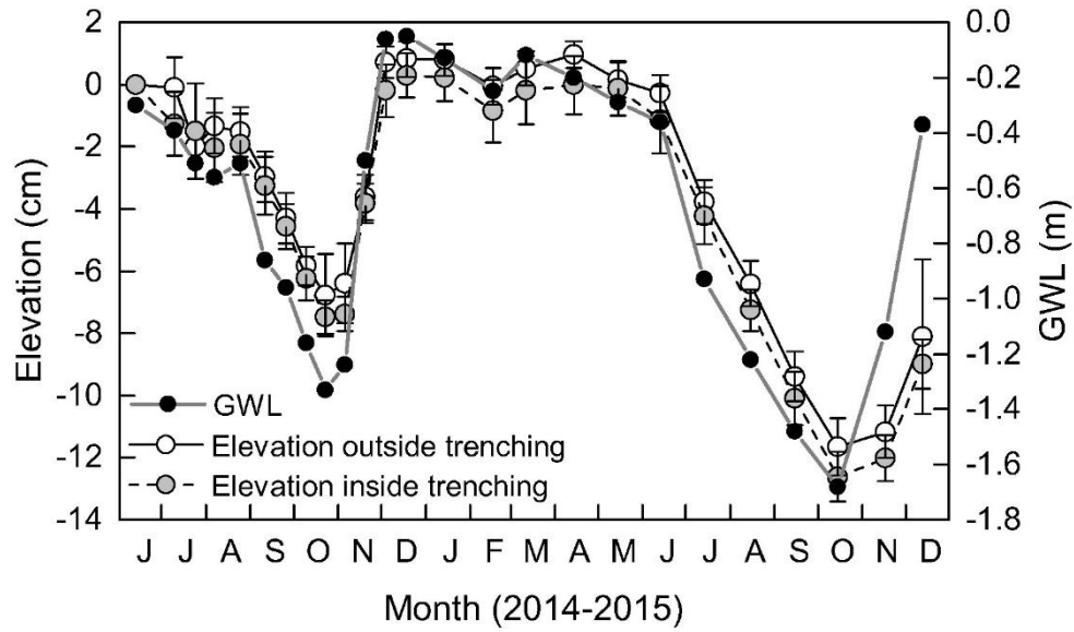
Fig. 9. Seasonal variations in peat surface elevation and groundwater level (GWL) from June 2014 through December 2015. Mean elevation ( n = 3 ) is shown relatively to that in June 2014. Vertical bars denote 1 standard deviation.
