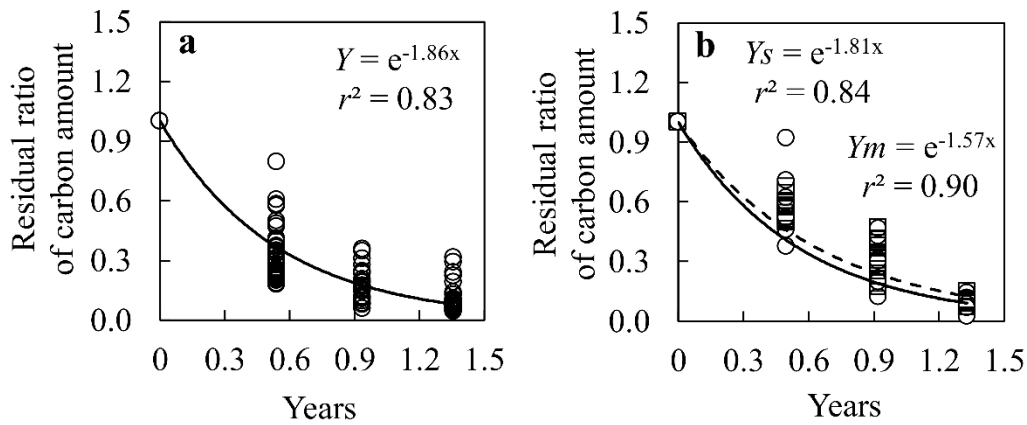
Fig. 12. C loss pattern of a) M in Riau and b) M (squares, dash line) and S (circles, solid line) in Jambi. y_m and y_s represent the fitted equations for M and S in Jambi, respectively.
