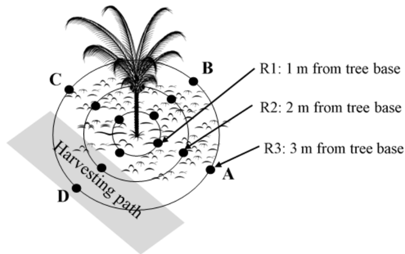
Fig. 10. Scheme of sequential soil core sampling at different distances and areas from oil palm tree base.
