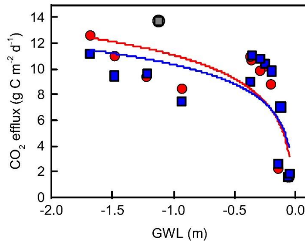
Fig. 8. Relationship between total soil respiration (SR) and groundwater level (GWL) for near (circles) and far (squares) positions from tree rows. Each symbol denotes a daily average ( n = 6 ). A grey symbol denotes November's measurement. A logarithmic curve is fitted without the grey symbol for each position ( p < 0.01 ): near) y = 11.1 - 2.63 \ln(-x) ( r^2 = 0.61 ), far) y = 10.4 - 2.17 \ln(-x) ( r^2 = 0.47 ).
