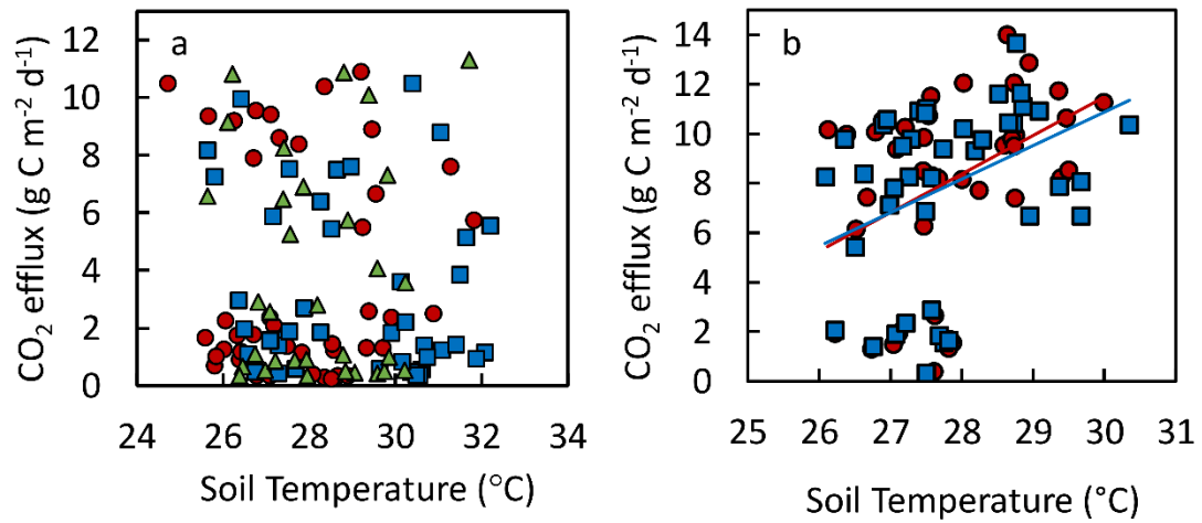
Fig. 6. Relationship between (a) peat decomposition (PD) and soil temperature in trenching 1 (circles), 2 (squares) and 3 (triangles), (b) total soil respiration (SR) and soil temperature for near (circles) and far (squares) positions from tree rows. Each symbol denotes one chamber base. A line is fitted for SR ( p < 0.05 ) at near ( y = 1.56x - 35.2 ; r^2 = 0.15 ) and far ( y = 1.35x - 29.8 ; r^2 = 0.14 ) positions from rubber tree.
