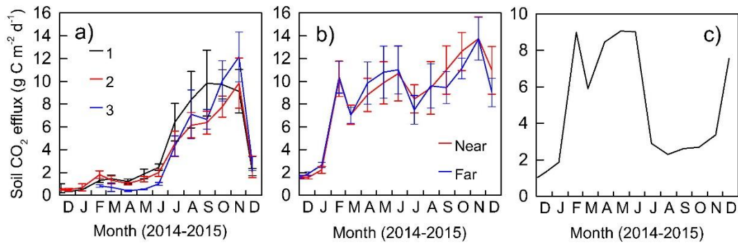
Fig. 5. Seasonal variations in daily mean (a) peat decomposition (PD, three trenching plots, n = 4 ), (b) total soil respiration (SR, near and far positions from tree rows, n = 6 ) and (c) residual between means of SR and PD from December 2014 to December 2015. Vertical bars in (a) and (b) denote 1 standard error (SE).
