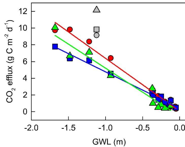
Fig. 7. Relationship between peat decomposition (PD) and groundwater level (GWL) in trenching 1 (circles), 2 (squares) and 3 (triangles). Each symbol denotes a daily average ( n = 4 ). A grey symbol denotes November's measurement. A line is fitted without the grey symbol for each trenching ( p < 0.001 ): 1) y = 0.07 - 6.3x ( r^2 = 0.98 ), 2) y = 0.41 - 4.35x ( r^2 = 0.98 ), 3) y = -0.53 - 5.74x ( r^2 = 0.94 ).
