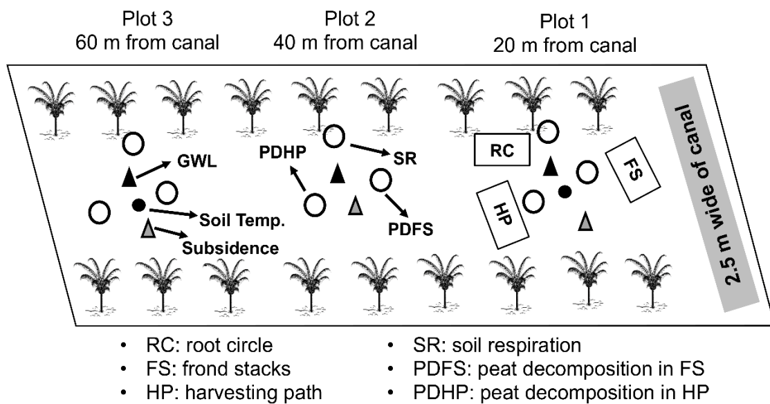
Fig. 13. Experimental plots and the distribution of chamber bases and ground sensors in South Kalimantan.
