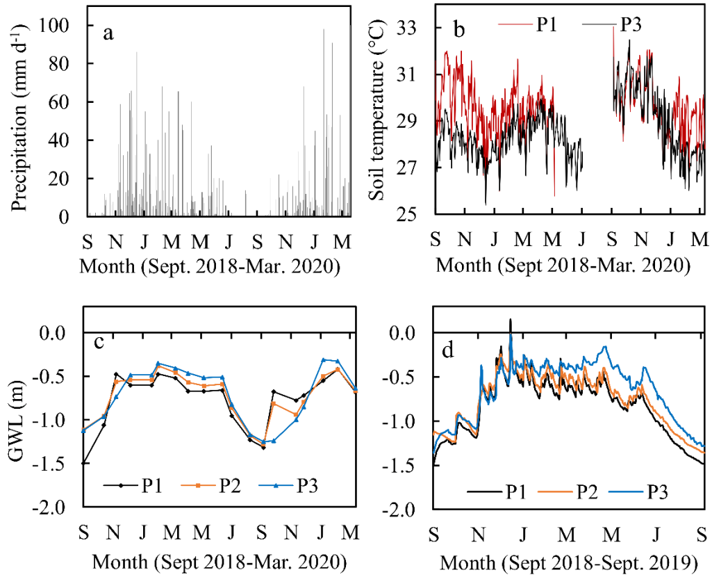
Fig. 14. Variations in daily values of (a) precipitation, (b) soil temperature in plot 1 and 3, (c) groundwater level (GWL) in 3 plots from monthly manual measurement from September 2018 to March 2020, and (d) GWL from automatic measurement in 3 plots from September 2018 to September 2019 (data after September 2019 were missing because of the sensors problem). Precipitation was measured about 5 km distant from the study site (BMKG, South Kalimantan).
