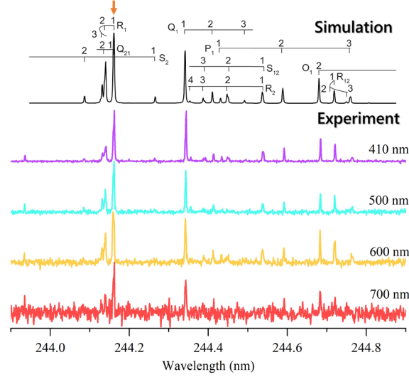
Fig. 2. Experimental (2+1) REMPI spectra of the OH radicals desorbed from ASW by a 410–700 nm PSD laser compared with the simulated spectrum of the D^2\Sigma^- (\nu' = 0) \leftarrow X^2\Pi (\nu'' = 0) transition at a rotational temperature of 140 K. An arrow on the top spectrum shows the REMPI wavelength 244.162 nm for monitoring the OH intensity.
